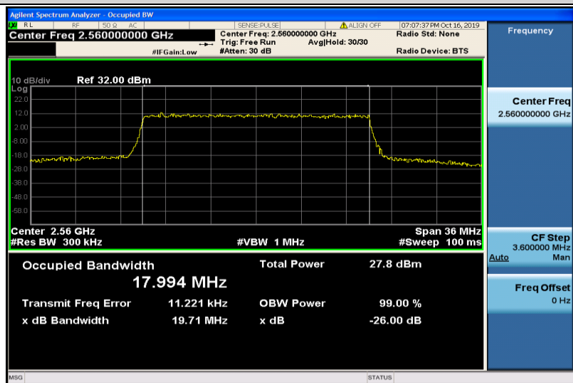
Band7-20MHz-16QAM-21350-100RB#0-17.994
