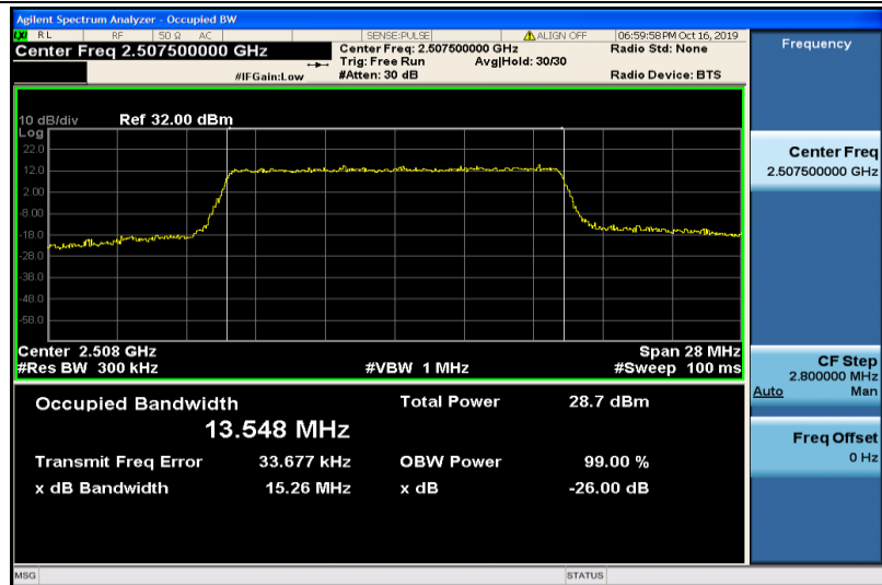
Band7-15MHz-QPSK-20825-75RB#0-13.548
