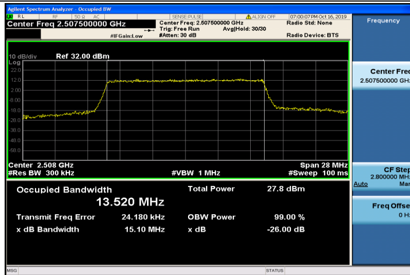
Band7-15MHz-16QAM-20825-75RB#0-13.520
