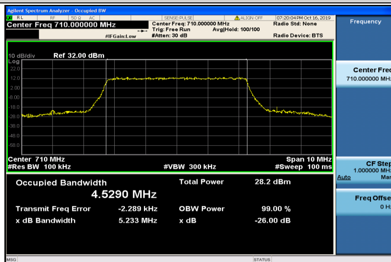
Band17-5MHz-16QAM-23790-25RB#0-4.5290
