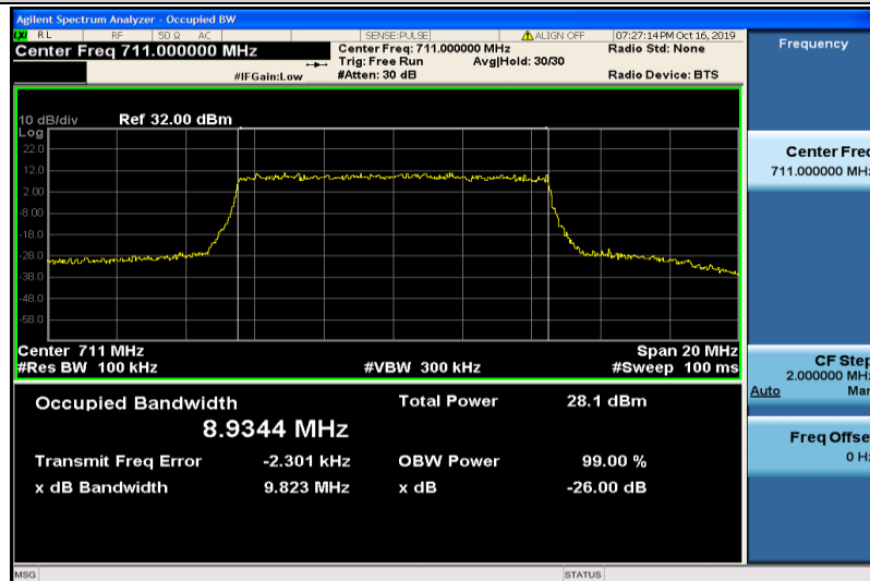
Band17-10MHz-16QAM-23800-50RB#0-8.9344
