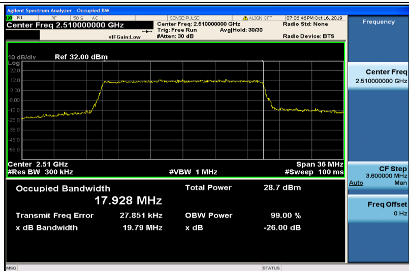
Band7-20MHz-QPSK-20850-100RB#0-17.928
