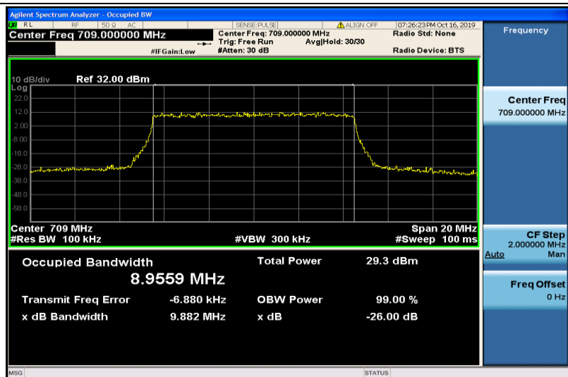
Band17-10MHz-QPSK-23780-50RB#0-8.9559
