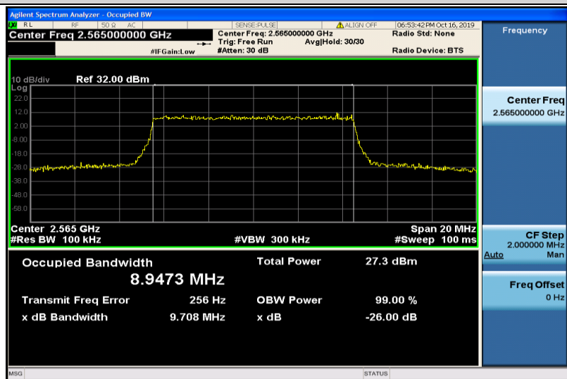
Band7-10MHz-16QAM-21400-50RB#0-8.9473
