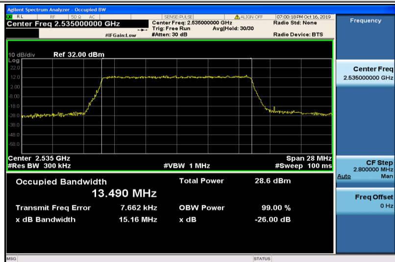
Band7-15MHz-QPSK-21100-75RB#0-13.490
