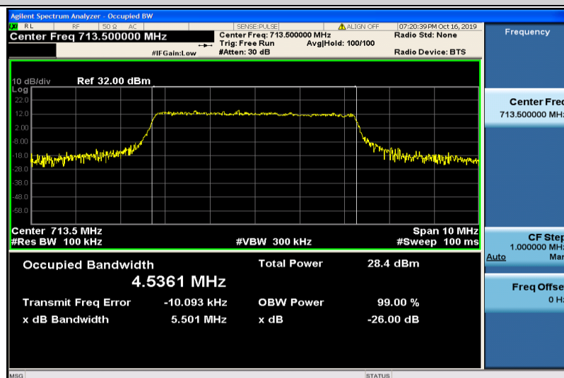
Band17-5MHz-16QAM-23825-25RB#0-4.5361
