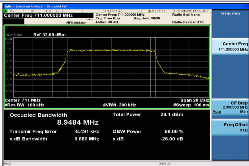
Band17-10MHz-QPSK-23800-50RB#0-8.9484
