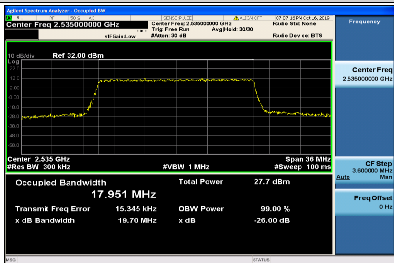
Band7-20MHz-16QAM-21100-100RB#0-17.951
