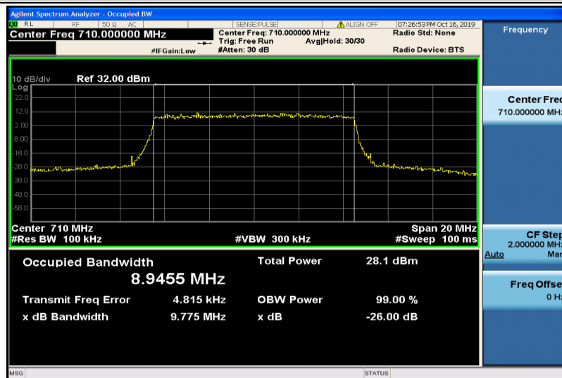
Band17-10MHz-16QAM-23790-50RB#0-8.9455
