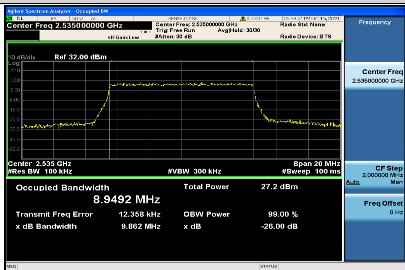
Band7-10MHz-16QAM-21100-50RB#0-8.9492
