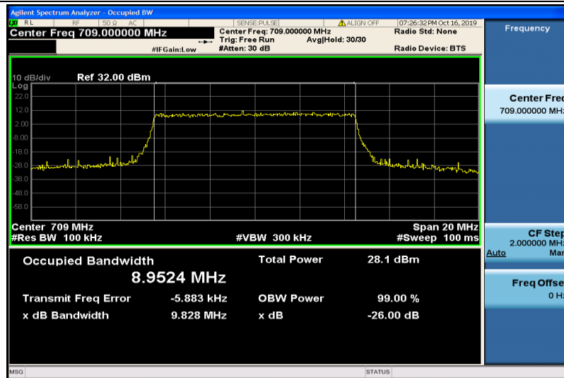
Band17-10MHz-16QAM-23780-50RB#0-8.9524
