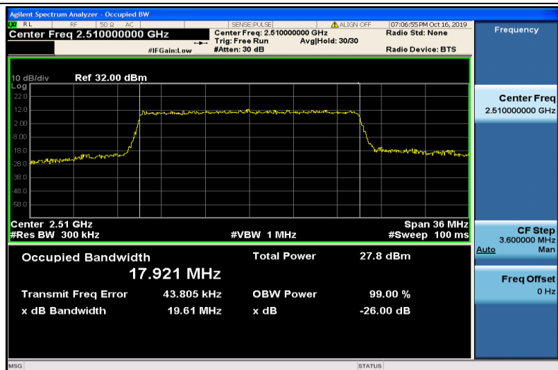
Band7-20MHz-16QAM-20850-100RB#0-17.921
