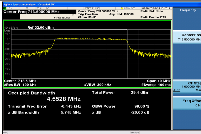
Band17-5MHz-QPSK-23825-25RB#0-4.5528
