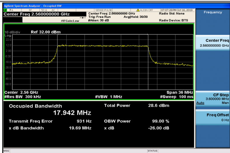
Band7-20MHz-QPSK-21350-100RB#0-17.942
