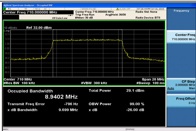
Band17-10MHz-QPSK-23790-50RB#0-8.9402
