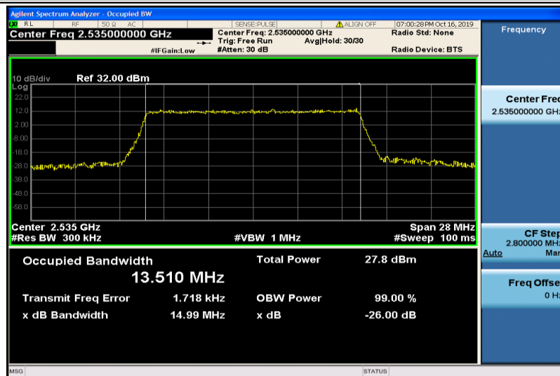
Band7-15MHz-16QAM-21100-75RB#0-13.510
