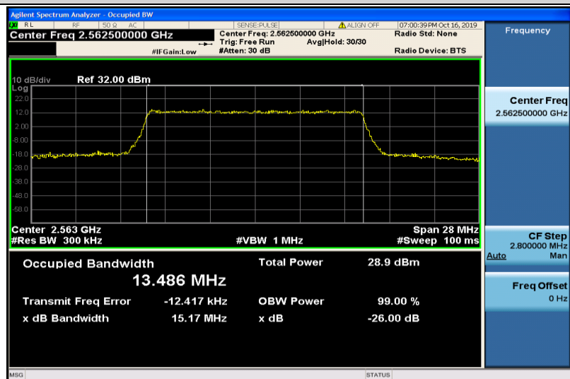
Band7-15MHz-QPSK-21375-75RB#0-13.486
