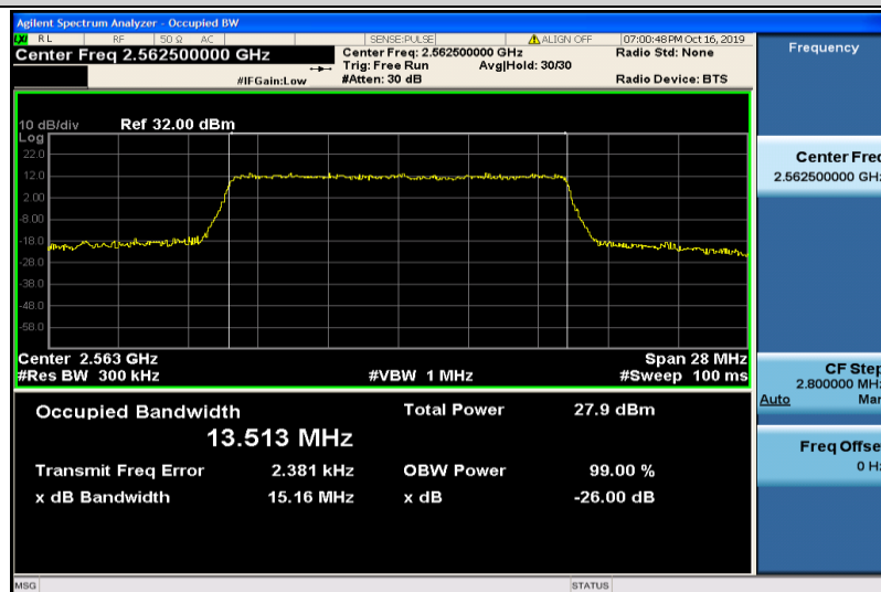
Band7-15MHz-16QAM-21375-75RB#0-13.513
