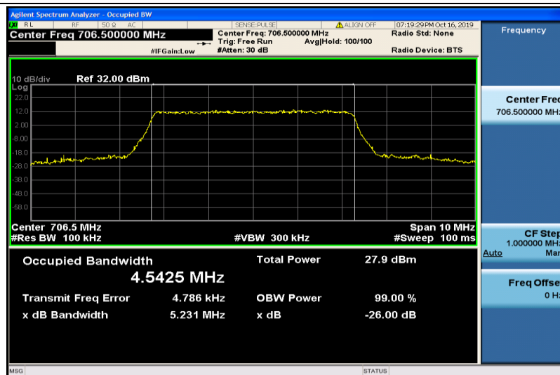
Band17-5MHz-16QAM-23755-25RB#0-4.5425
