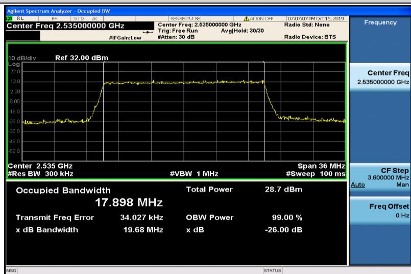
Band7-20MHz-QPSK-21100-100RB#0-17.898
