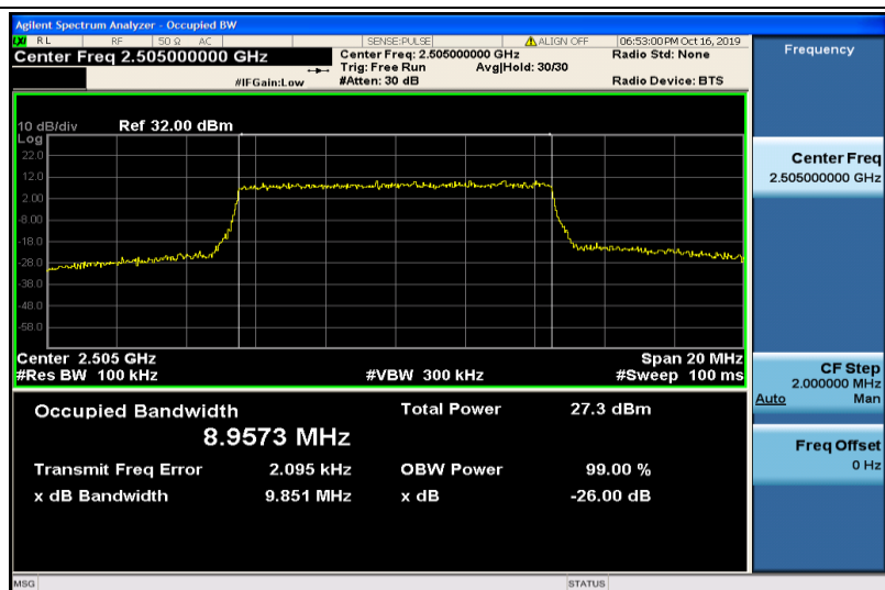
Band7-10MHz-16QAM-20800-50RB#0-8.9573
