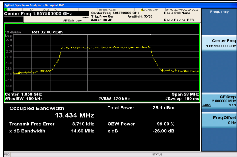
Band2-15MHz-16QAM-18675-75RB#0-13.434
