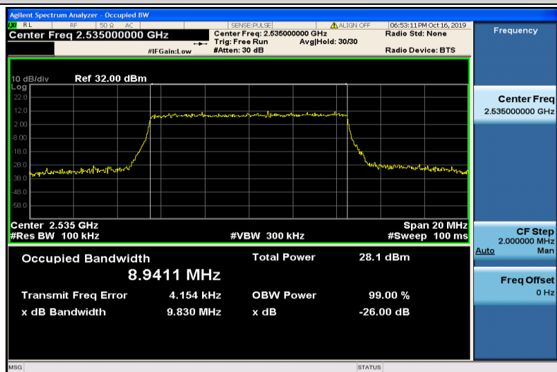
Band7-10MHz-QPSK-21100-50RB#0-8.9411
