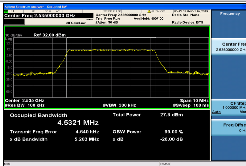
Band7-5MHz-16QAM-21100-25RB#0-4.5321
