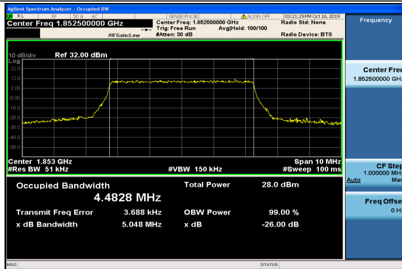
Band2-5MHz-16QAM-18625-25RB#0-4.4828
