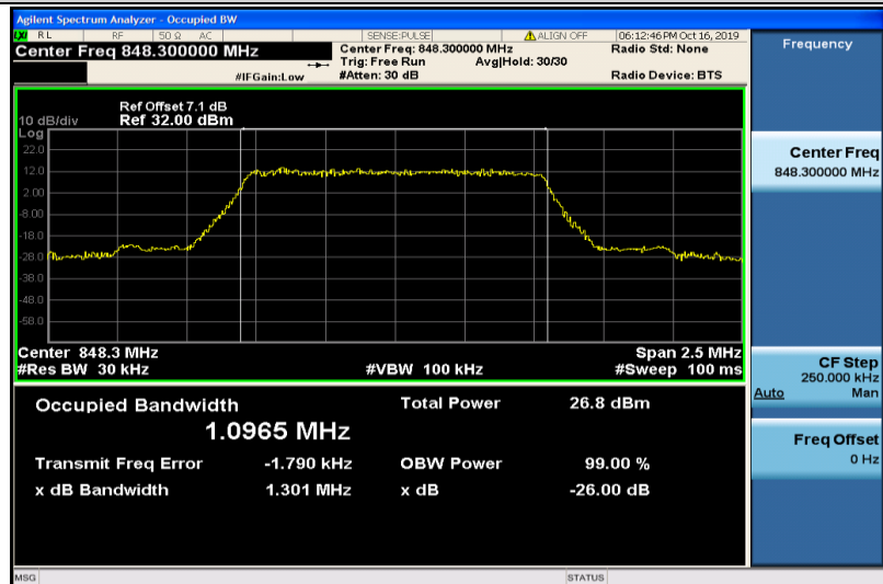
Band5-1.4MHz-16QAM-20643-6RB#0-1.0965
