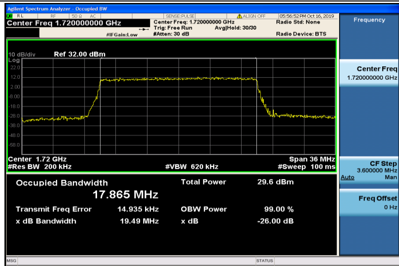
Band4-20MHz-QPSK-20050-100RB#0-17.865
