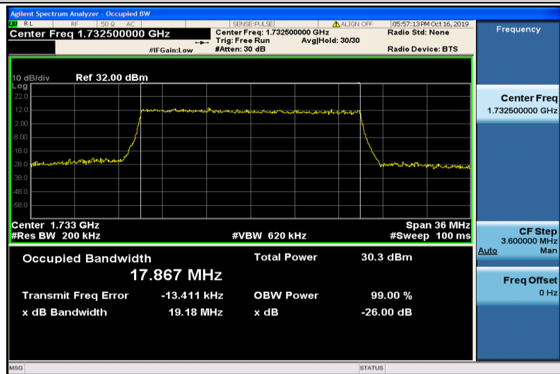
Band4-20MHz-QPSK-20175-100RB#0-17.867
