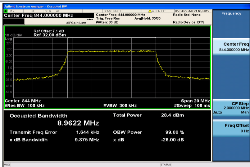
Band5-10MHz-QPSK-20600-50RB#0-8.9622
