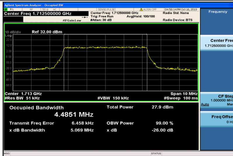
Band4-5MHz-16QAM-19975-25RB#0-4.4851
