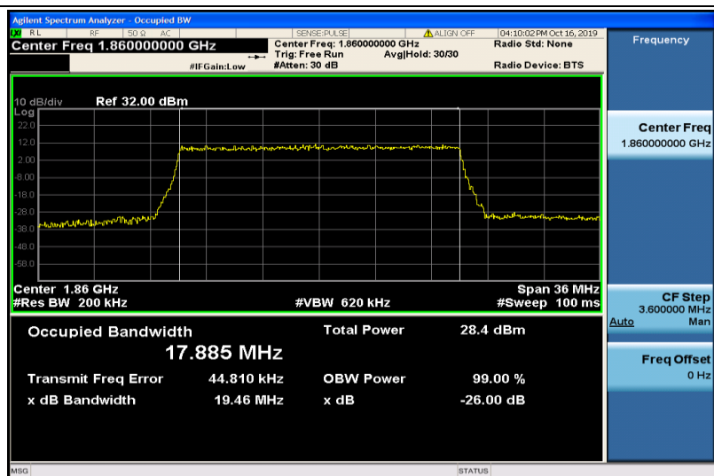
Band2-20MHz-16QAM-18700-100RB#0-17.885
