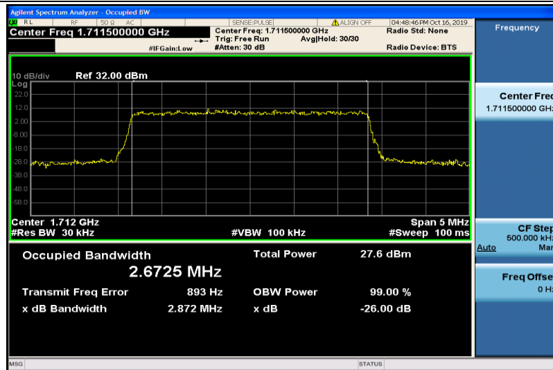
Band4-3MHz-16QAM-19965-15RB#0-2.6725
