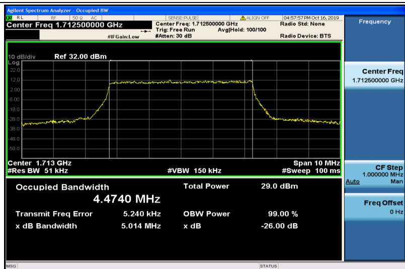
Band4-5MHz-QPSK-19975-25RB#0-4.4740
