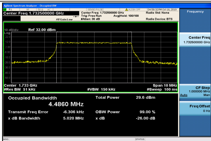
Band4-5MHz-QPSK-20175-25RB#0-4.4860
