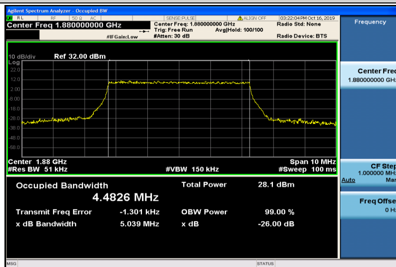
Band2-5MHz-16QAM-18900-25RB#0-4.4826
