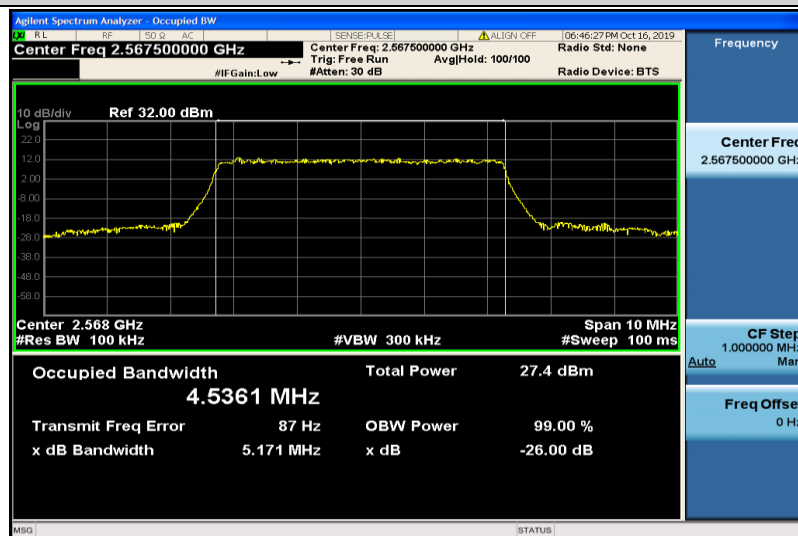
Band7-5MHz-16QAM-21425-25RB#0-4.5361
