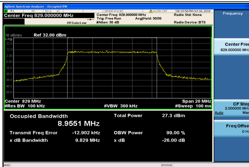
Band5-10MHz-16QAM-20450-50RB#0-8.9551
