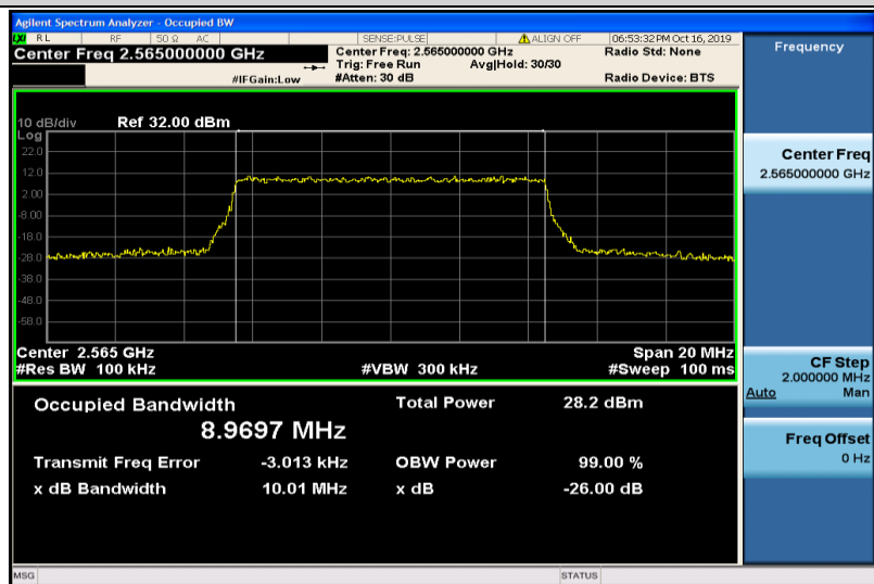
Band7-10MHz-QPSK-21400-50RB#0-8.9697
