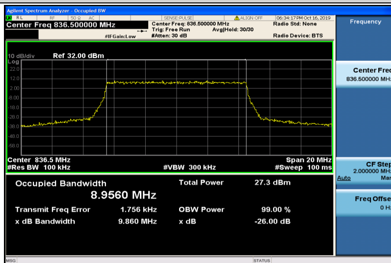
Band5-10MHz-16QAM-20525-50RB#0-8.9560
