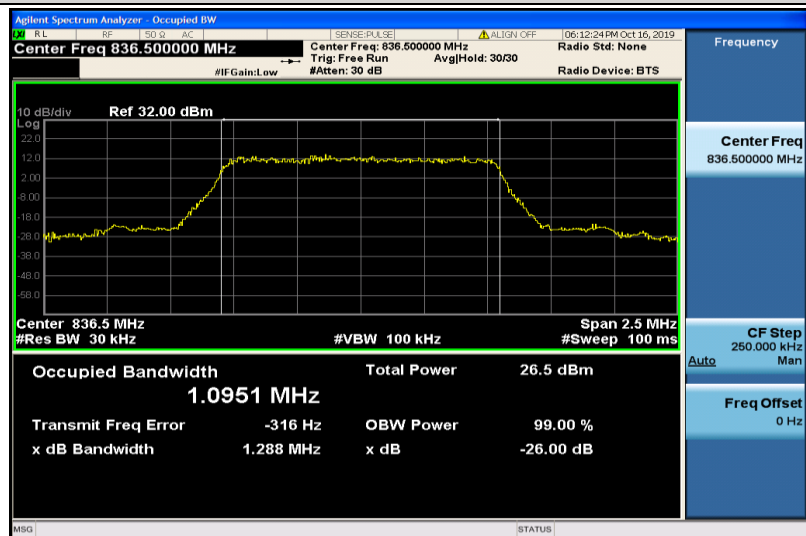
Band5-1.4MHz-16QAM-20525-6RB#0-1.0951
