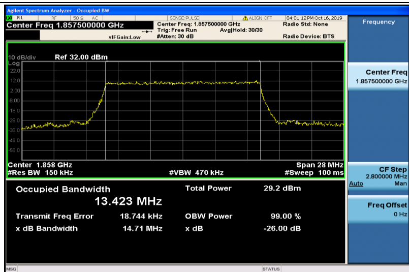
Band2-15MHz-QPSK-18675-75RB#0-13.423
