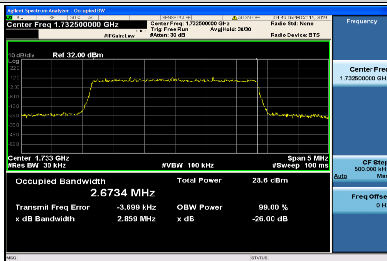
Band4-3MHz-16QAM-20175-15RB#0-2.6734
