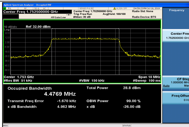
Band4-5MHz-16QAM-20375-25RB#0-4.4769
