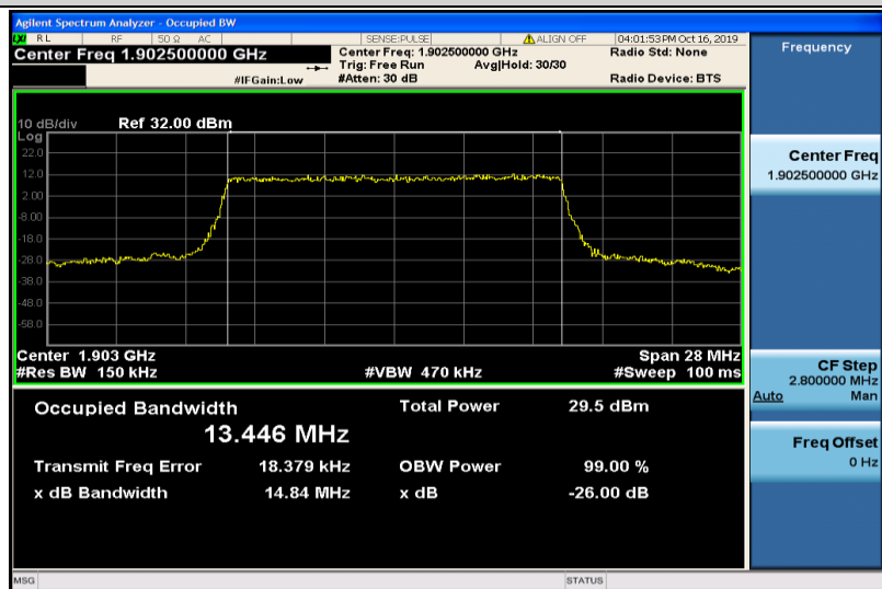
Band2-15MHz-QPSK-19125-75RB#0-13.446
