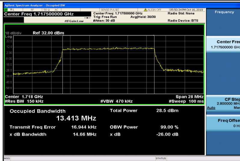
Band4-15MHz-16QAM-20025-75RB#0-13.413
