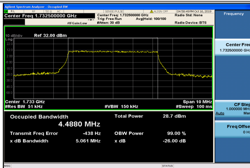
Band4-5MHz-16QAM-20175-25RB#0-4.4880
