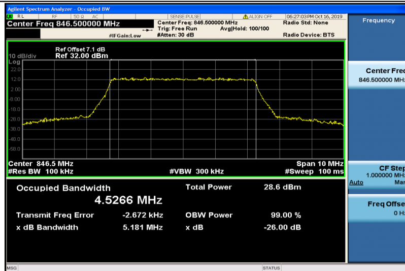
Band5-5MHz-QPSK-20625-25RB#0-4.5266
