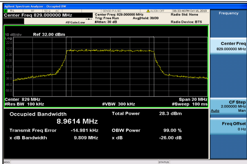
Band5-10MHz-QPSK-20450-50RB#0-8.9614
