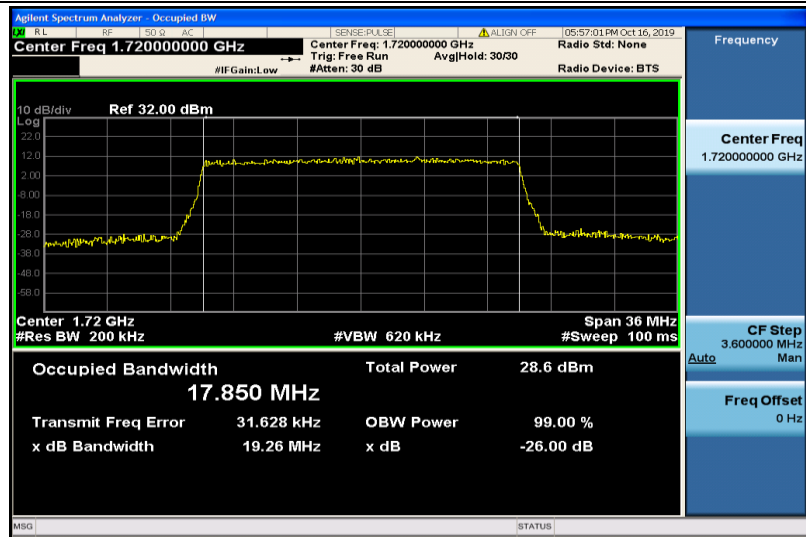
Band4-20MHz-16QAM-20050-100RB#0-17.850
