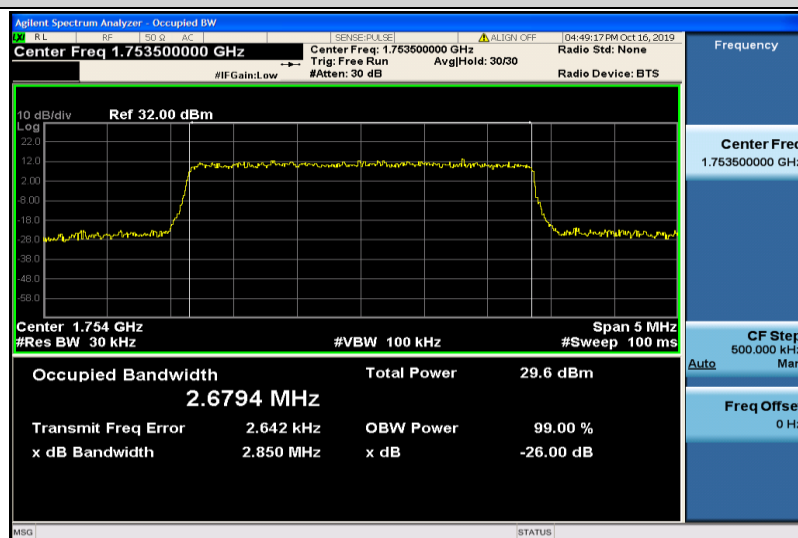
Band4-3MHz-QPSK-20385-15RB#0-2.6794
