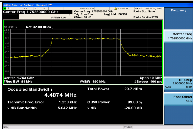
Band4-5MHz-QPSK-20375-25RB#0-4.4874
