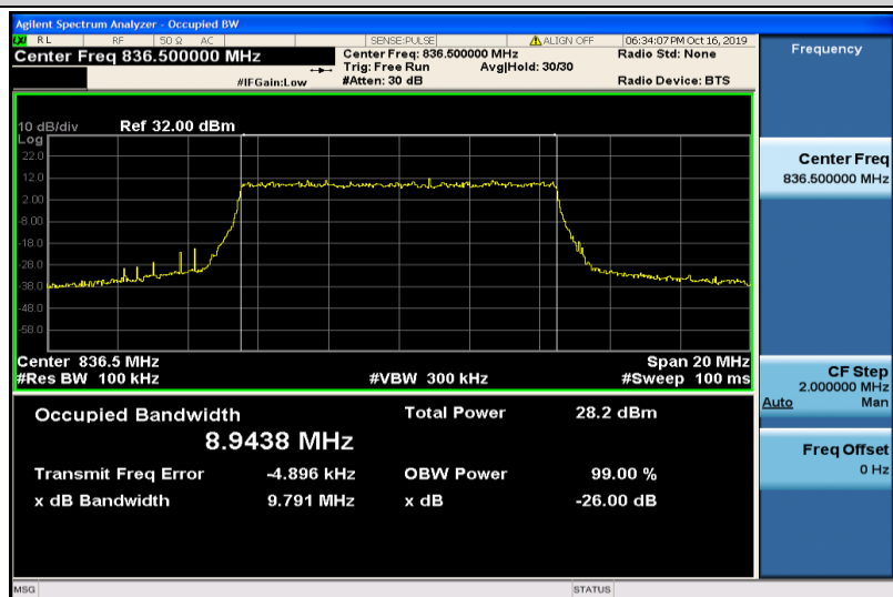
Band5-10MHz-QPSK-20525-50RB#0-8.9438
