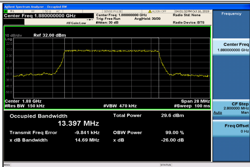
Band2-15MHz-QPSK-18900-75RB#0-13.397
