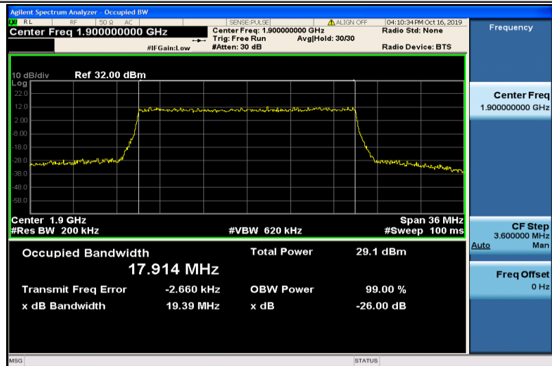
Band2-20MHz-QPSK-19100-100RB#0-17.914
