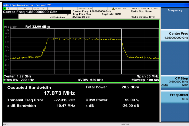
Band2-20MHz-16QAM-18900-100RB#0-17.873
