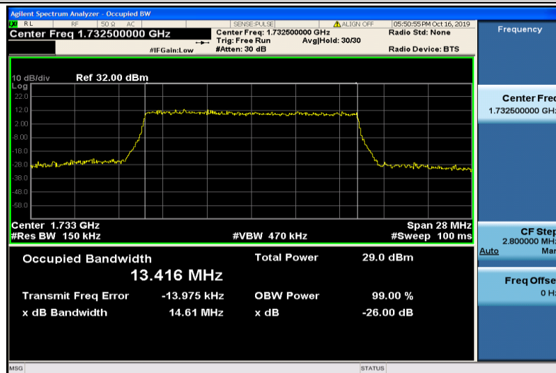
Band4-15MHz-16QAM-20175-75RB#0-13.416
