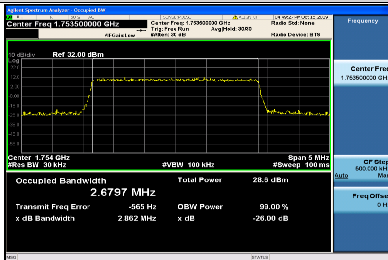
Band4-3MHz-16QAM-20385-15RB#0-2.6797
