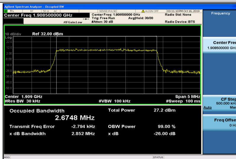
Band2-3MHz-16QAM-19185-15RB#0-2.6748
