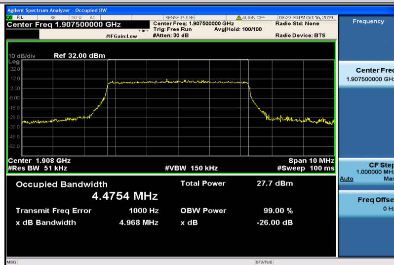
Band2-5MHz-16QAM-19175-25RB#0-4.4754
