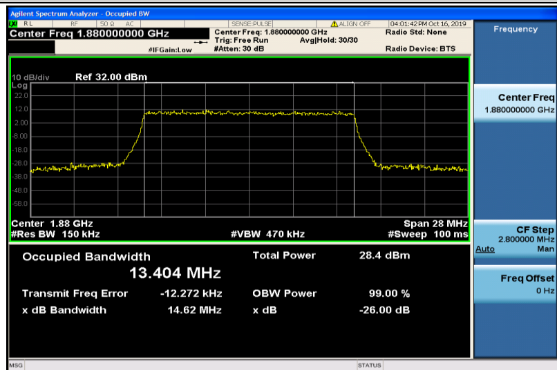
Band2-15MHz-16QAM-18900-75RB#0-13.404
