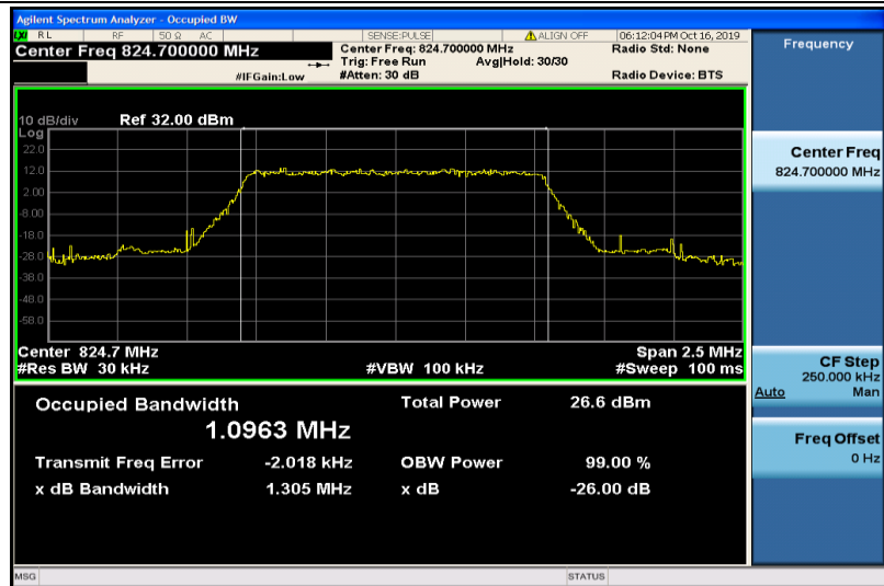
Band5-1.4MHz-16QAM-20407-6RB#0-1.0963
