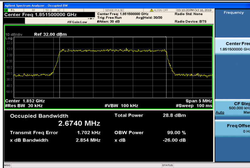
Band2-3MHz-QPSK-18615-15RB#0-2.6740
