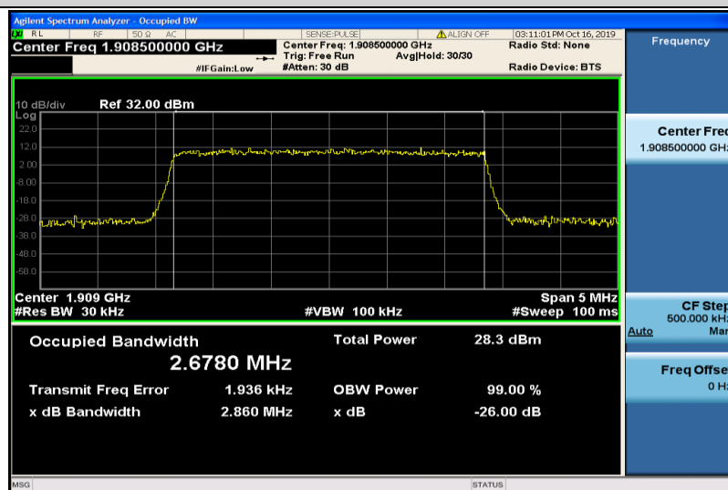
Band2-3MHz-QPSK-19185-15RB#0-2.6780
