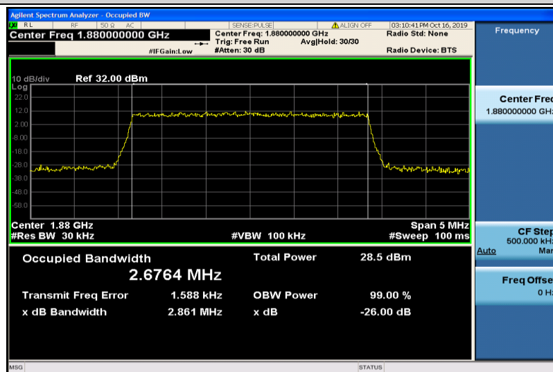
Band2-3MHz-QPSK-18900-15RB#0-2.6764
