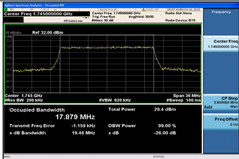
Band4-20MHz-16QAM-20300-100RB#0-17.879
