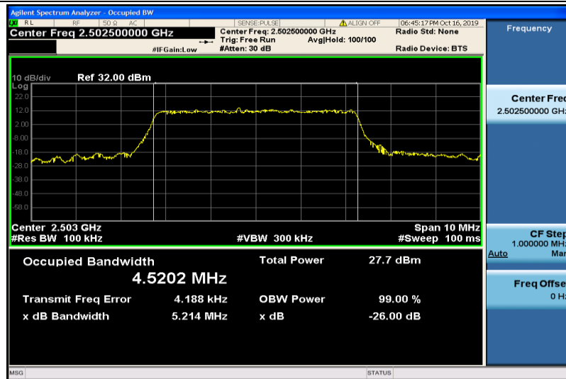
Band7-5MHz-16QAM-20775-25RB#0-4.5202
