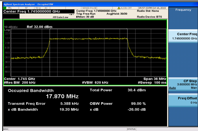
Band4-20MHz-QPSK-20300-100RB#0-17.870
