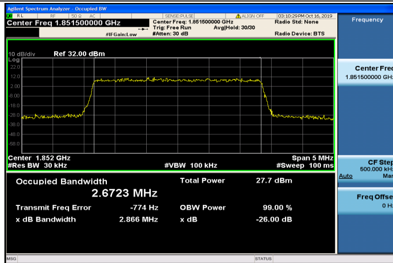
Band2-3MHz-16QAM-18615-15RB#0-2.6723
