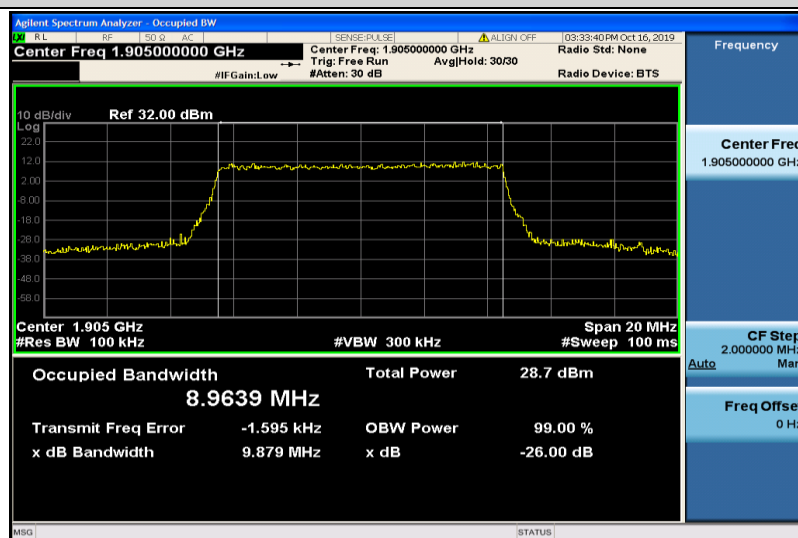
Band2-10MHz-QPSK-19150-50RB#0-8.9639
