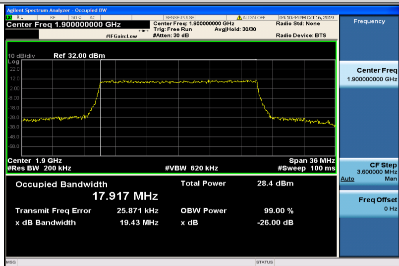
Band2-20MHz-16QAM-19100-100RB#0-17.917
