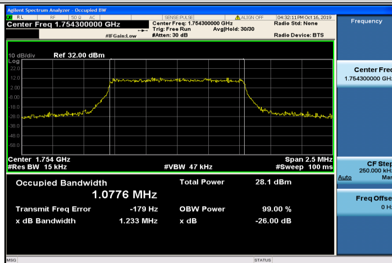
Band4-1.4MHz-16QAM-20393-6RB#0-1.0776
