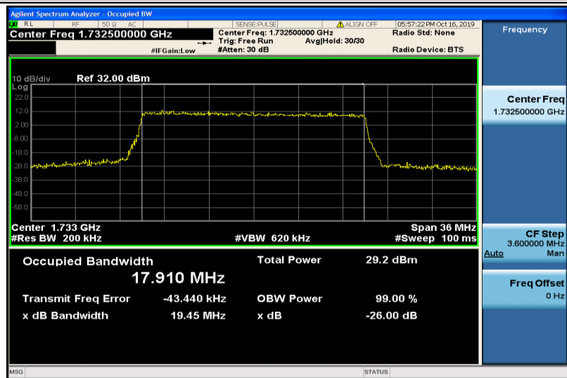
Band4-20MHz-16QAM-20175-100RB#0-17.910
