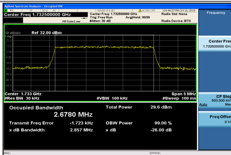
Band4-3MHz-QPSK-20175-15RB#0-2.6780
