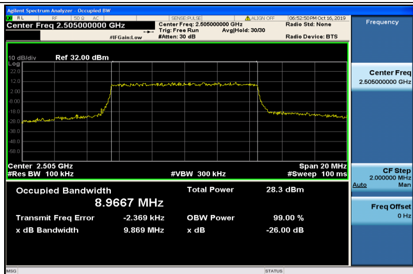
Band7-10MHz-QPSK-20800-50RB#0-8.9667
