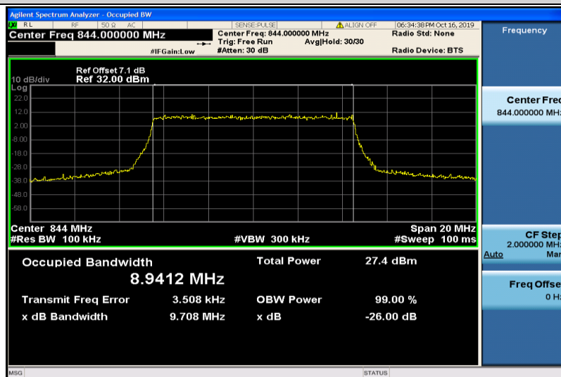
Band5-10MHz-16QAM-20600-50RB#0-8.9412
