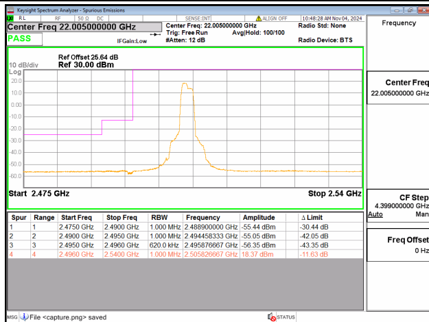
41C / 10+20MHz / Low CH / QPSK / 1#49-1#0
