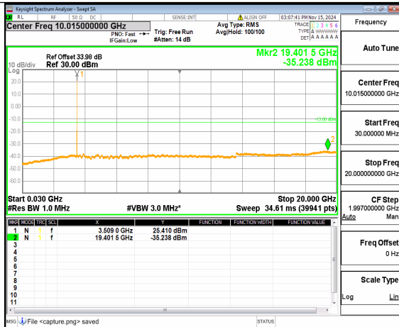
n78(3450-3550MHz) (30MHz-20GHz) 20M DFT-s-OFDM BPSK Inner_1RB_Right Mid
