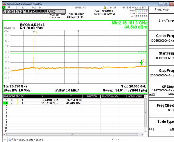
n78(3450-3550MHz) (30MHz-20GHz) 20M DFT-s-OFDM BPSK Inner_1RB_Right High
