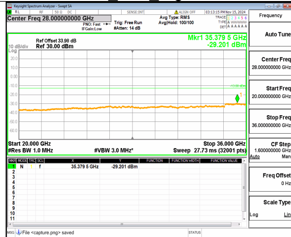
n78(3450-3550MHz) (20GHz-36GHz) 20M DFT-s-OFDM BPSK Inner_1RB_Left High
