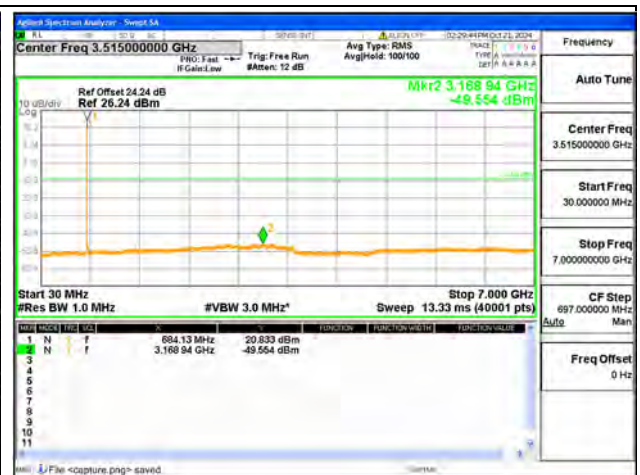
B71 / 15MHz / High CH / 16QAM
