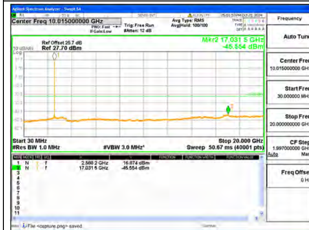
B38-30M-20G / 15MHz / Mid CH / QPSK
