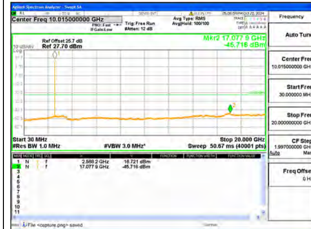
B41-30M-20G / 10MHz / Mid CH / QPSK
