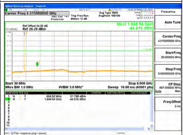
B26 Part22 / 3MHz / Low CH / QPSK
