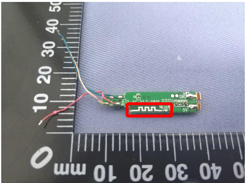
BT Antenna
