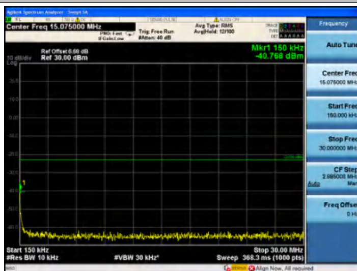
Band V_4132
