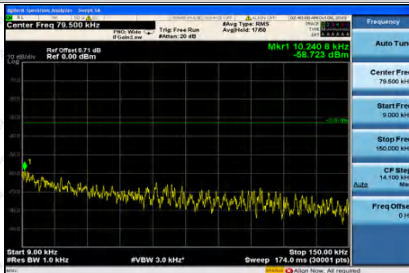
EGPRS850-251-0.009-0.15
