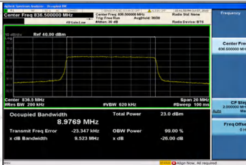
Band5-10MHz-QPSK-20600-50RB#0-8.9913
