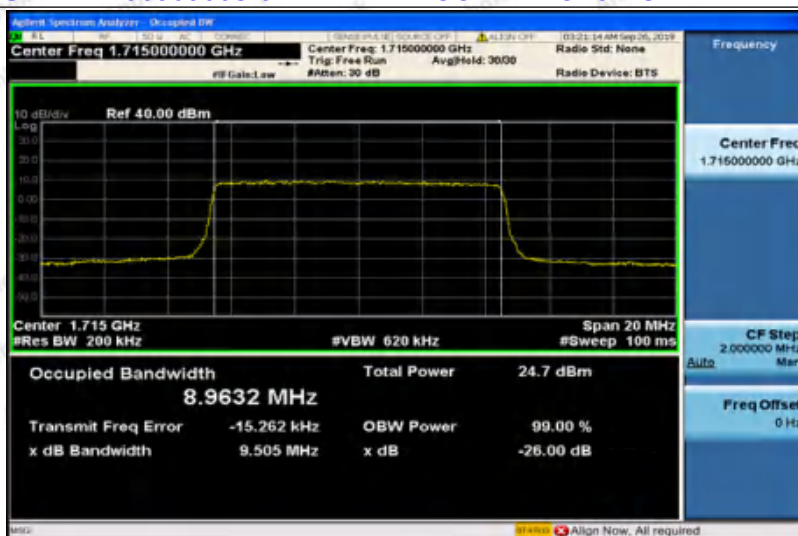
Band4-10MHz-QPSK-20175-50RB#0-8.9680
