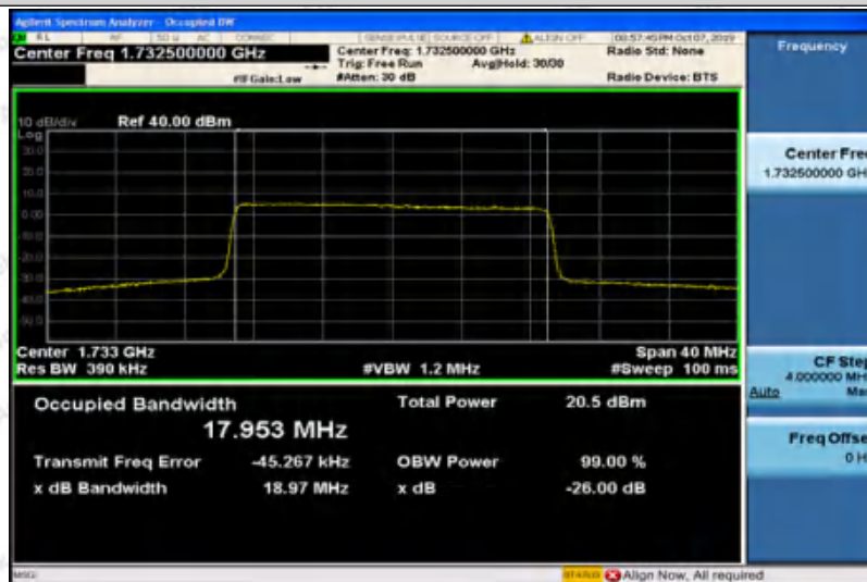
Band4-20MHz-16QAM-20300-100RB#0-17.986
