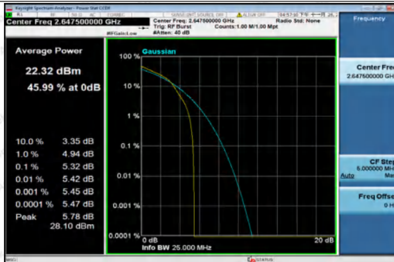
Band41-15MHz-16QAM-41165-5RB#0
