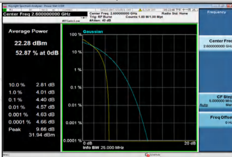
Band41-20MHz-QPSK-40690-100RB#0
