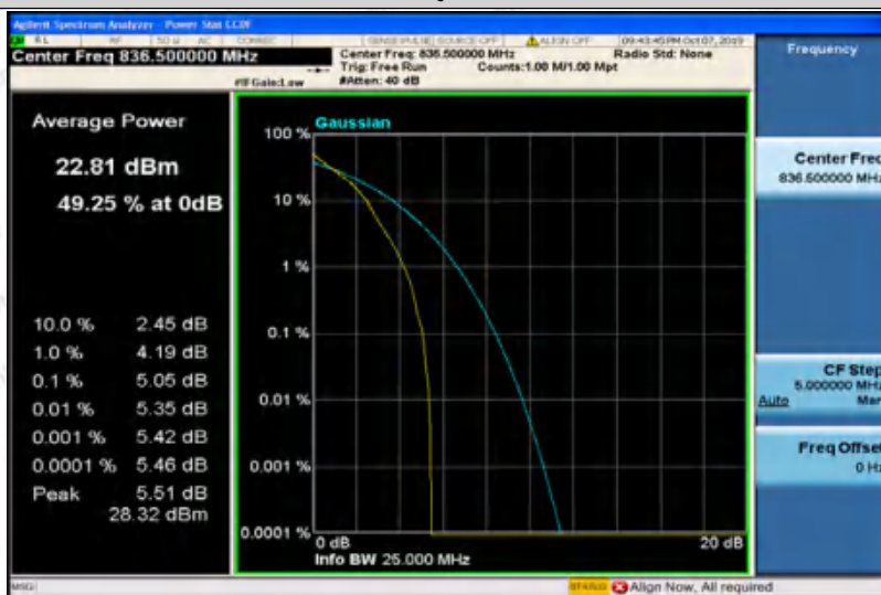
Band5-1.4MHz-QPSK-20525-6RB#0
