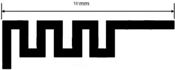
Antenna Photo & Length (mm)
