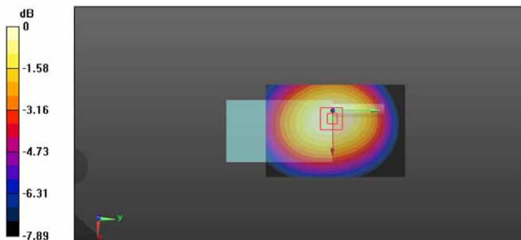
Figure 2: Face held for FM Modulation at 12.5KHz Channel Separation Front towards Phantom 467.6375 MHz
