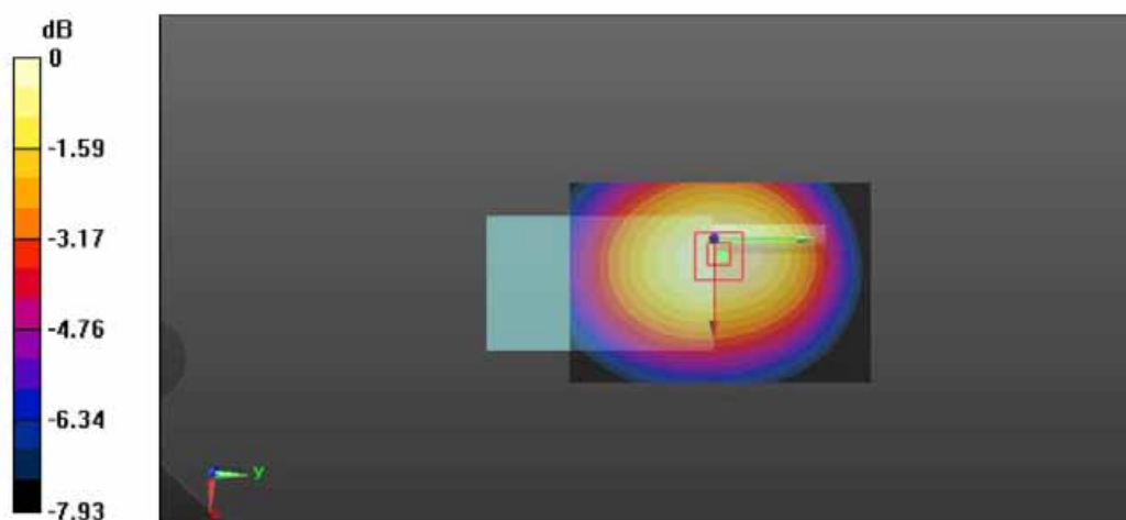
Figure 1: Face held for FM Modulation at 12.5KHz Channel Separation Front towards Phantom 462.6375 MHz
