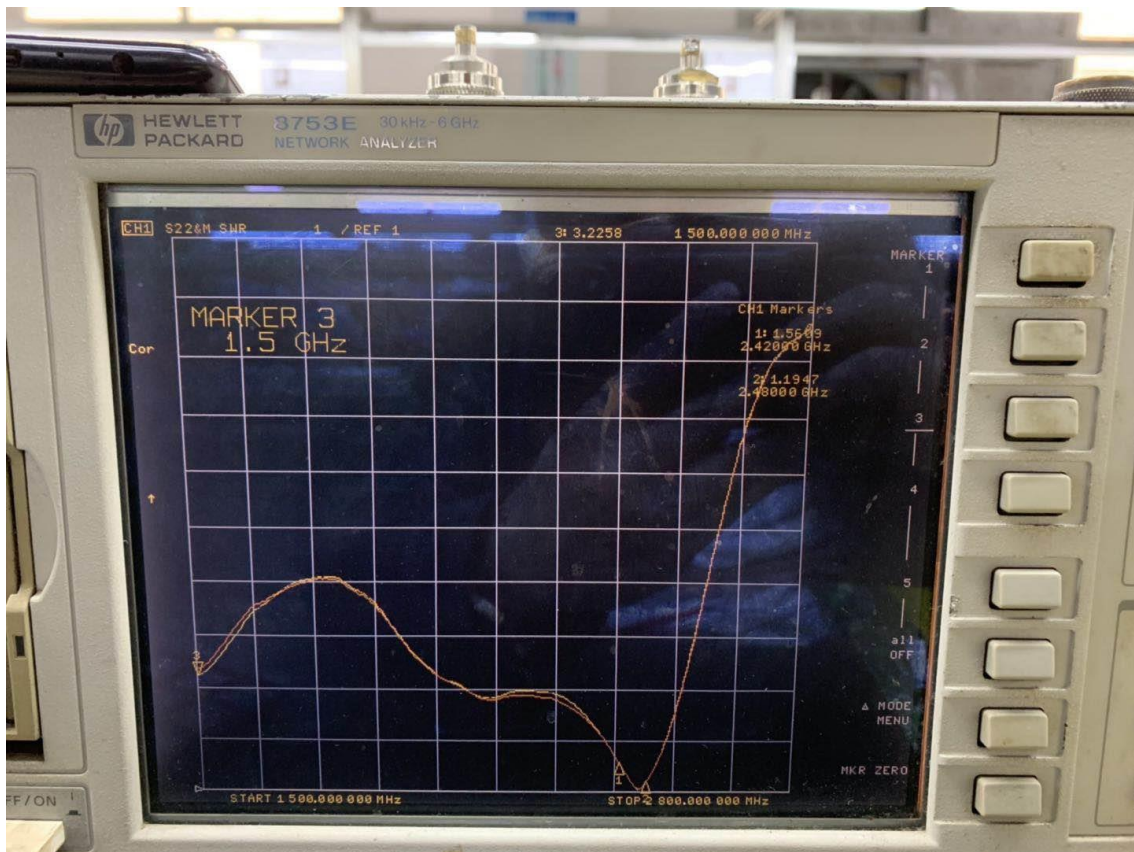
BT antenna standing wave ratio curve
