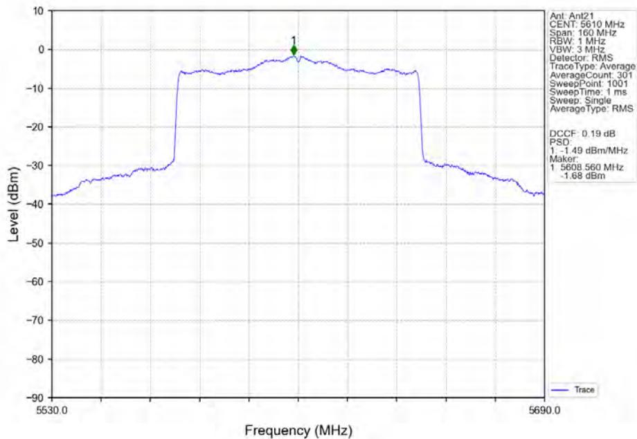
802.11ax(HEW80)_HCH_5610MHz_SU_/_Ant21_NTNV
