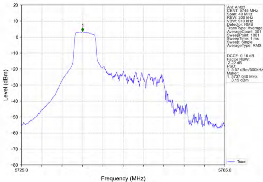
802.11ax(HEW20)_LCH_5745MHz_RU52_Left_Ant23_NTNV
