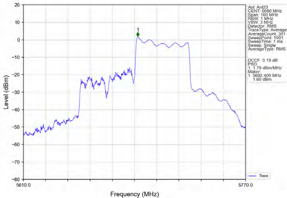
802.11ax(HEW80)_HCH_5690MHz_RU484_Right_Ant23_NTNV
