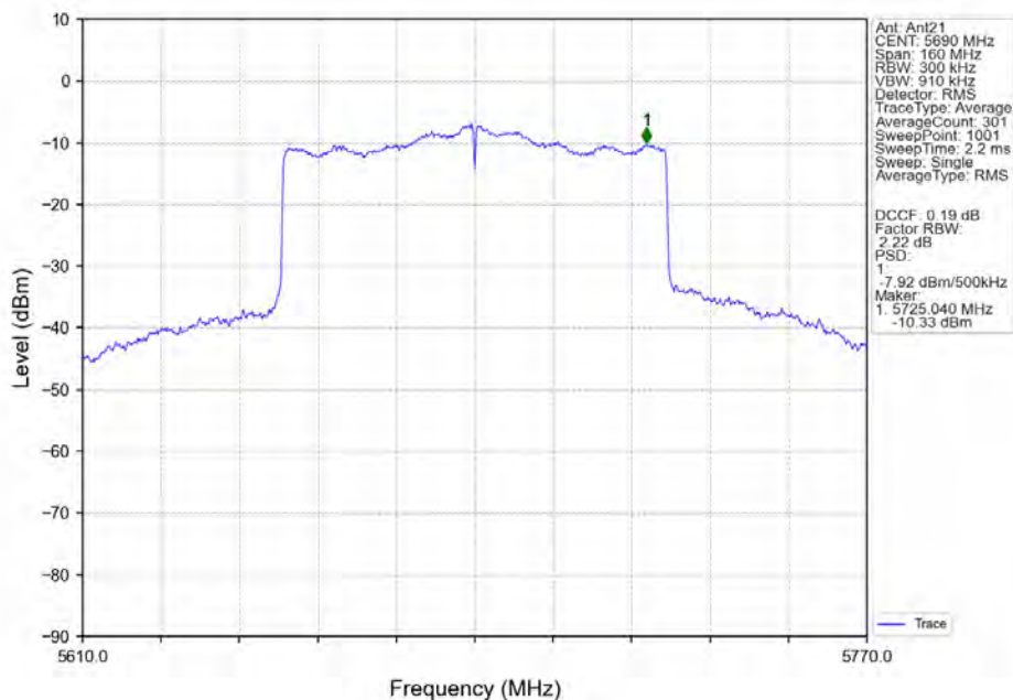
802.11ax(HEW80)_HCH_5690MHz_SU_/_Ant21_NTNV
