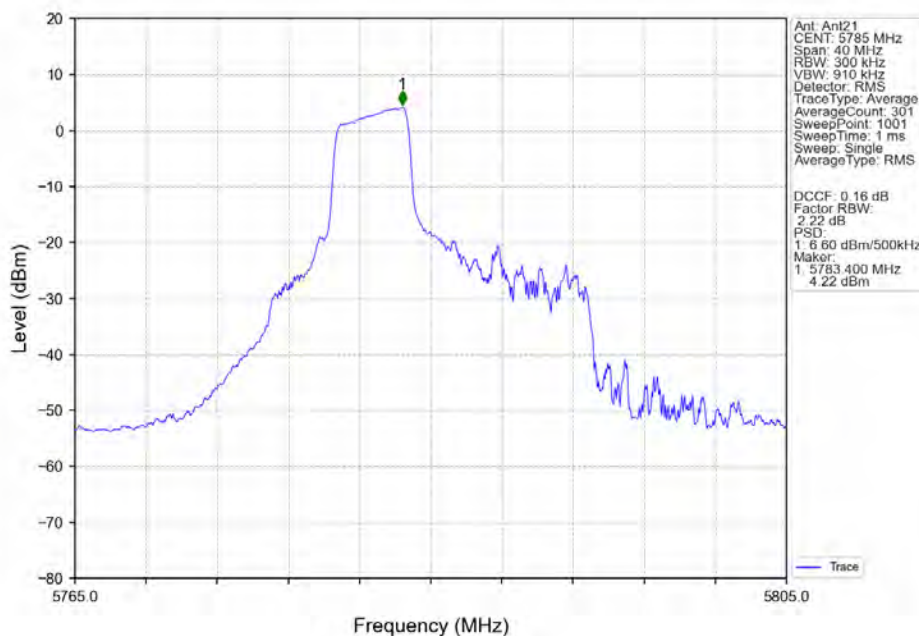
802.11ax(HEW20)_MCH_5785MHz_RU52_Mid_MIMO_NTNV
