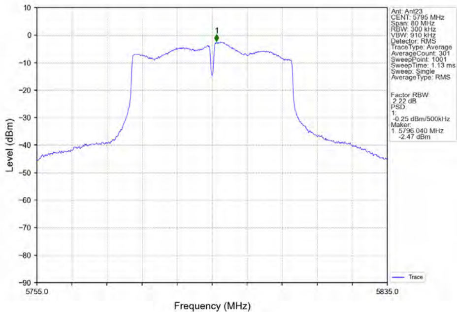
802.11n(HT40)_HCH_5795MHz_Ant23_NTNV
