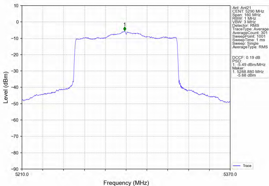
802.11ax(HEW80)_MCH_5290MHz_SU_/_Ant21_NTNV
