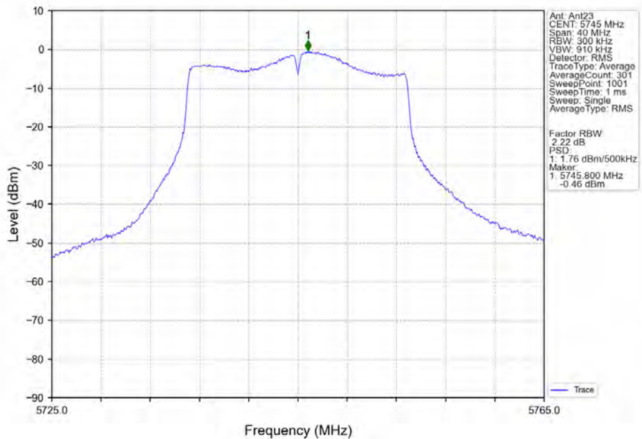
802.11ac(VHT20)_LCH_5745MHz_Ant23_NTNV
