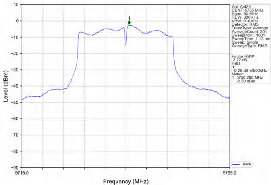
802.11ac(VHT40)_LCH_5755MHz_Ant23_NTNV
