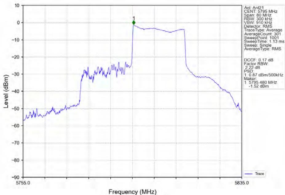
802.11ax(HEW40)_HCH_5795MHz_RU242_Right_Ant21_NTNV
