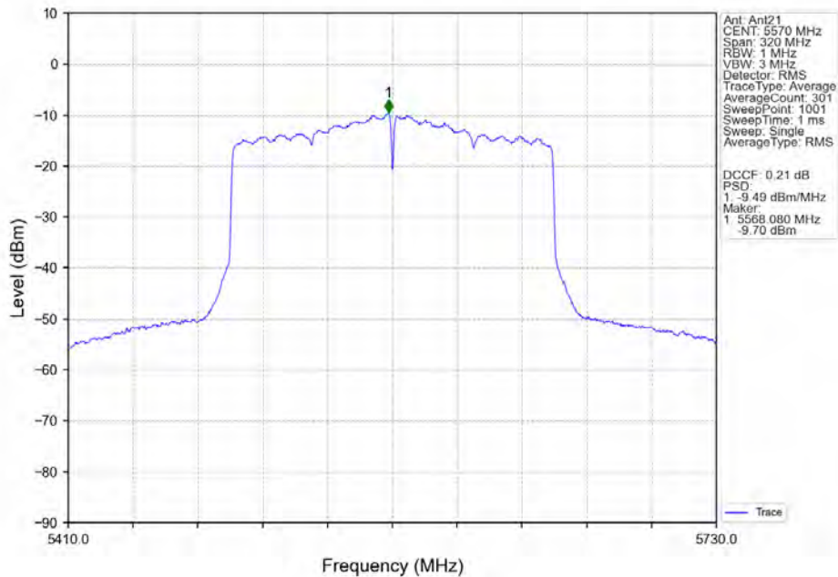
802.11ax(HEW160)_MCH_5570MHz_SU_/_MIMO_NTNV
