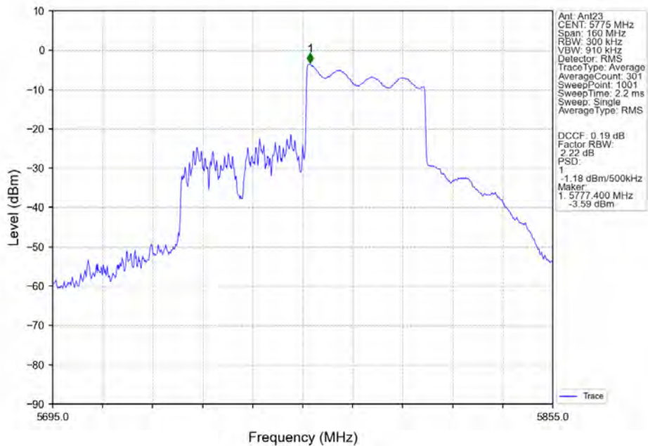
802.11ax(HEW80)_MCH_5775MHz_RU484_Right_Ant23_NTNV
