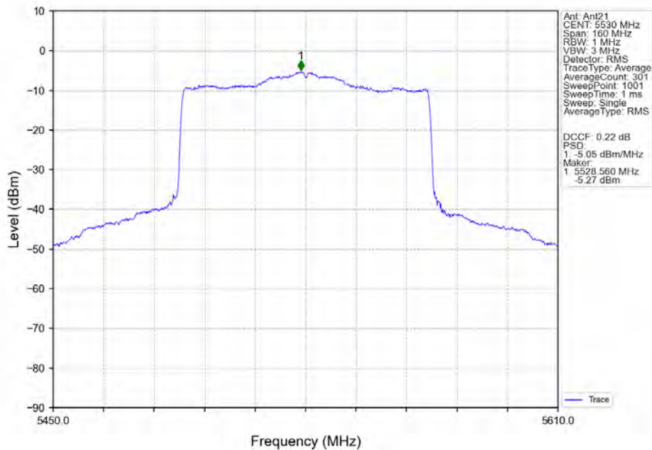
802.11ax(HEW80)_LCH_5530MHz_SU_/_Ant21_NTNV
