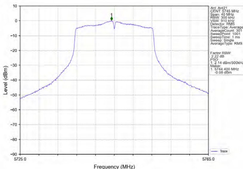
802.11a_LCH_5745MHz_Ant21_NTNV
