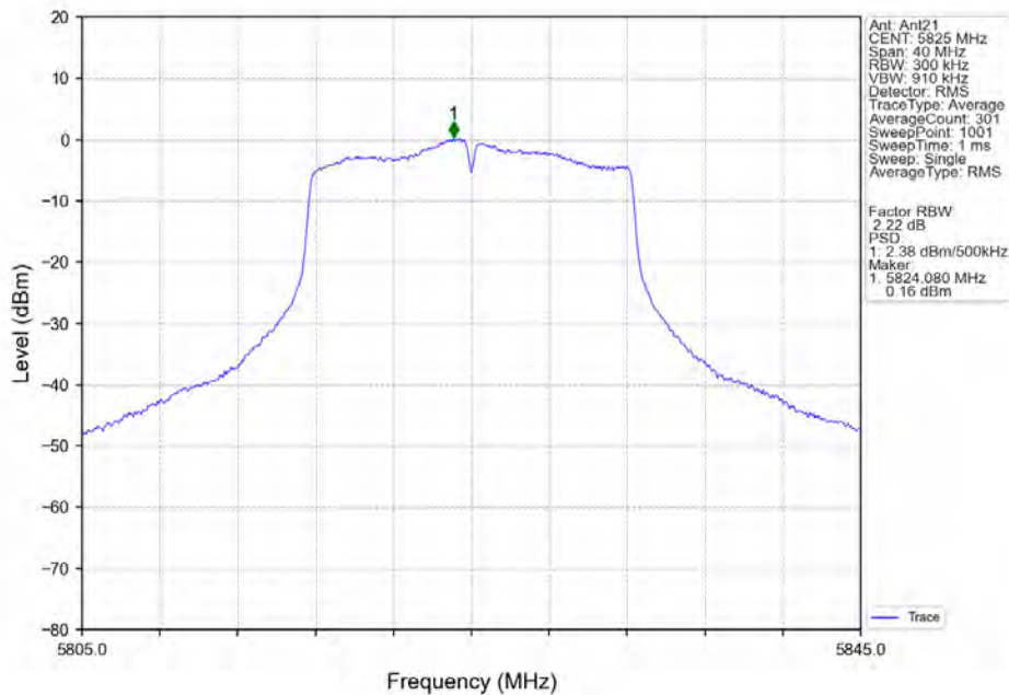
802.11a_HCH_5825MHz_Ant21_NTNV
