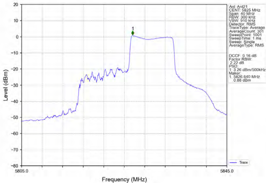
802.11ax(HEW20)_HCH_5825MHz_RU106_Right_Ant21_NTNV
