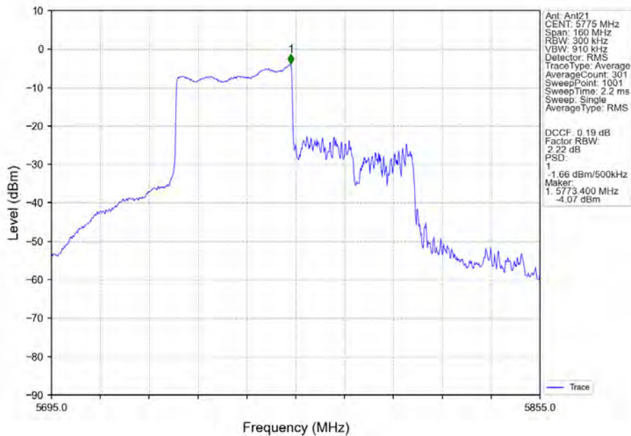
802.11ax(HEW80)_MCH_5775MHz_RU484_Left_Ant21_NTNV
