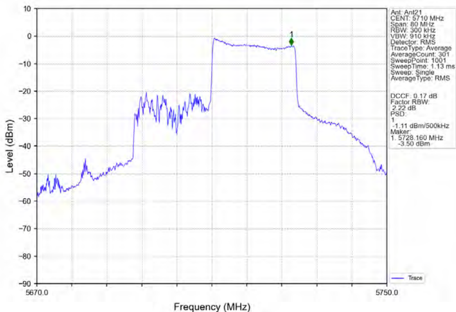
802.11ax(HEW40)_HCH_5710MHz_RU242_Right_Ant21_NTNV
