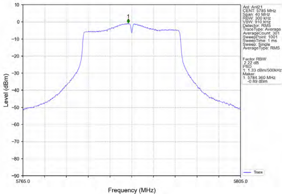
802.11ac(VHT20)_MCH_5785MHz_Ant21_NTNV
