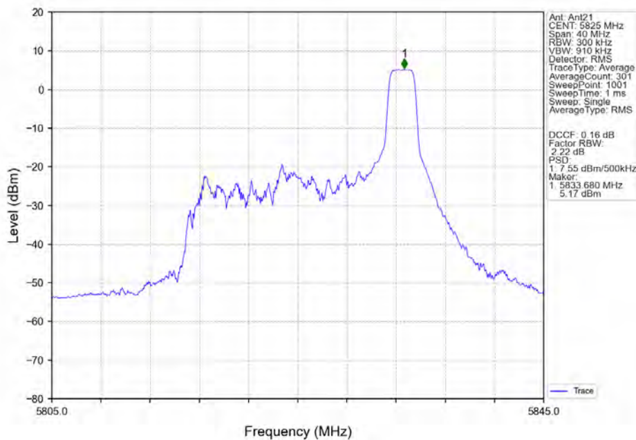
802.11ax(HEW20)_HCH_5825MHz_RU26_Right_Ant21_NTNV
