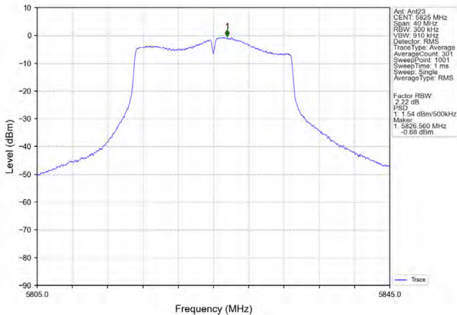
802.11ac(VHT20)_HCH_5825MHz_Ant23_NTNV
