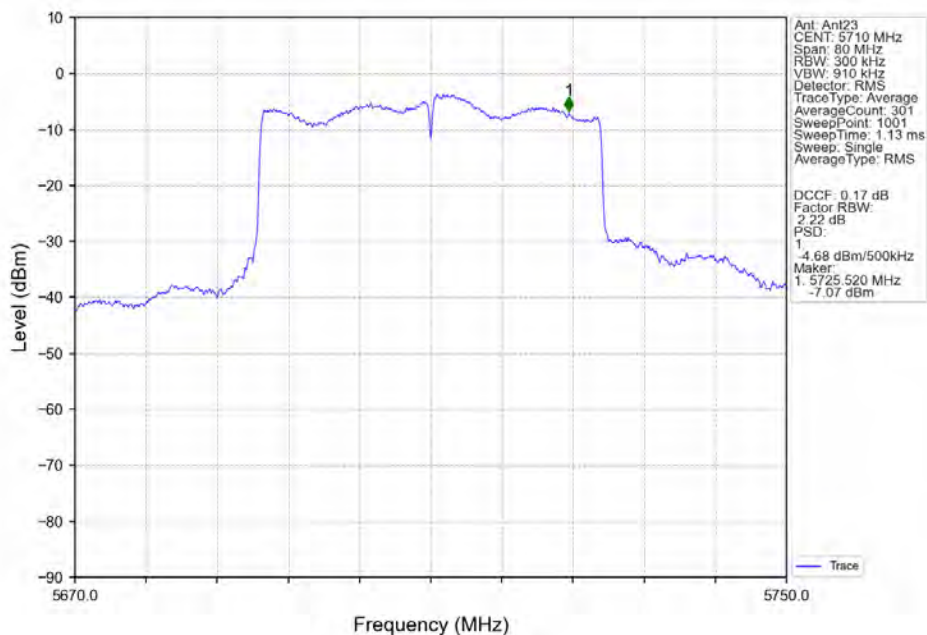
802.11ax(HEW40)_HCH_5710MHz_SU_/_Ant23_NTNV
