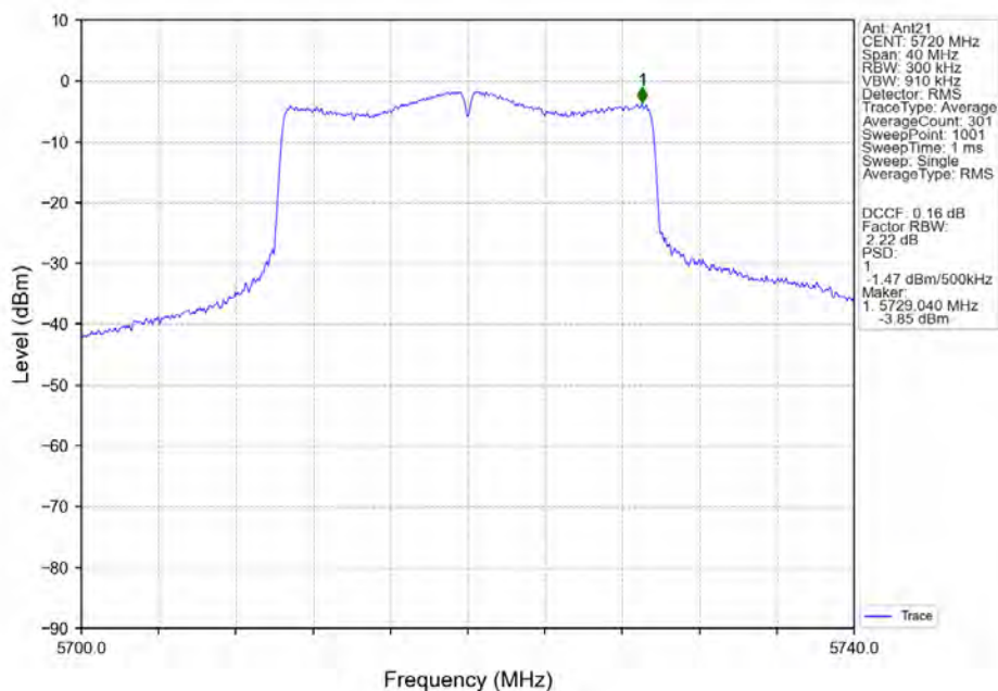
802.11ax(HEW20)_HCH_5720MHz_SU_/_MIMO_NTNV
