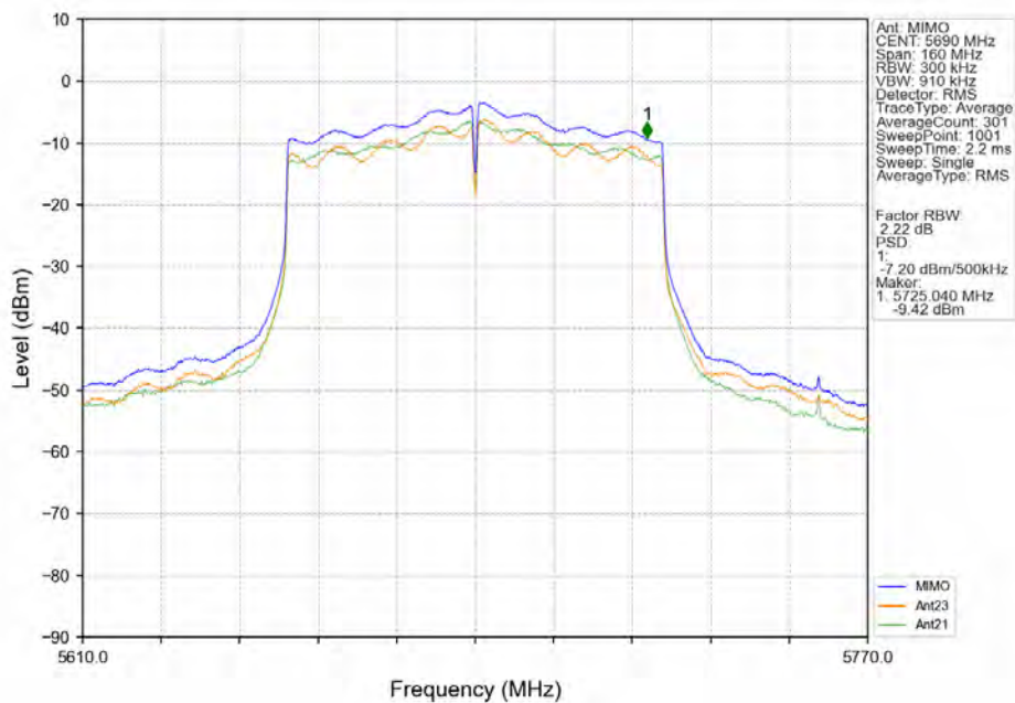
802.11ac(VHT80)_HCH_5690MHz_MIMO_NTNV
