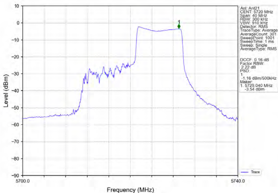
802.11ax(HEW20)_HCH_5720MHz_RU106_Right_Ant21_NTNV
