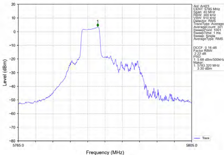
802.11ax(HEW20)_MCH_5785MHz_RU52_Mid_Ant23_NTNV
