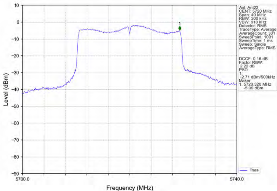
802.11ax(HEW20)_HCH_5720MHz_SU_/_Ant23_NTNV
