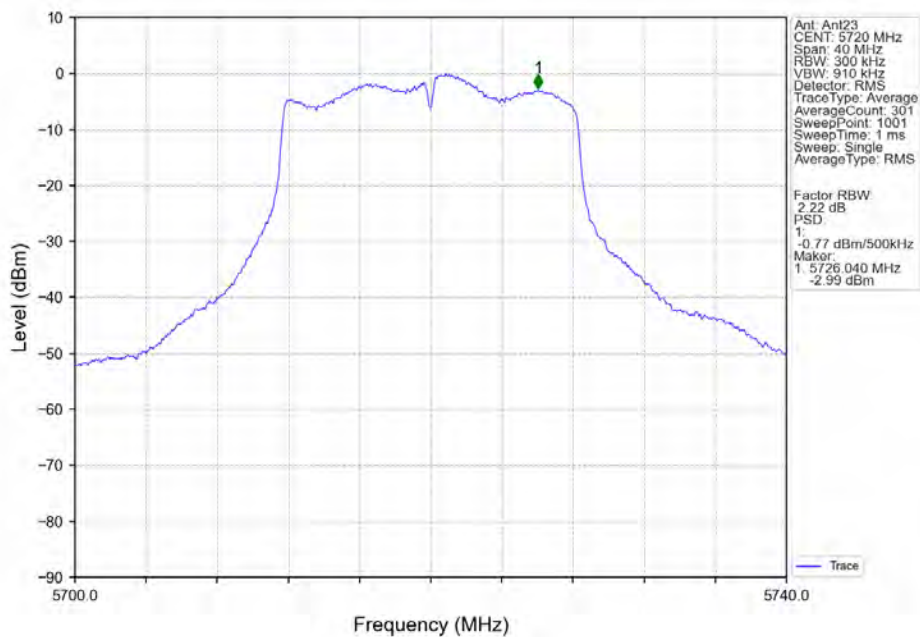
802.11a_HCH_5720MHz_Ant23_NTNV
