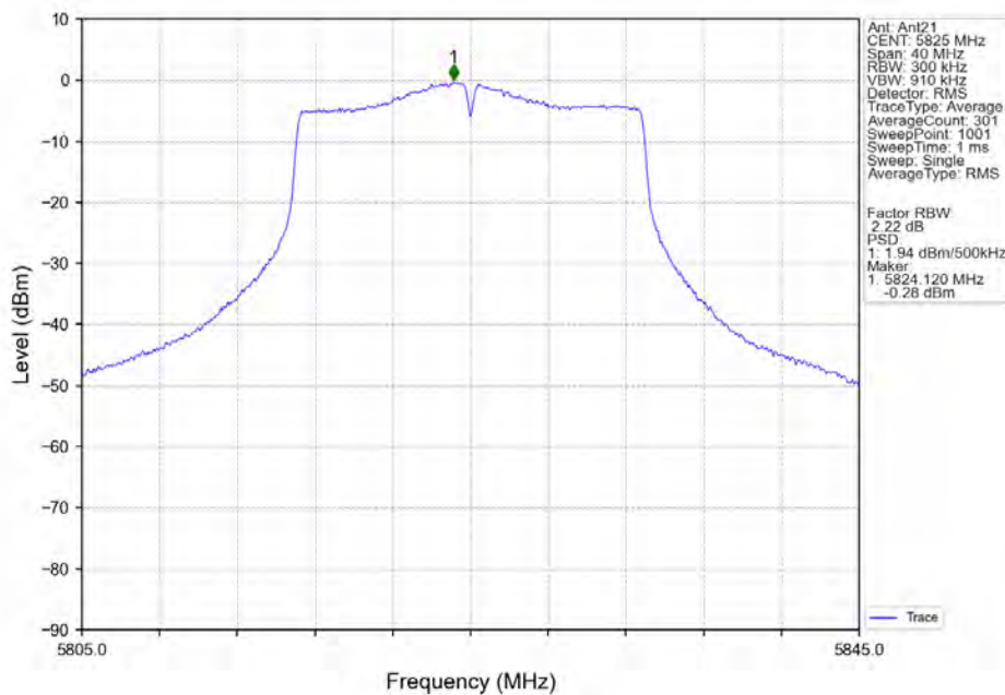
802.11n(HT20)_HCH_5825MHz_Ant21_NTNV
