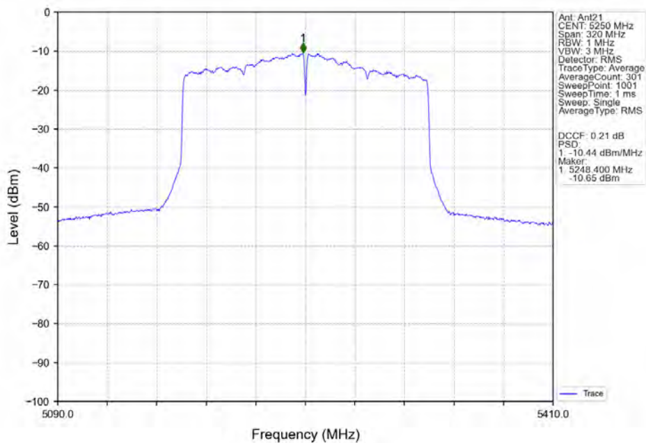
802.11ax(HEW160)_MCH_5250MHz_SU_/_Ant21_NTNV
