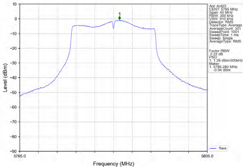
802.11n(HT20)_MCH_5785MHz_Ant23_NTNV
