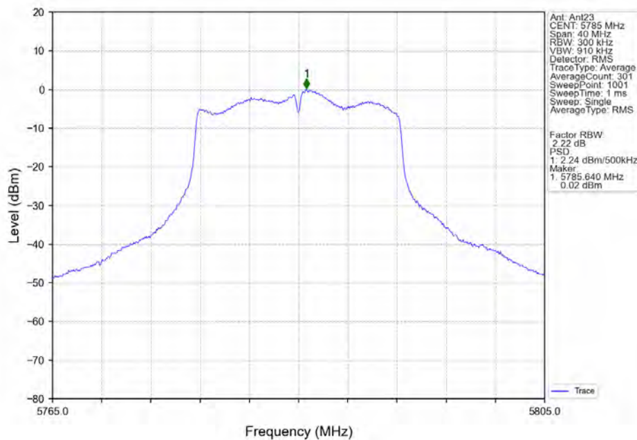
802.11a_MCH_5785MHz_Ant23_NTNV
