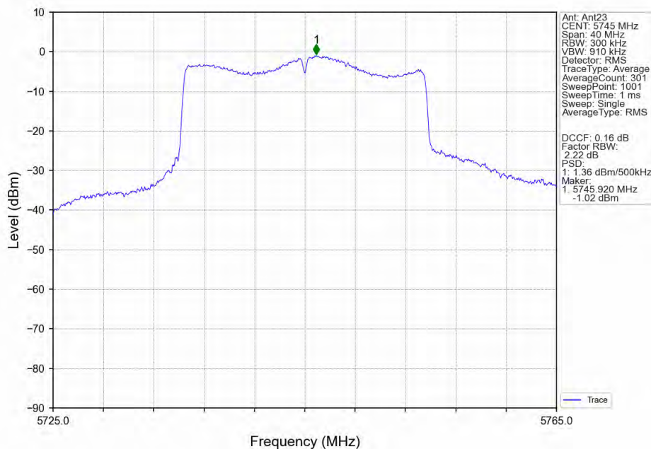
802.11ax(HEW20)_LCH_5745MHz_SU_/_Ant23_NTNV
