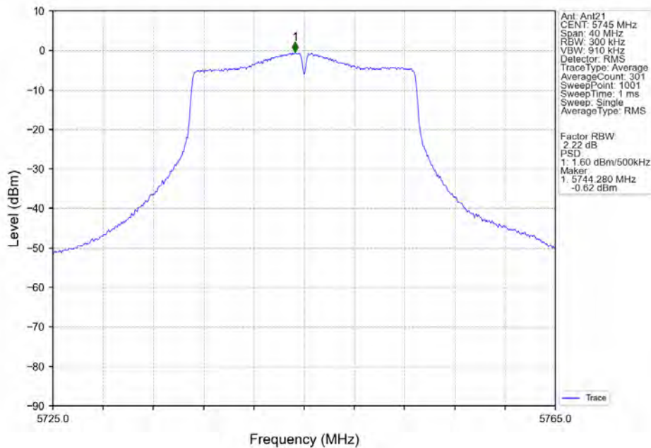
802.11n(HT20)_LCH_5745MHz_Ant21_NTNV
