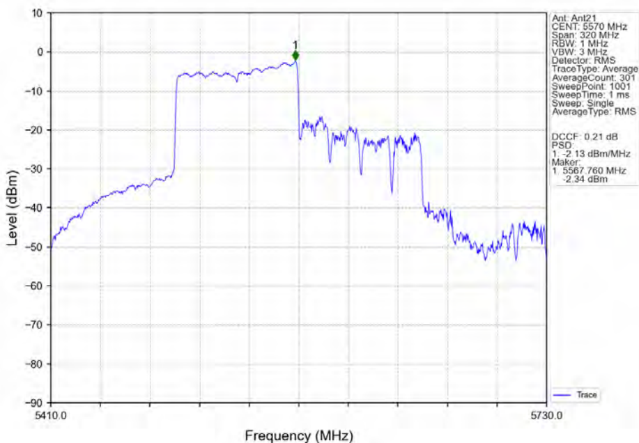
802.11ax(HEW160)_MCH_5570MHz_RU996_Left_MIMO_NTNV
