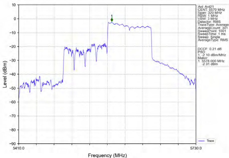
802.11ax(HEW160)_MCH_5570MHz_RU996_Right_Ant21_NTNV
