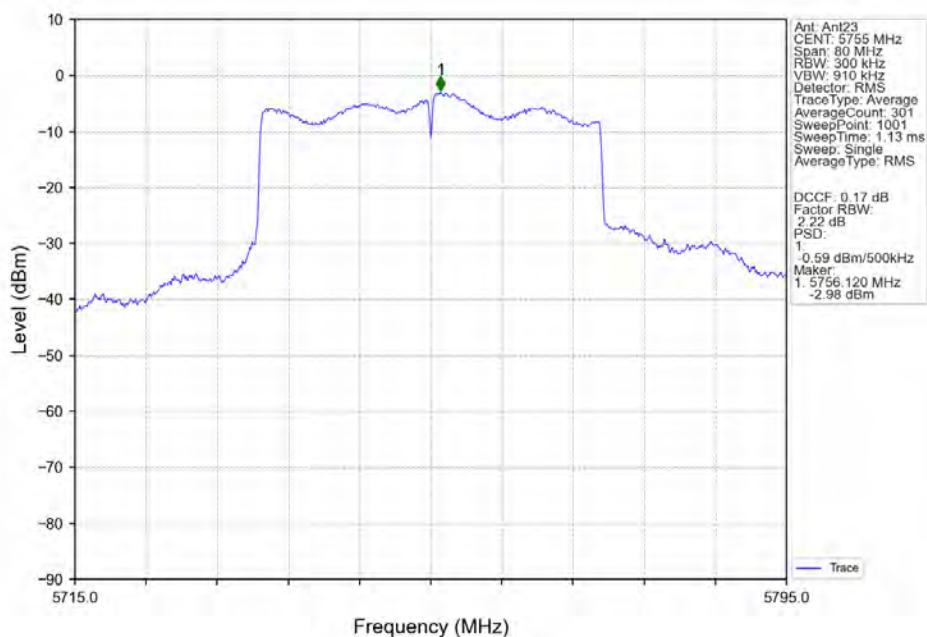
802.11ax(HEW40)_LCH_5755MHz_SU_/_Ant23_NTNV
