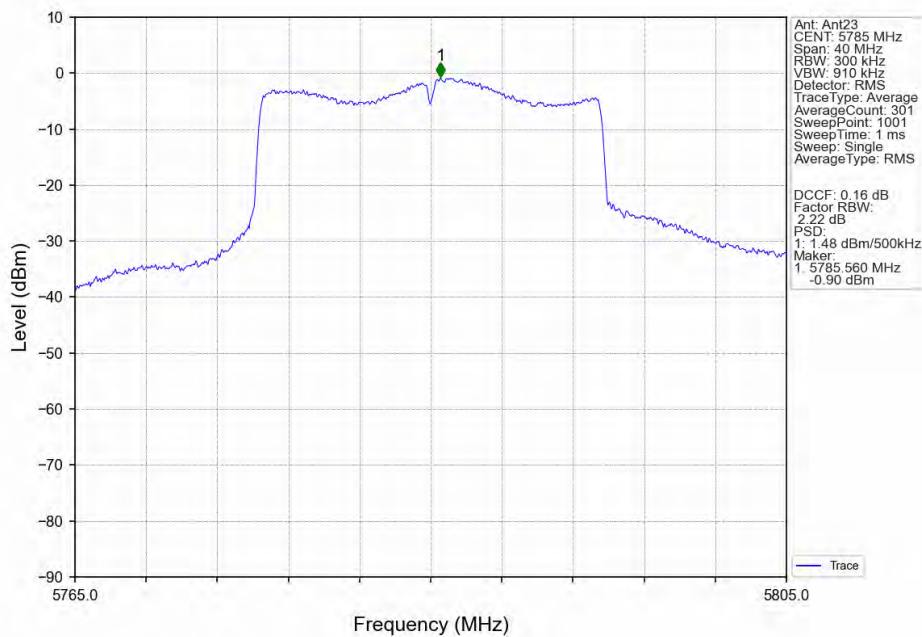
802.11ax(HEW20)_MCH_5785MHz_SU_/_Ant23_NTNV
