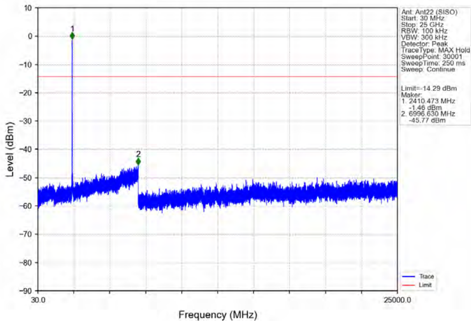
802.11ac(VHT20)_LCH_2412MHz_Ant22 (SISO)_NTNV
