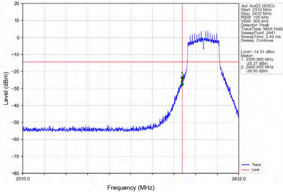
802.11n(HT20)_LCH_2412MHz_Ant22 (SISO)_NTNV
