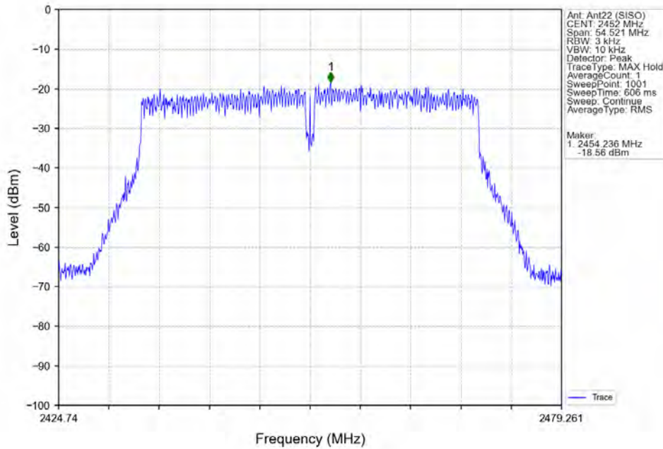
802.11ac(VHT40)_HCH_2452MHz_Ant22 (SISO)_NTNV
