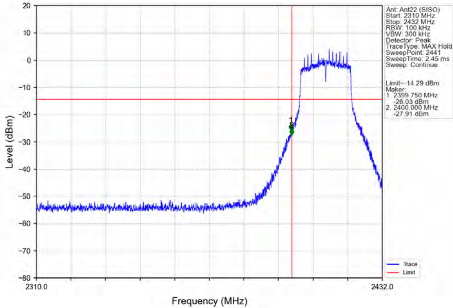
802.11ac(VHT20)_LCH_2412MHz_Ant22 (SISO)_NTNV
