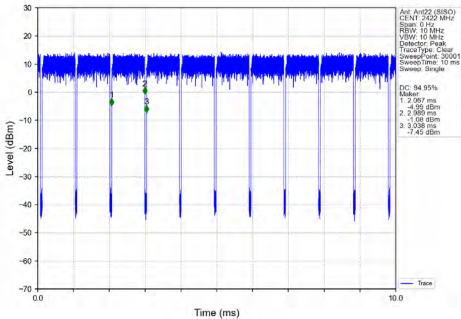
802.11n(HT40)_LCH_2422MHz_Ant22 (SISO)_NTNV
