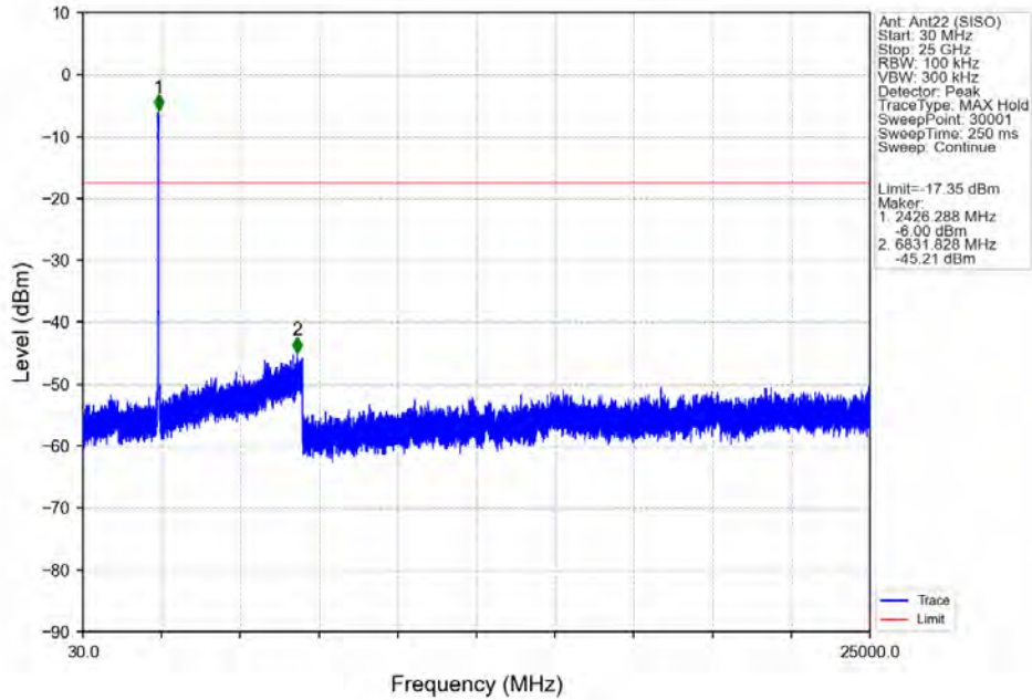
802.11ac(VHT40)_MCH_2437MHz_Ant22 (SISO)_NTNV
