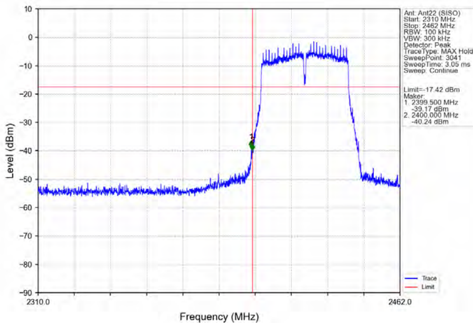
802.11n(HT40)_LCH_2422MHz_Ant22 (SISO)_NTNV
