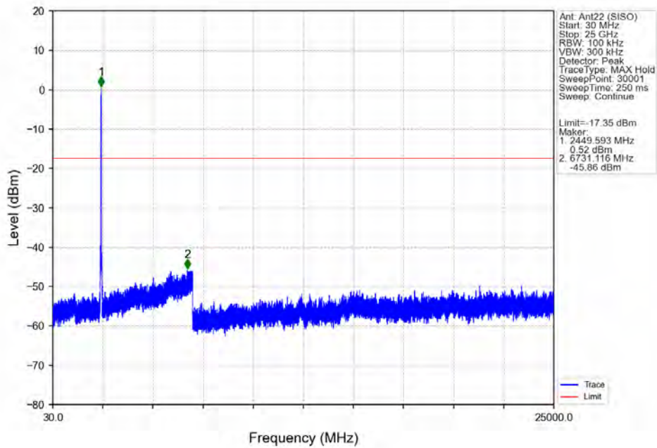
802.11ac(VHT40)_MCH_2437MHz_Ant22 (SISO)_NTNV
