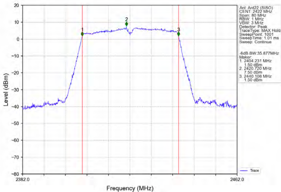
802.11ac(VHT40)_LCH_2422MHz_Ant22 (SISO)_NTNV
