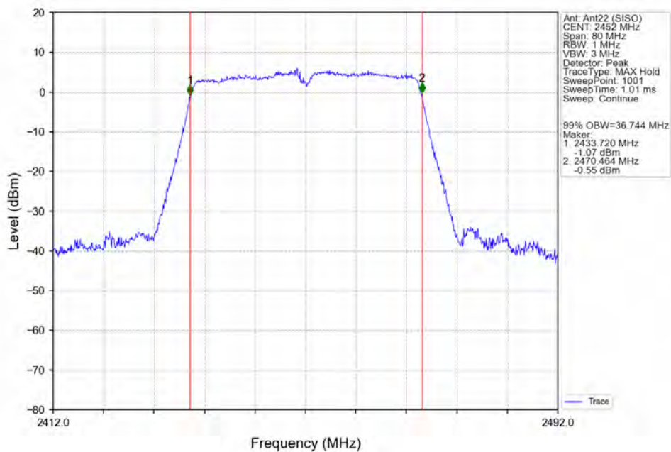
802.11ac(VHT40)_HCH_2452MHz_Ant22 (SISO)_NTNV
