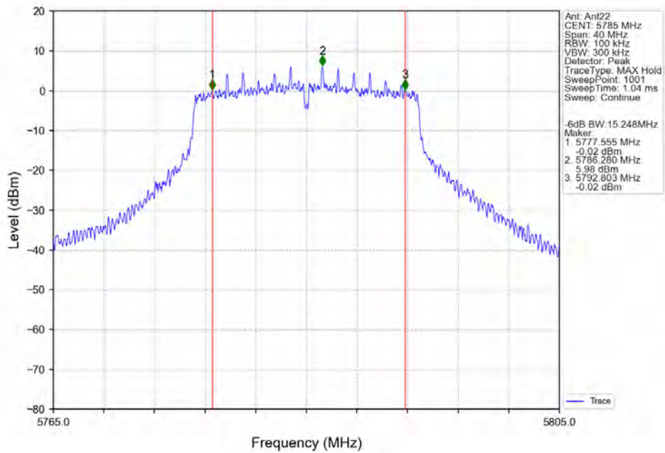
802.11ac(VHT20)_MCH_5785MHz_Ant22_NTNV
