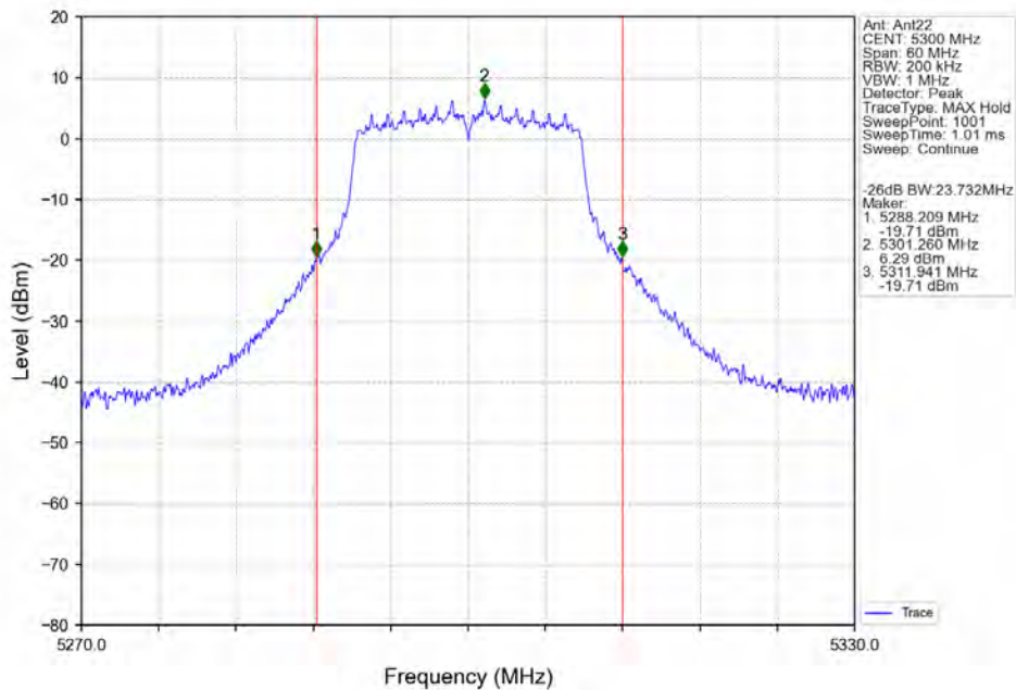
802.11n(HT20)_MCH_5300MHz_Ant22_NTNV
