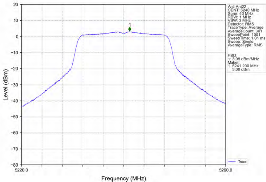
802.11ac(VHT20)_HCH_5240MHz_Ant22_NTNV
