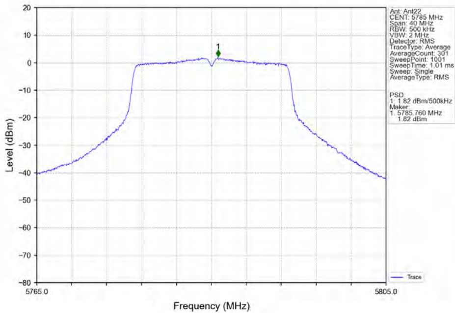
802.11ac(VHT20)_MCH_5785MHz_Ant22_NTNV
