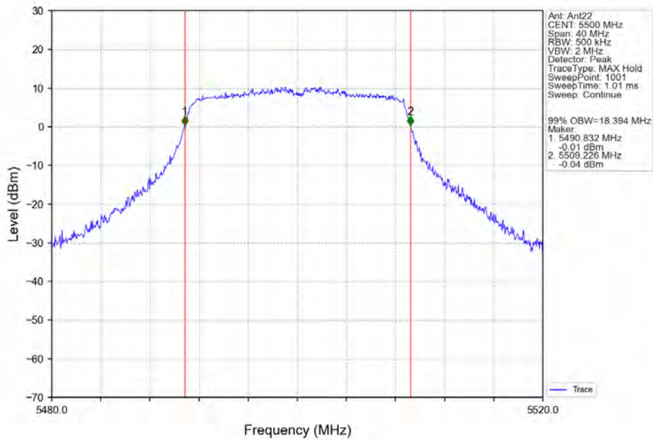
802.11ac(VHT20)_LCH_5500MHz_Ant22_NTNV
