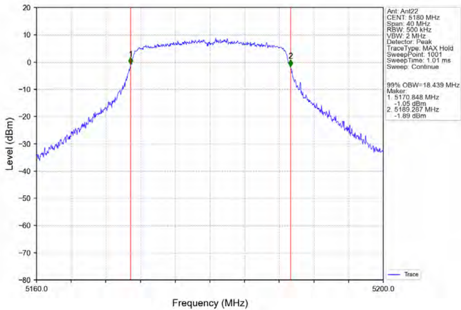
802.11ac(VHT20)_LCH_5180MHz_Ant22_NTNV
