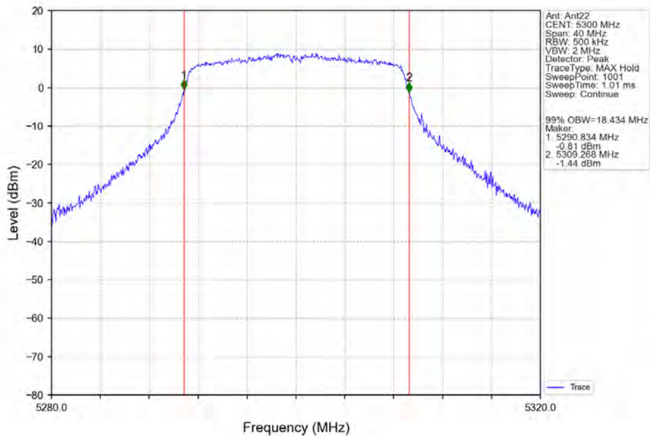
802.11ac(VHT20)_MCH_5300MHz_Ant22_NTNV
