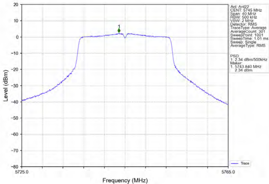
802.11n(HT20)_LCH_5745MHz_Ant22_NTNV
