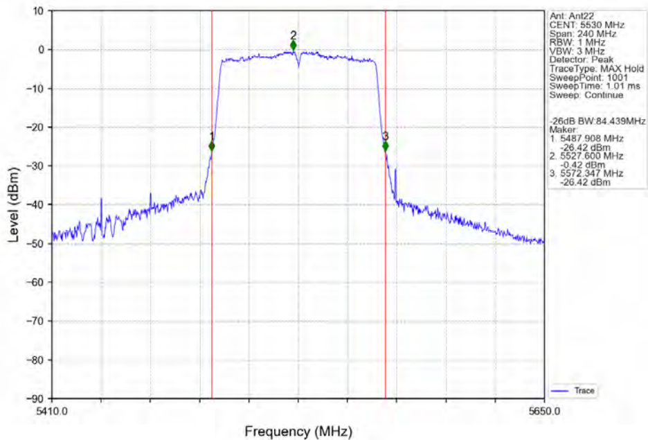
802.11ac(VHT80)_LCH_5530MHz_Ant22_NTNV
