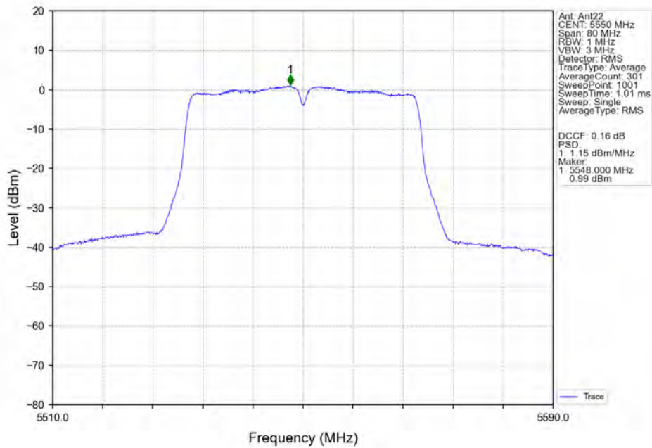
802.11n(HT40)_MCH_5550MHz_Ant22_NTNV
