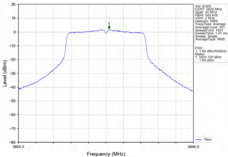
802.11n(HT20)_HCH_5825MHz_Ant22_NTNV
