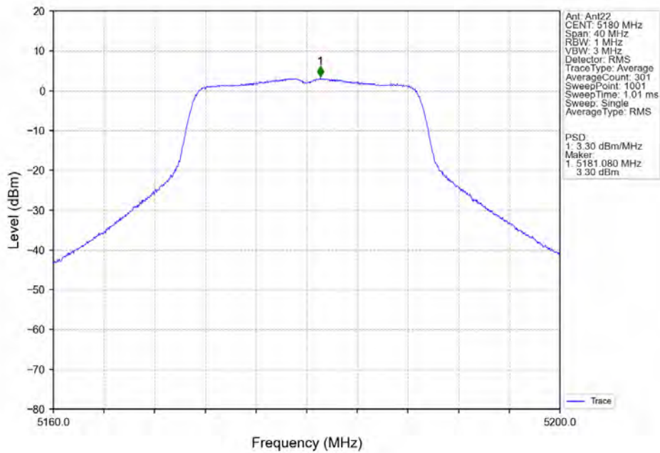
802.11ac(VHT20)_LCH_5180MHz_Ant22_NTNV
