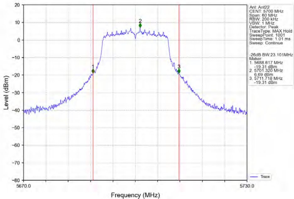
802.11ac(VHT20)_HCH_5700MHz_Ant22_NTNV
