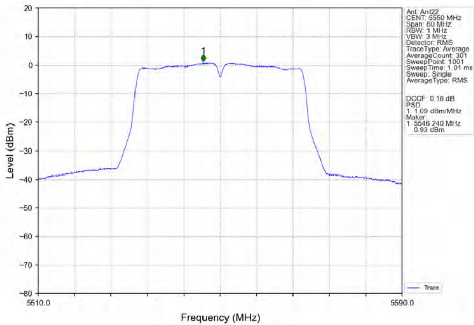
802.11ac(VHT40)_MCH_5550MHz_Ant22_NTNV
