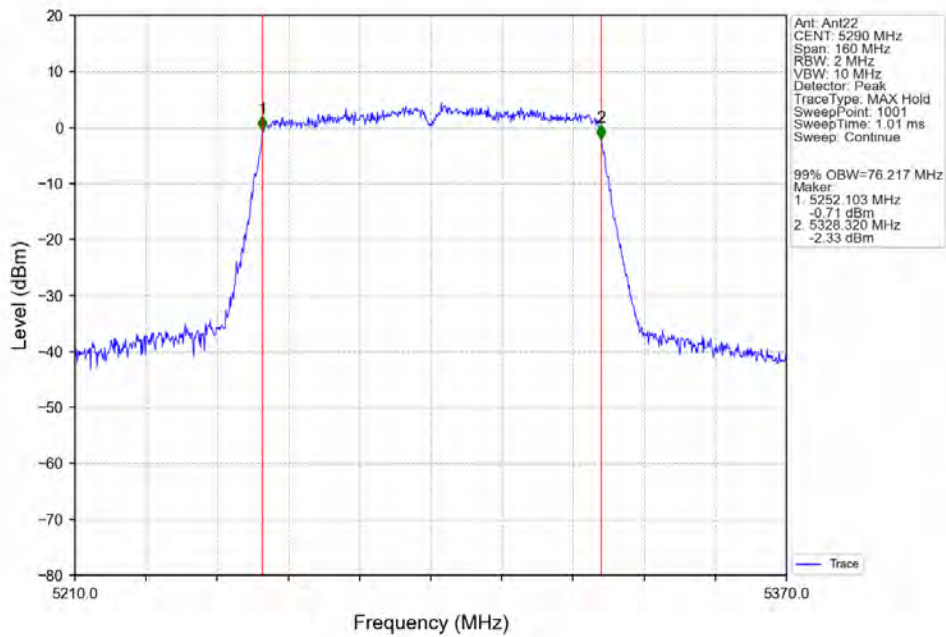
802.11ac(VHT80)_MCH_5290MHz_Ant22_NTNV
