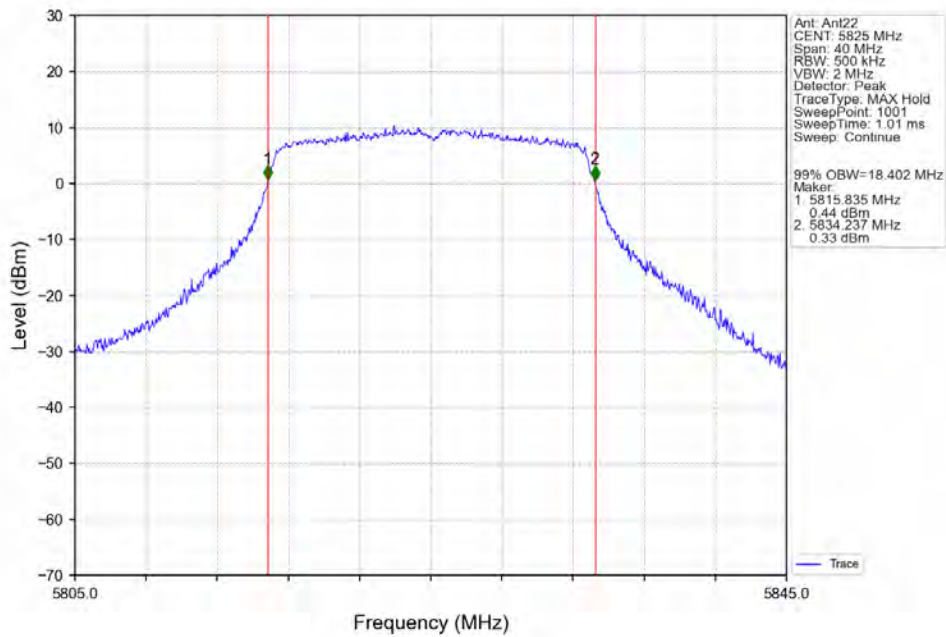
802.11n(HT20)_HCH_5825MHz_Ant22_NTNV
