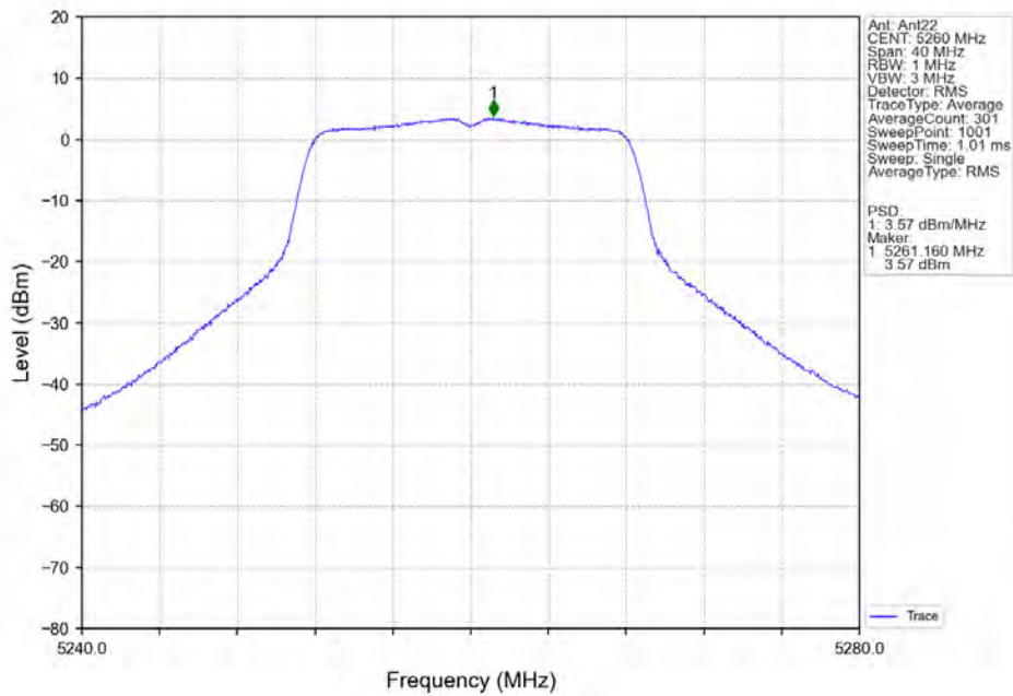
802.11a_LCH_5260MHz_Ant22_NTNV
