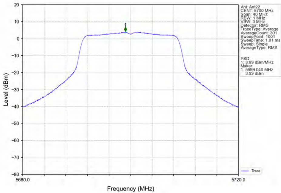
802.11n(HT20)_HCH_5700MHz_Ant22_NTNV
