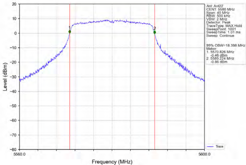
802.11n(HT20)_MCH_5580MHz_Ant22_NTNV
