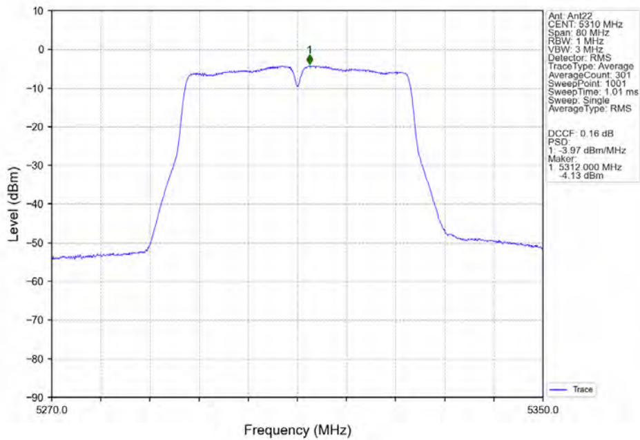
802.11ac(VHT40)_HCH_5310MHz_Ant22_NTNV
