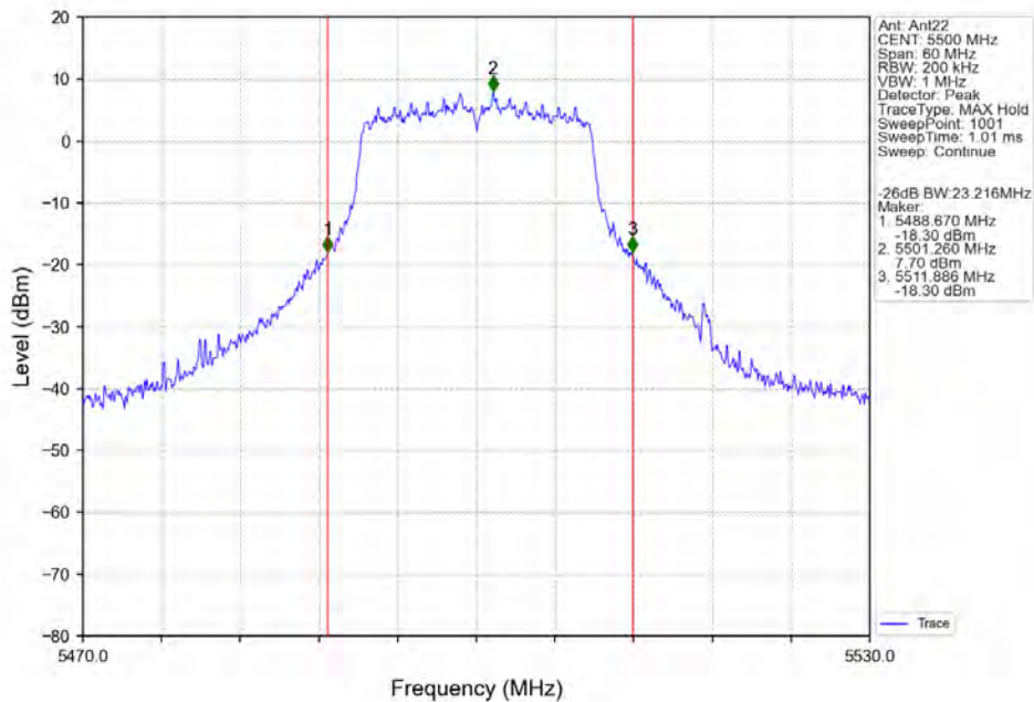
802.11ac(VHT20)_LCH_5500MHz_Ant22_NTNV
