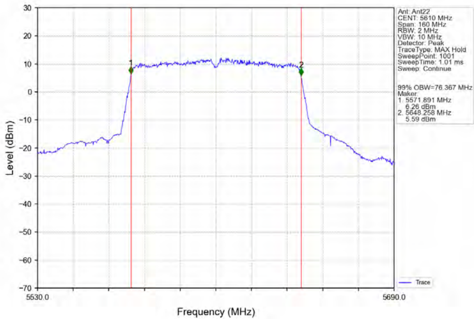
802.11ac(VHT80)_HCH_5610MHz_Ant22_NTNV
