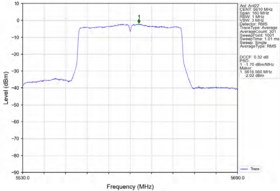
802.11ac(VHT80)_HCH_5610MHz_Ant22_NTNV
