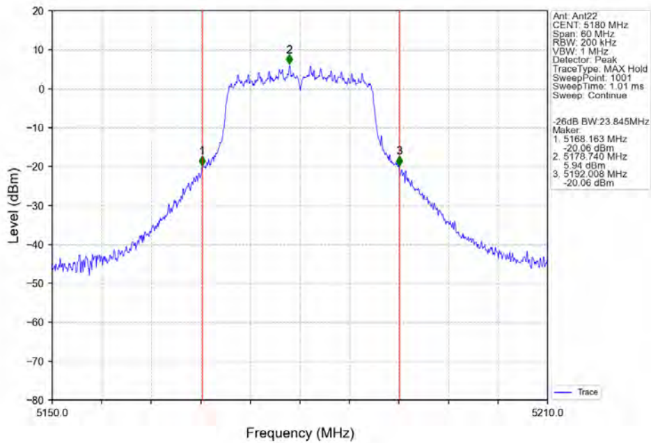
802.11ac(VHT20)_LCH_5180MHz_Ant22_NTNV
