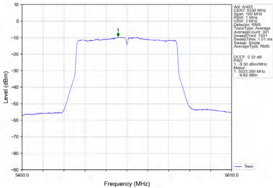
802.11ac(VHT80)_LCH_5530MHz_Ant22_NTNV
