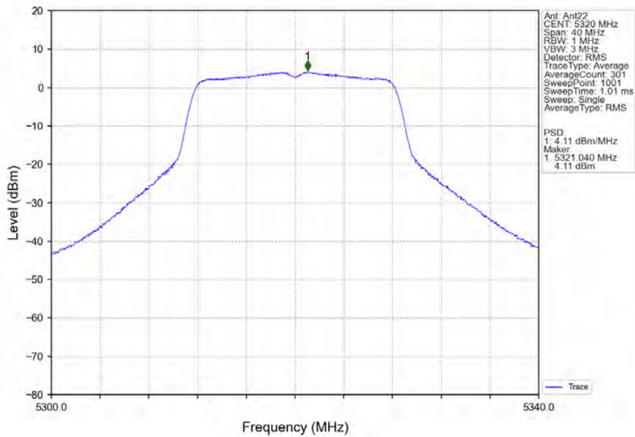
802.11a_HCH_5320MHz_Ant22_NTNV
