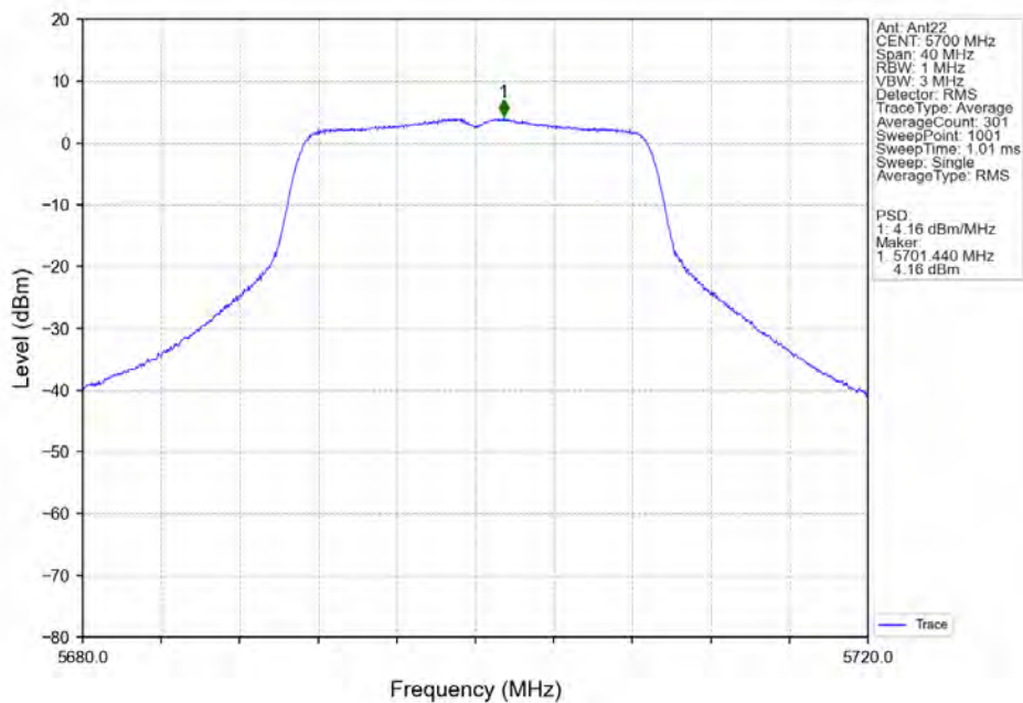
802.11ac(VHT20)_HCH_5700MHz_Ant22_NTNV
