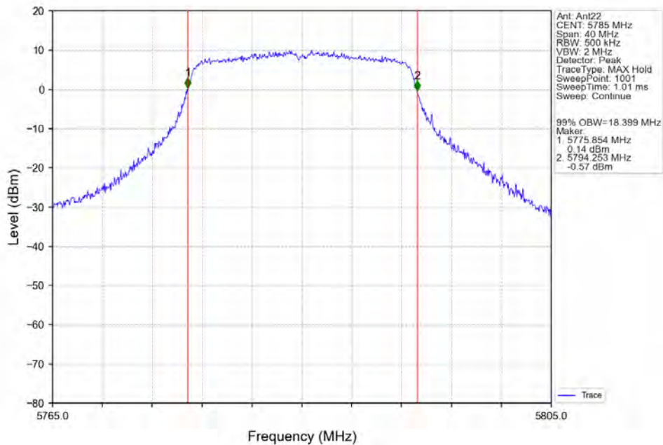
802.11ac(VHT20)_MCH_5785MHz_Ant22_NTNV
