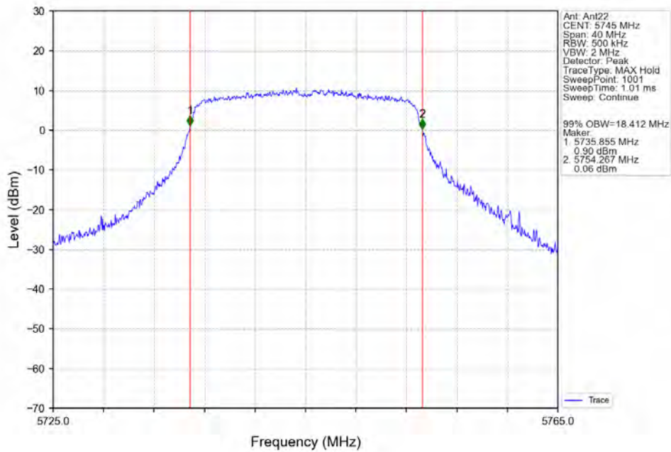
802.11n(HT20)_LCH_5745MHz_Ant22_NTNV
