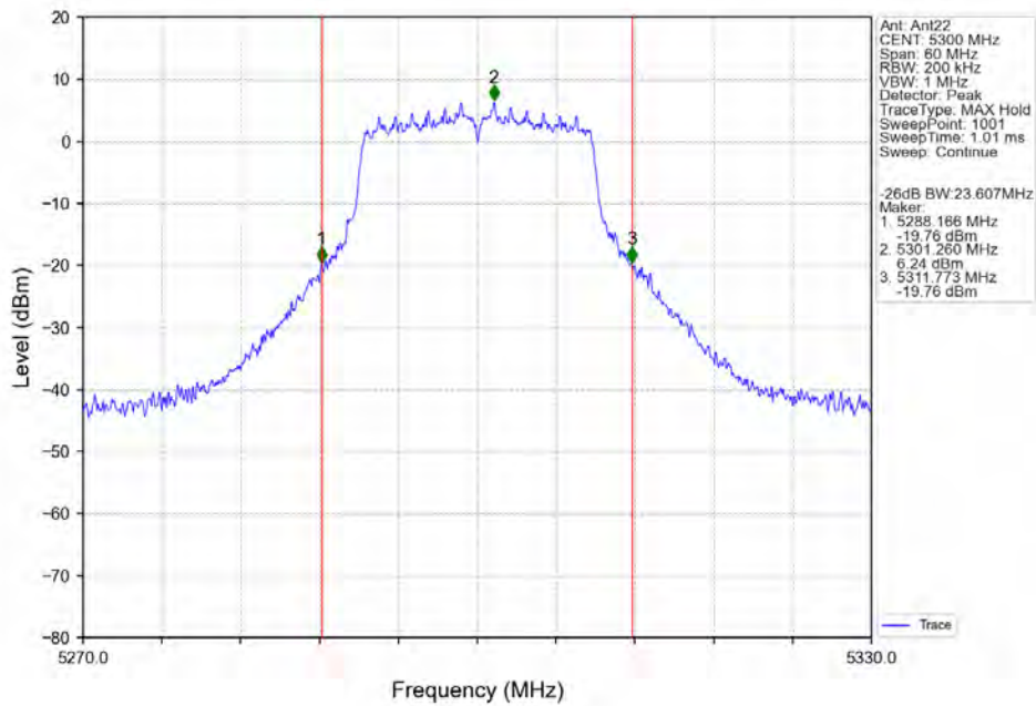
802.11ac(VHT20)_MCH_5300MHz_Ant22_NTNV
