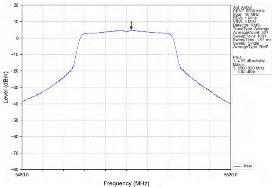
802.11ac(VHT20)_LCH_5500MHz_Ant22_NTNV
