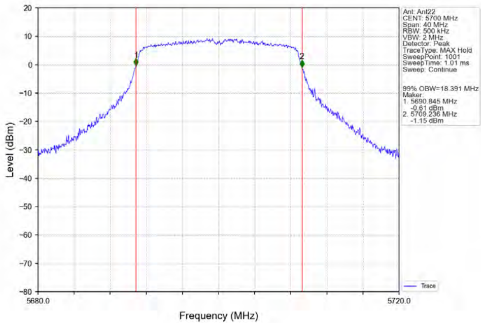
802.11ac(VHT20)_HCH_5700MHz_Ant22_NTNV
