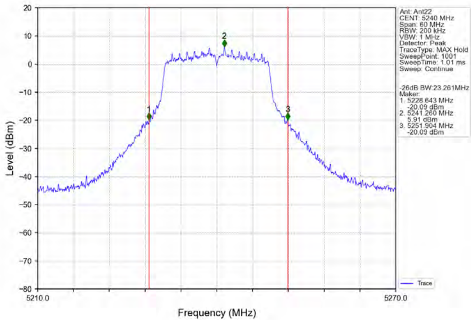
802.11n(HT20)_HCH_5240MHz_Ant22_NTNV
