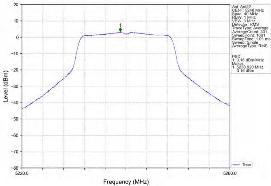
802.11n(HT20)_HCH_5240MHz_Ant22_NTNV
