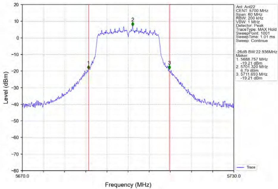
802.11n(HT20)_HCH_5700MHz_Ant22_NTNV
