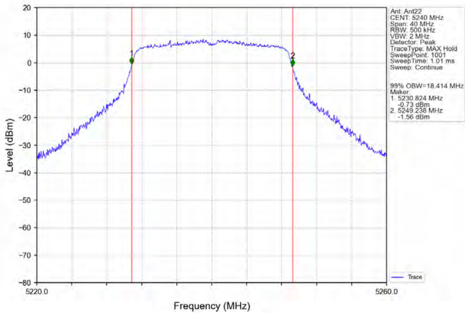
802.11ac(VHT20)_HCH_5240MHz_Ant22_NTNV
