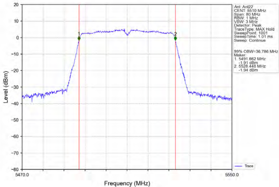
802.11ac(VHT40)_LCH_5510MHz_Ant22_NTNV
