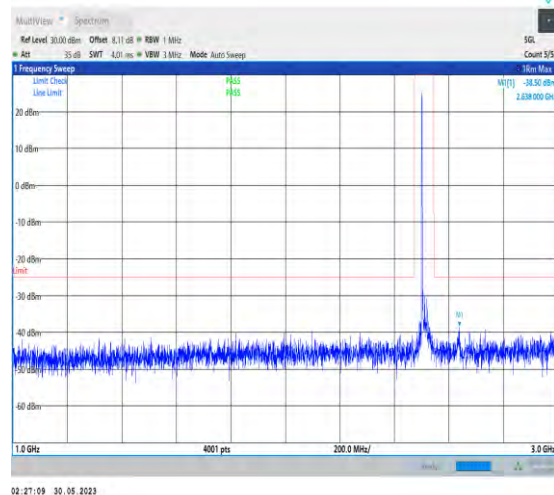
1-N7-PC3-15-20-L-1-N/A-DFT-PI2BPSK-Inner_1RB_ Left-1@1-1000-3000-Ant1-2380.50--38.50--25-PASS
