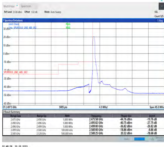
1-N7-PC3-15-5-L-4-CP-QPSK-Edge_1RB_Left-1@0-Ant1-1--PASS-see graph
