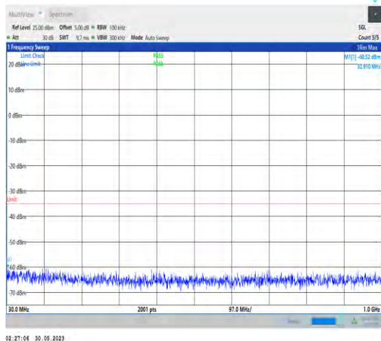
1-N7-PC3-15-20-L-1-N/A-DFT-PI2BPSK-Inner_1RB _Left-1@1-30-1000-Ant1-723.55--60.52--35-PASS
