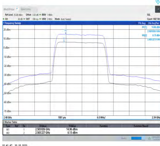
1-N7-PC3-15-20-L-1-DFT-256QAM-Outer_Full-100@ 0-Ant1-8.83-100%-0.00-8.83-PASS-≤13
