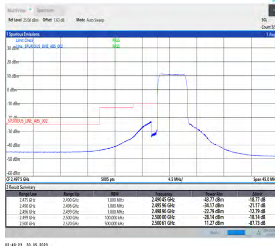
1-N7-PC3-15-5-L-6-CP-QPSK-Outer_Full-25@0-Ant1-1--PASS-see graph
