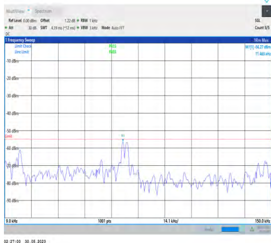
1-N7-PC3-15-20-L-1-N/A-DFT-PI2BPSK-Inner_1RB _Left-1@1-0.009-0.15-Ant1-0.02--56.27--55-PASS
