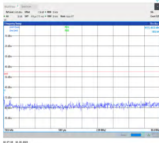
1-N7-PC3-15-20-L-1-N/A-DFT-PI2BPSK-Inner_1RB_ Left-1@1-0.15-30-Ant1-0.15--66.52--45-PASS
