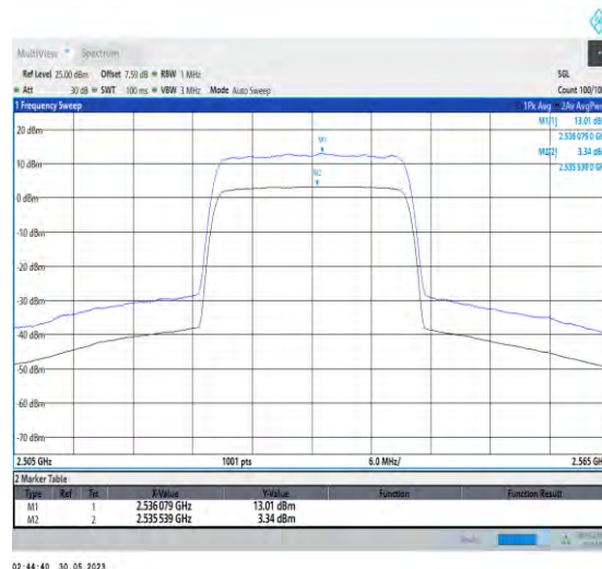
1-N7-PC3-15-20-M-2-CP-256QAM-Outer_Full-106 @0-Ant1-9.67-100%-0.00-9.67-PASS-≤13
