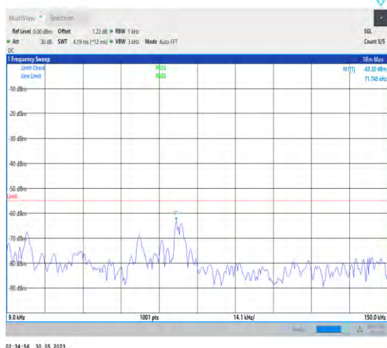
1-N7-PC3-15-20-M-1-N/A-DFT-PI2BPSK-Inner_1RB _Left-1@1-0.009-0.15-Ant1-0.01--63.20--55-PASS
