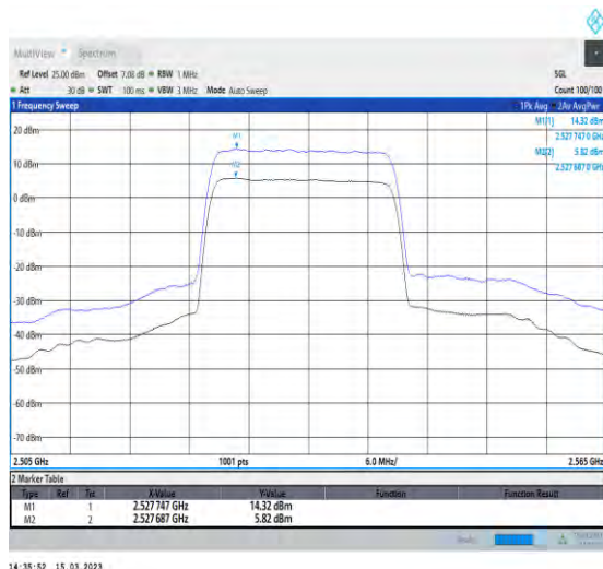
1-N7-PC3-15-20-M-1-DFT-256QAM-Outer_Full-100 @0-Ant1-8.50-100%-0.00-8.50-PASS-≤13
