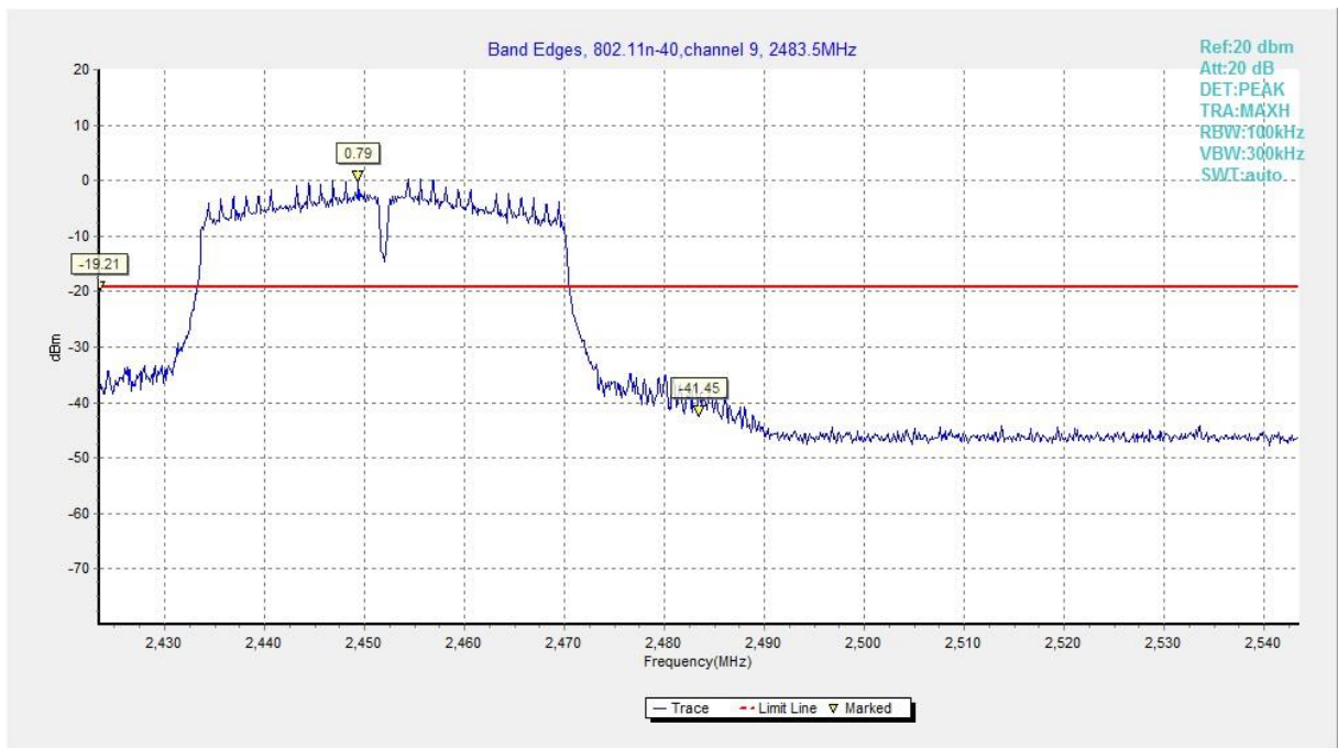
Fig.A.5.1.8 Band Edges (802.11n-HT40, Ch 9)
