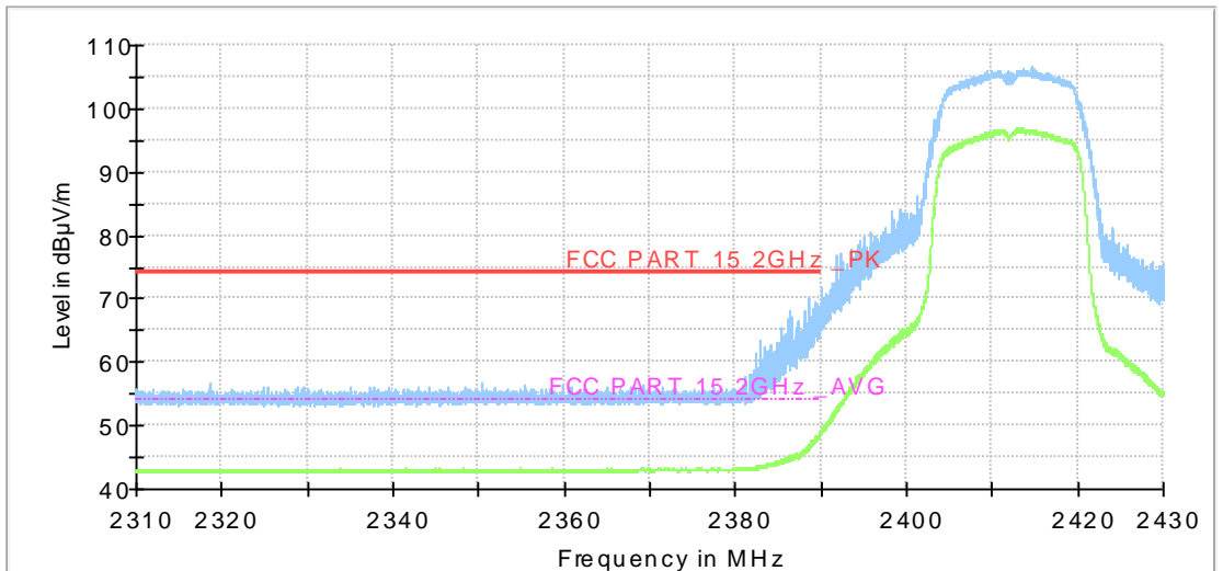
Full Spectrum
