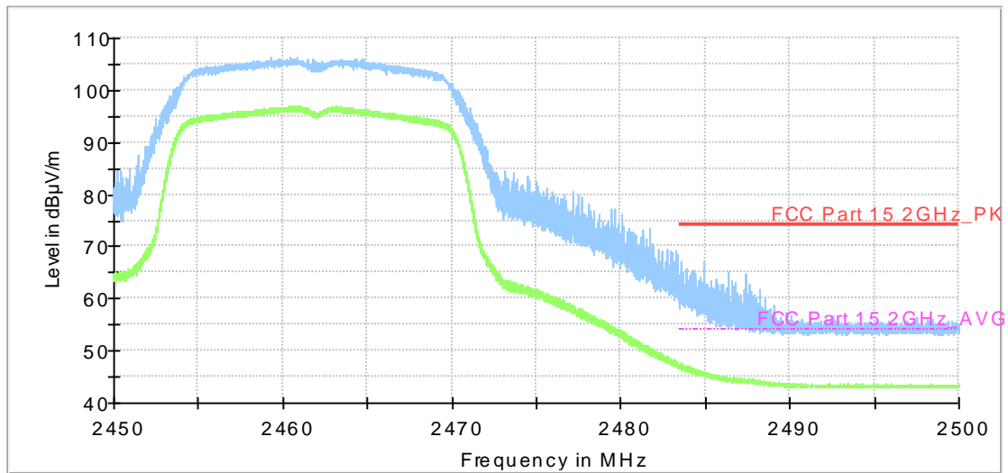
Full Spectrum
