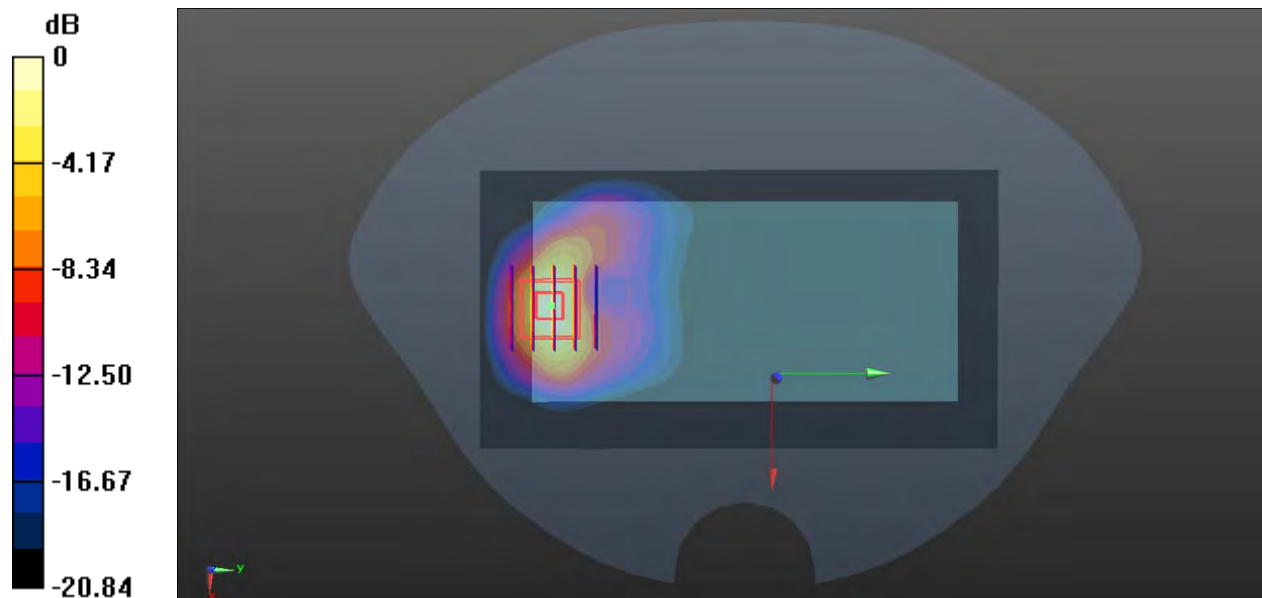
0 dB = 4.52 W/kg
