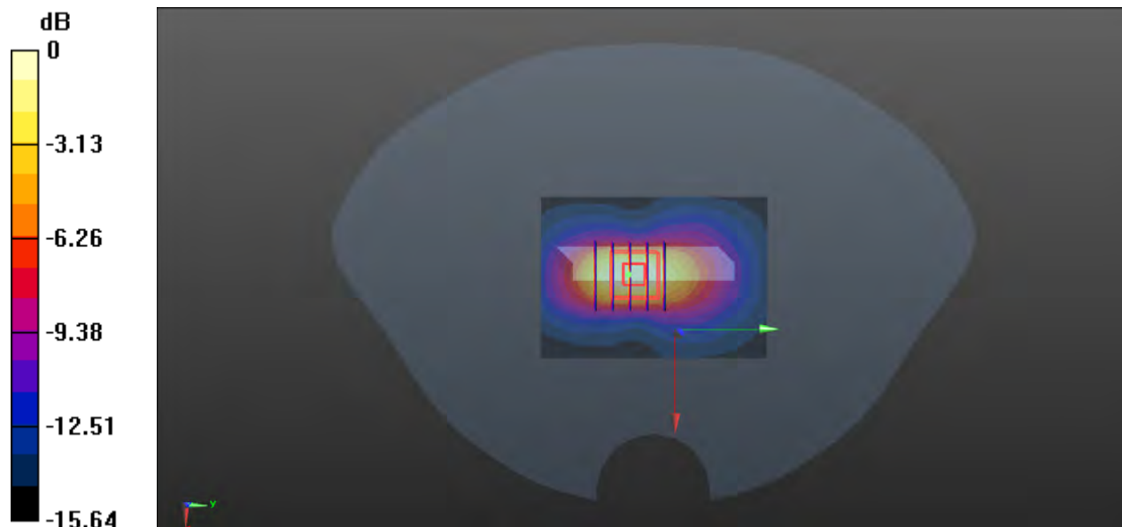
0 dB = 0.500 W/kg
