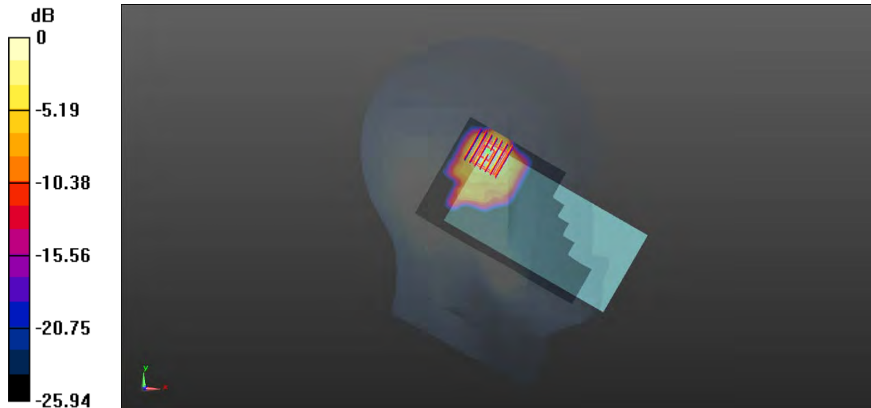
0 dB = 0.0760 W/kg
