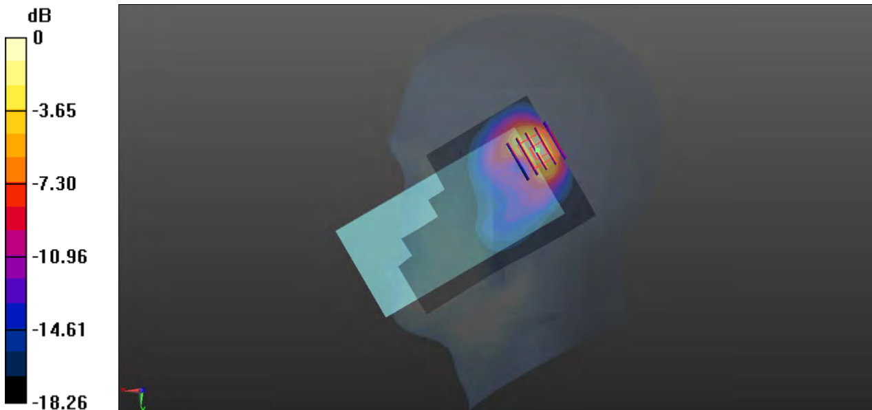
0 dB = 0.758 W/kg
