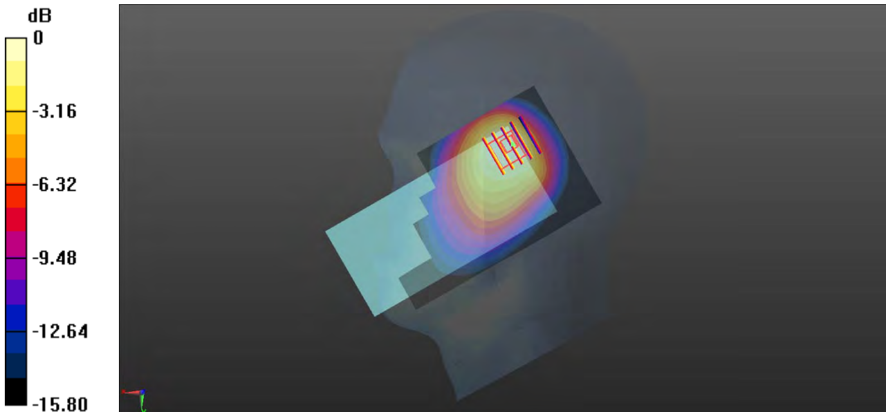
0 dB = 0.601 W/kg
