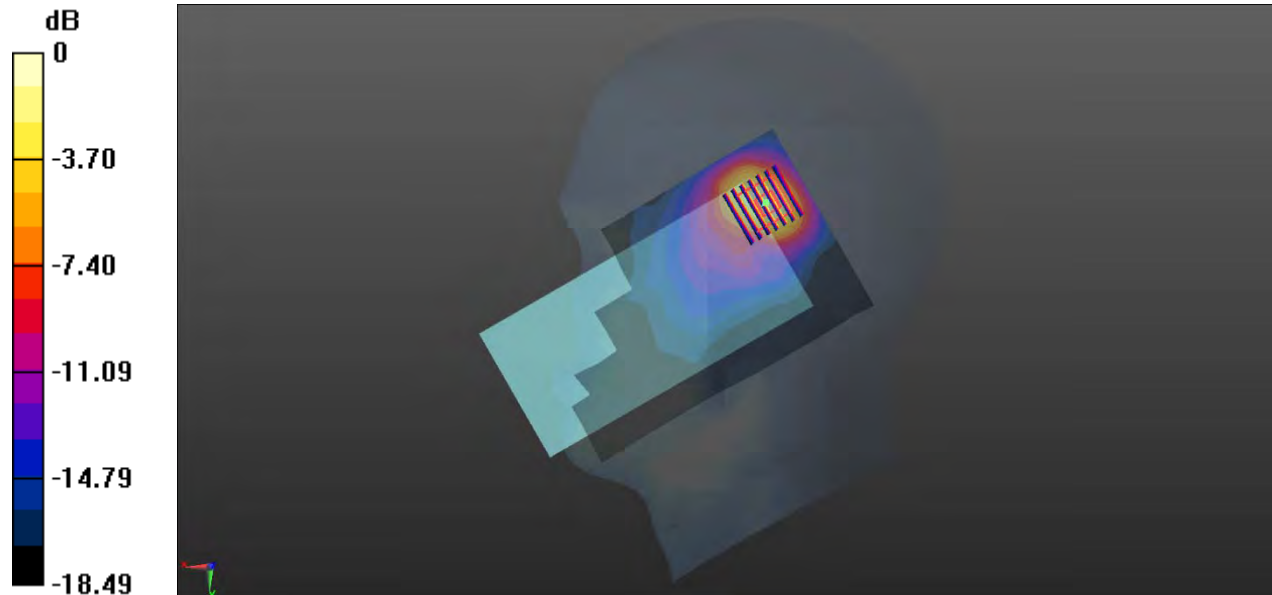
0 dB = 0.643 W/kg
