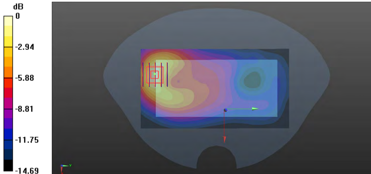
0 dB = 0.323 W/kg
