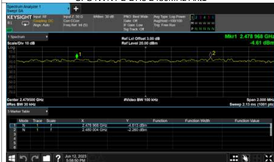
CFS NVNT 2-DH5 2480MHz Ant1
