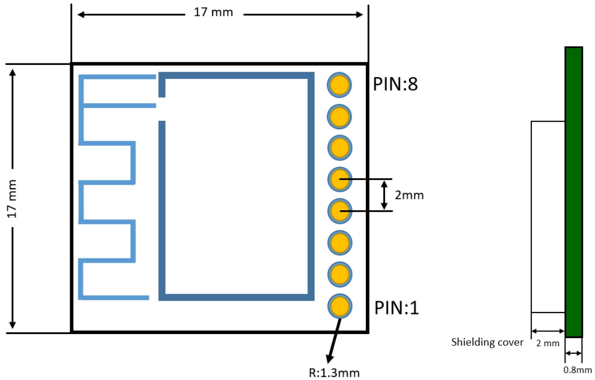
Figure 6-1 PCBA size
