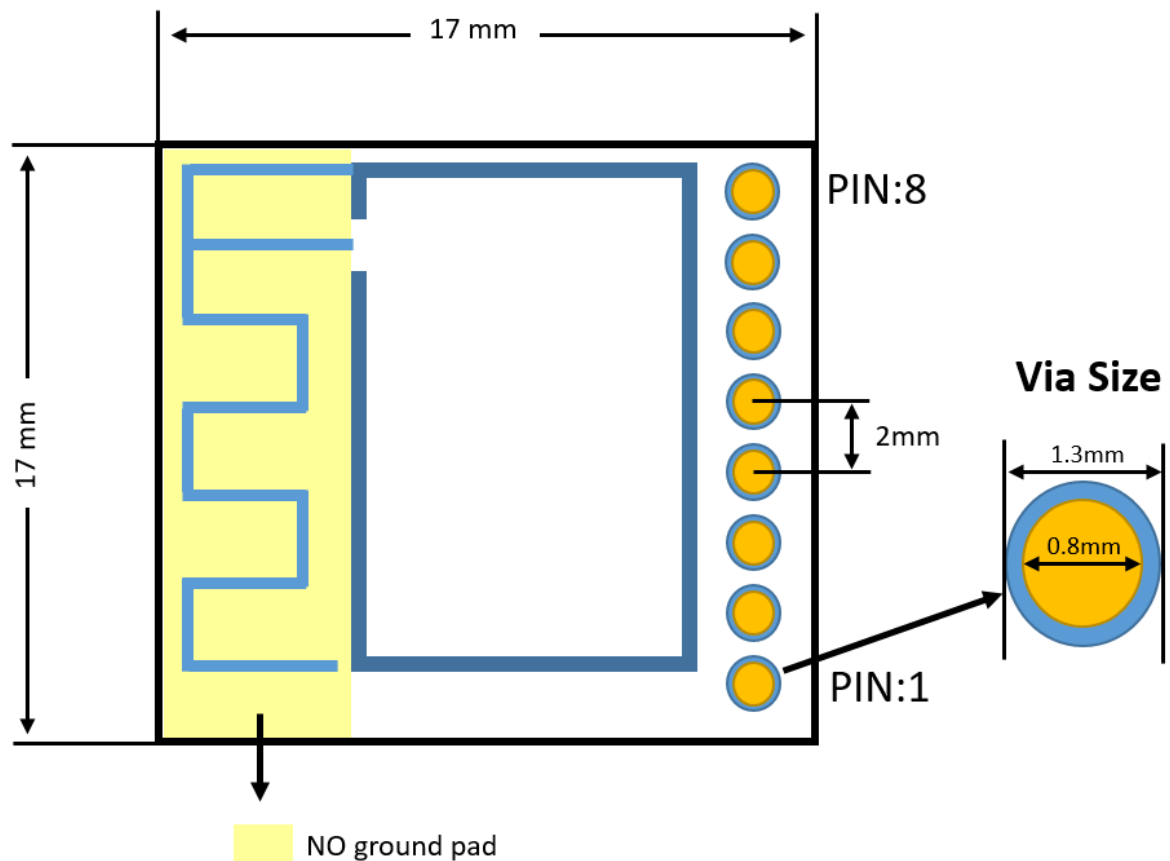
Figure 7-1 Solder pad layout reference
