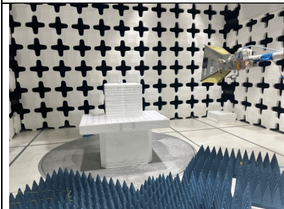
Radiated Emission Test 1-18GHz Front View
