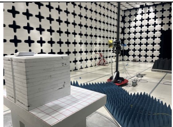
Radiated Emission Test 1-18GHz Rear View
