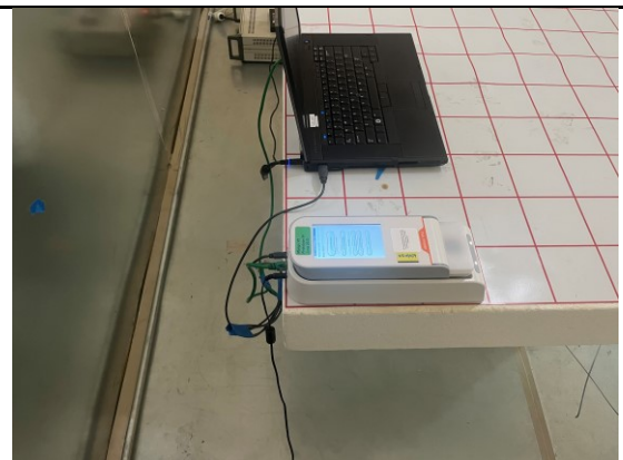
Conducted Emission Test Side View
