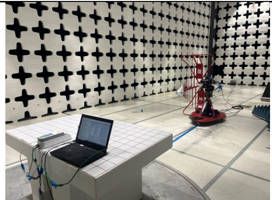
Radiated Emission Test below 1GHz Rear View
