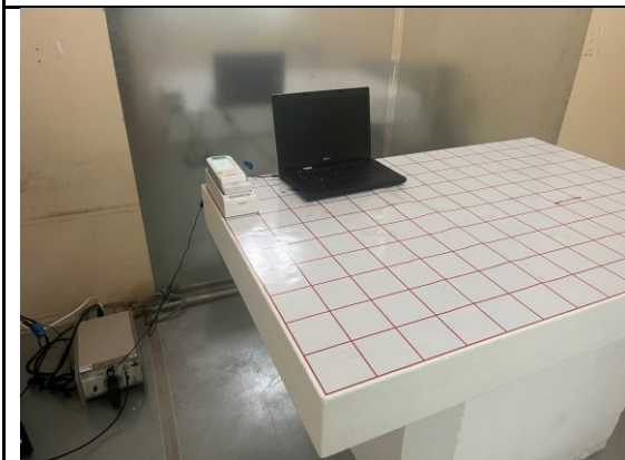
Conducted Emission Test Front View
