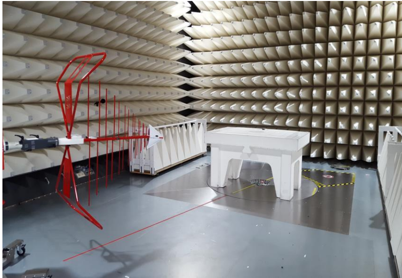
Figure B3. Radiated measurement setup Low range
