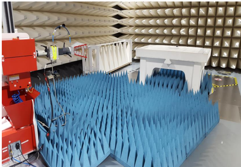
Figure B4. Radiated measurement setup High Range
