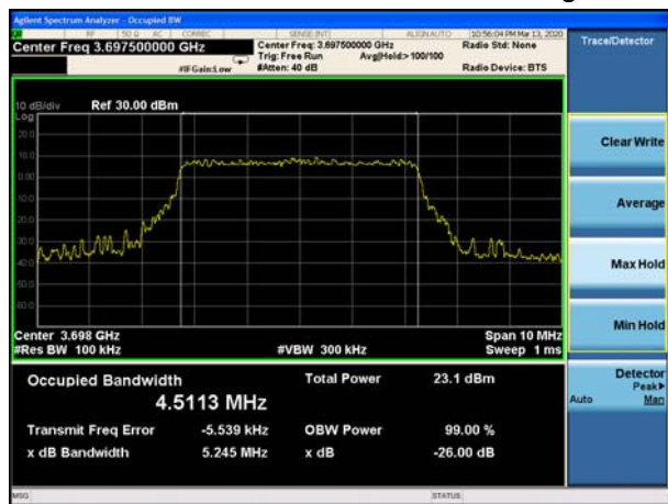
LTE Band 48 5MHz 16QAM CH-High
