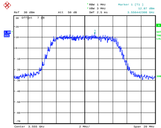
LTE Band 48 10MHz QPSK CH-Low
