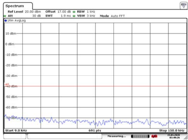
LTE Band 48 5MHz CH- Middle 9kHz~150kHz
