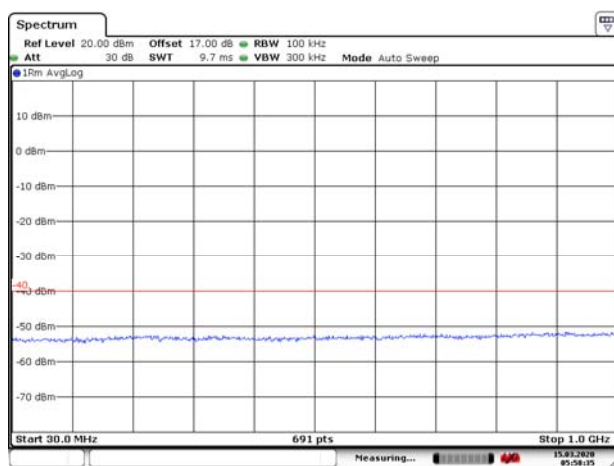
LTE Band 48 5MHz CH-Low 30MHz~1GHz
