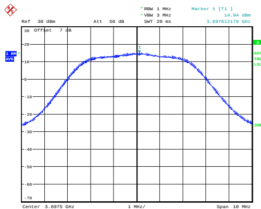
LTE Band 48 5MHz QPSK CH-High
