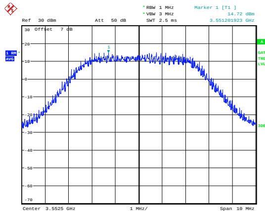
LTE Band 48 5MHz QPSK CH-Low
