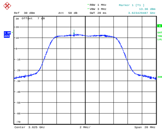
LTE Band 48 10MHz QPSK CH-Middle
