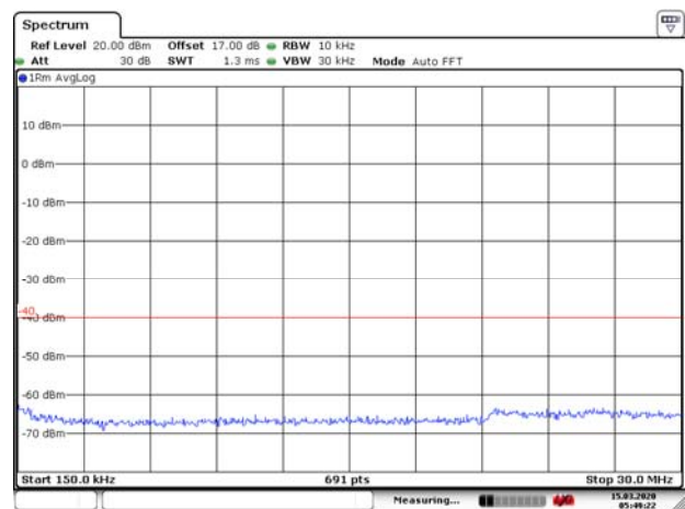
LTE Band 48 5MHz CH- Middle 150kHz~30MHz
