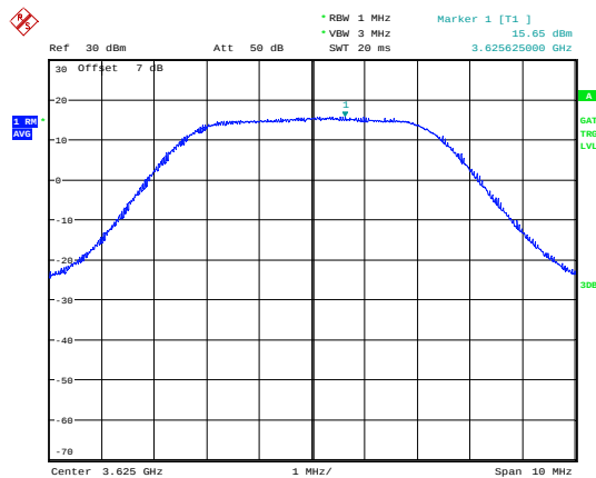
LTE Band 48 5MHz QPSK CH-Middle
