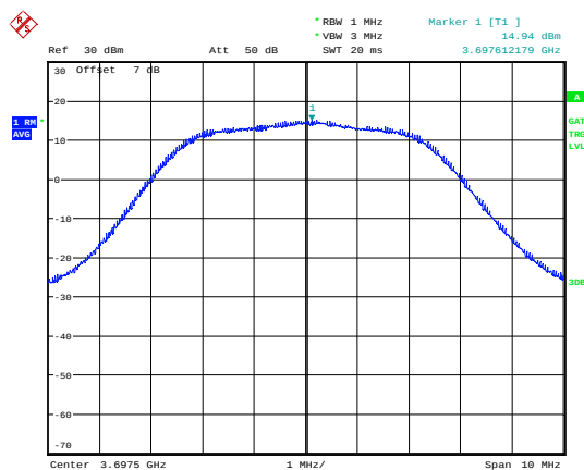
LTE Band 48 5MHz QPSK CH-High
