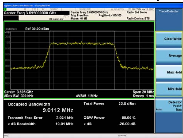
LTE Band 48 10MHz 16QAM CH-High
