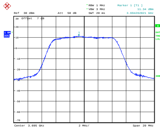
LTE Band 48 10MHz QPSK CH-High
