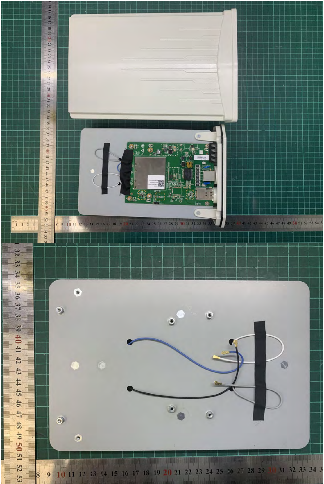
internal photo
