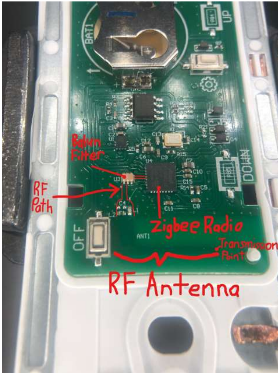
Legrand WNRL23 Zigbee Antenna View
