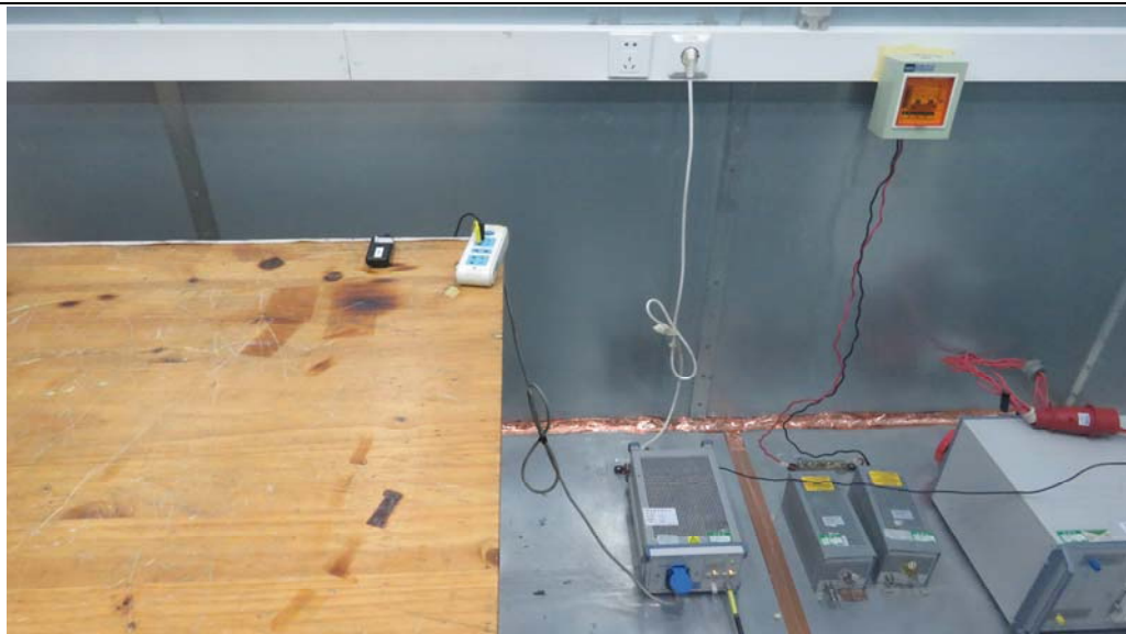
Picture 2: Conducted Emissions Test Setup
