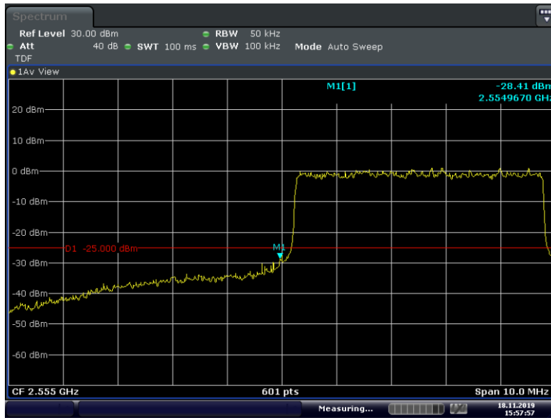
Band41-5MHz-QPSK-40265-25RB#0
