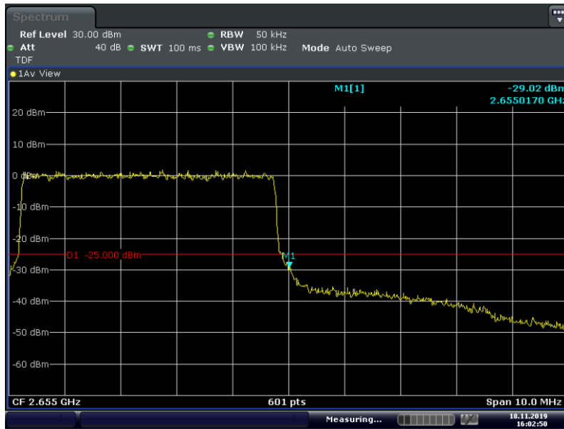
Band41-5MHz-QPSK-41215-25RB#0
