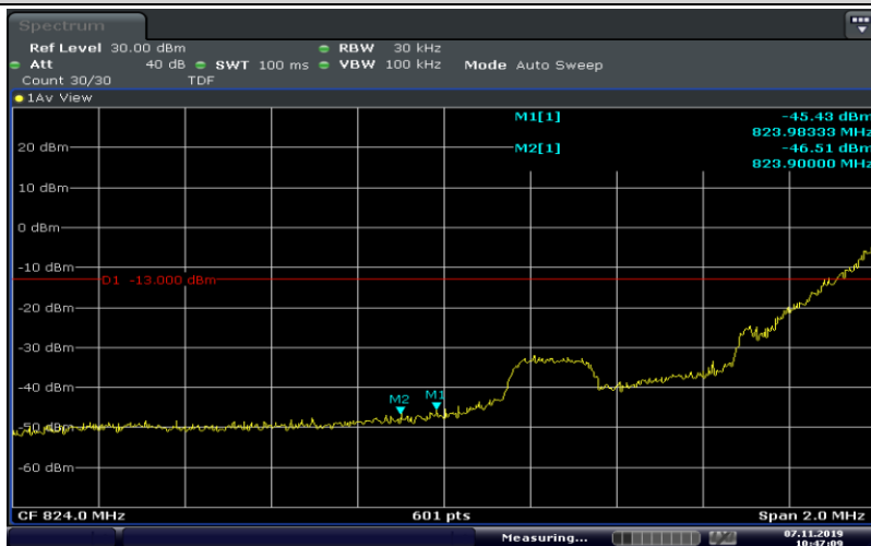
Band26-1.4MHz-16QAM-26797-1RB#5
