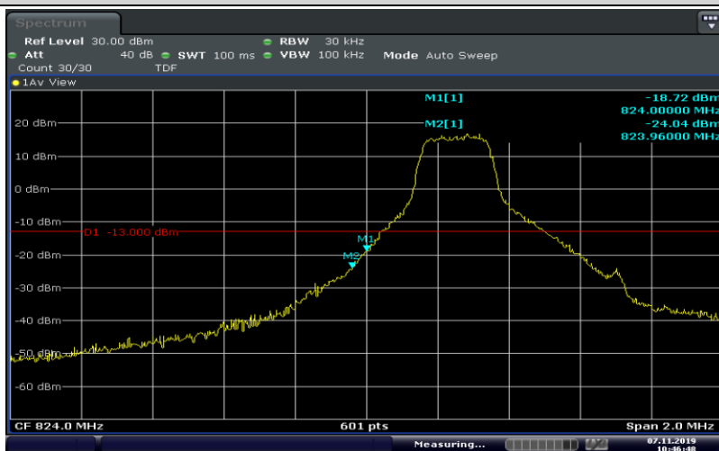
Band26-1.4MHz-16QAM-26797-1RB#0
