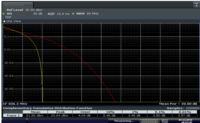
Band26-1.4MHz-QPSK-26915-6RB#0
