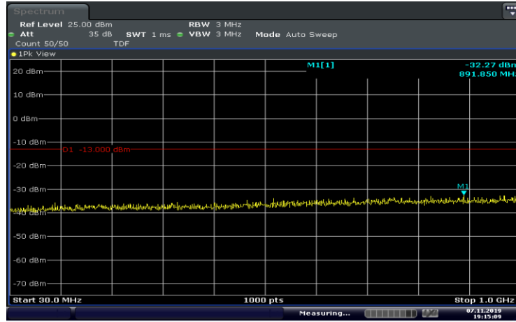
Band2-1.4MHz-QPSK-18607-6RB#0-Range1:30~1000MHz
