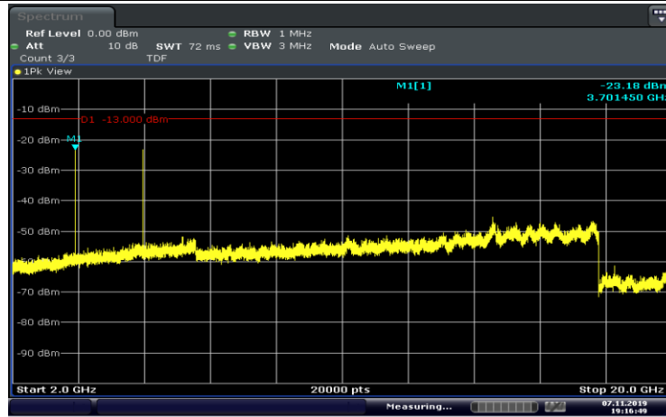
Band2-1.4MHz-QPSK-18607-6RB#0-Range3:2000~20000MHz
