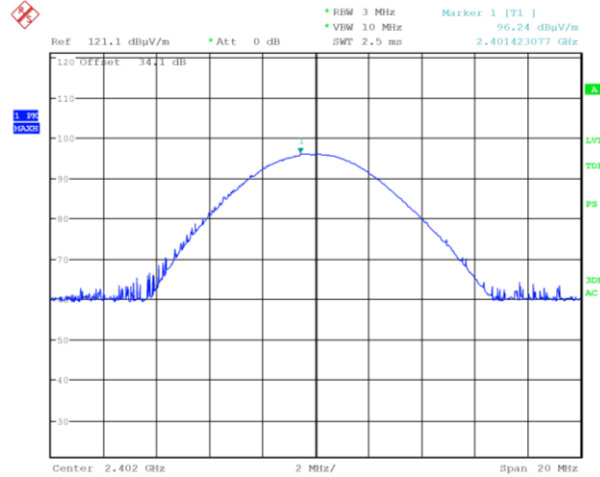
Low channel, vertical polarization
