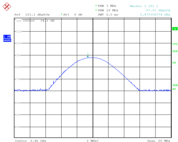
High channel horizontal polarization
