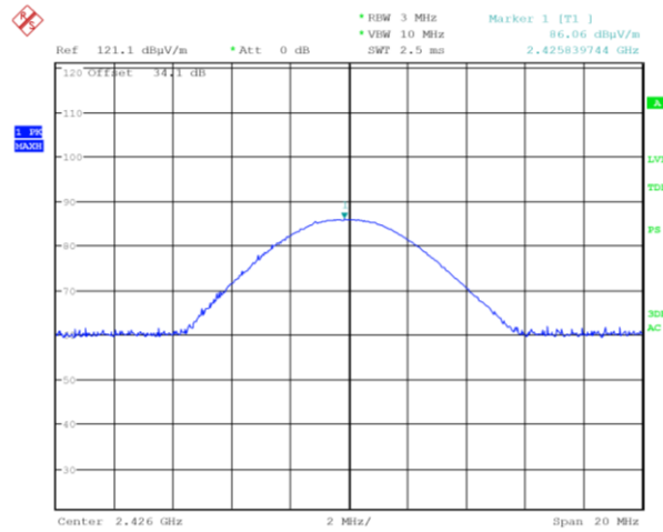
Middle channel, horizontal polarization
