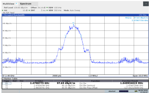
BLE: 99% bandwidth on high channel
