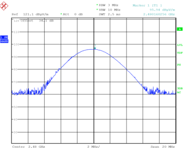
High channel vertical polarization
