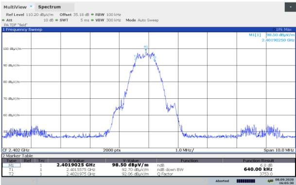
BLE: 6 dB bandwidth on low channel
