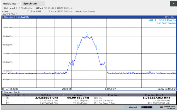
BLE: 99% bandwidth on middle channel
