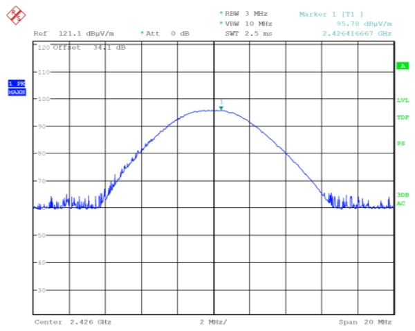
Middle channel, vertical polarization
