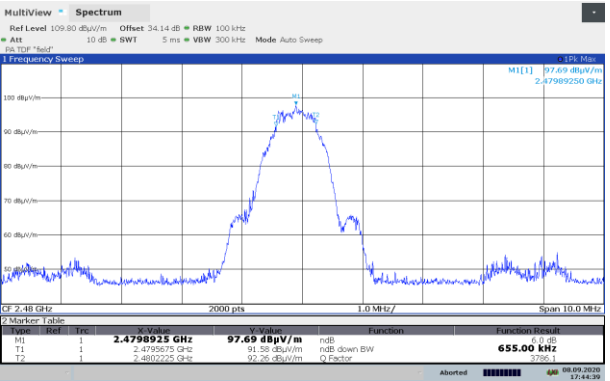
BLE: 6 dB bandwidth on high channel
