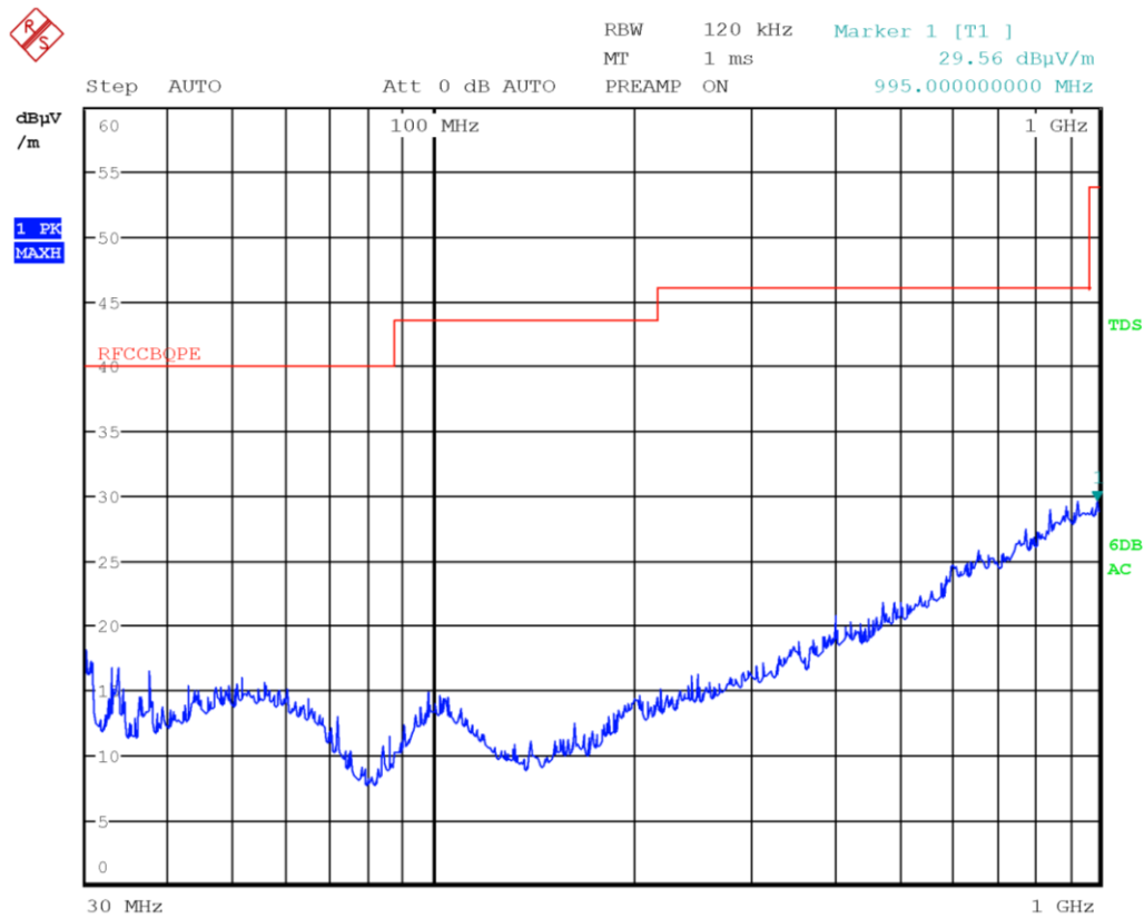
Radiated measurement BT vertical polarization, low channel
