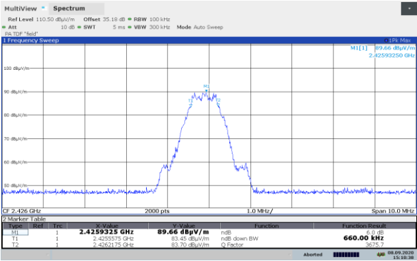
BLE: 6 dB bandwidth on middle channel
