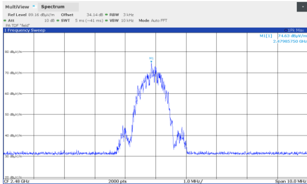
High channel, horizontal polarization
