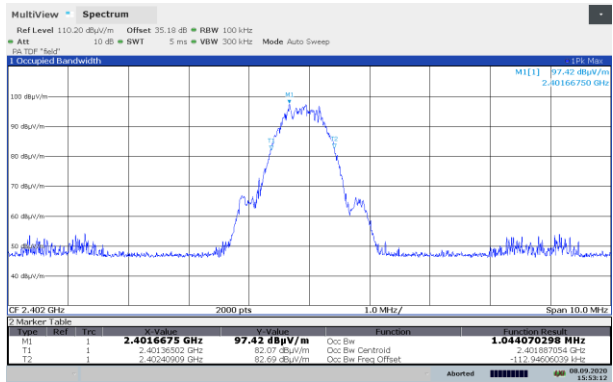
BLE: 99% bandwidth on low channel
