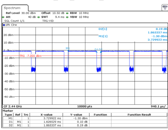
BLE_1M_Middle_Channel
