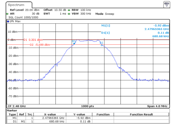
BLE_1M_High_Channel
