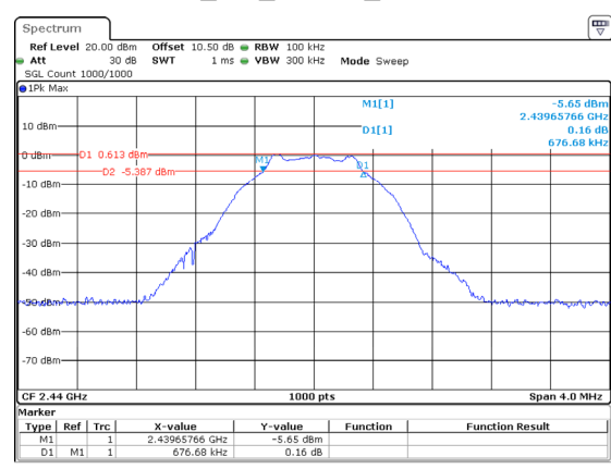
BLE_1M_Middle_Channel
