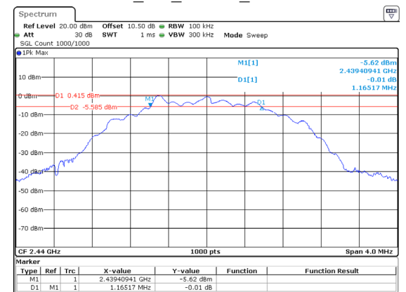
BLE_2M_Middle_Channel
