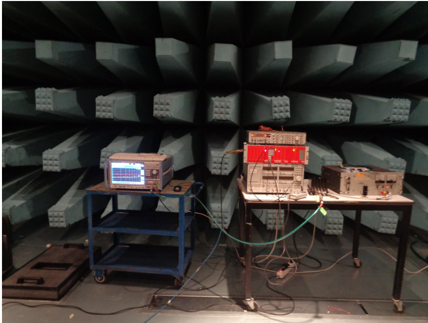
Set-up photo for antenna port tests
