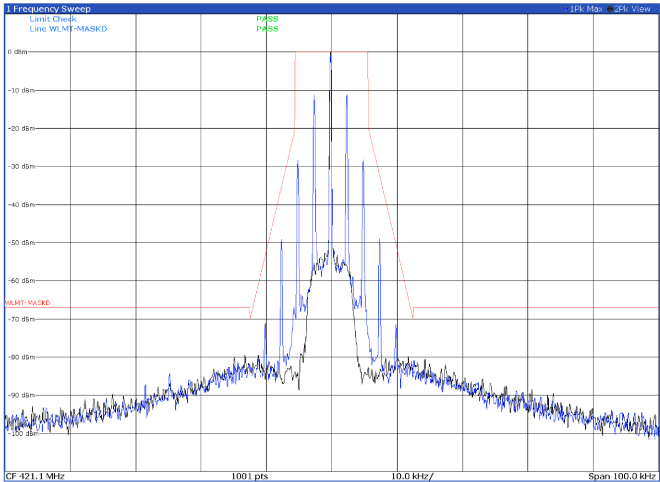
Emission mask D with modulation FM 12.5 kHz at 421.1 MHz
