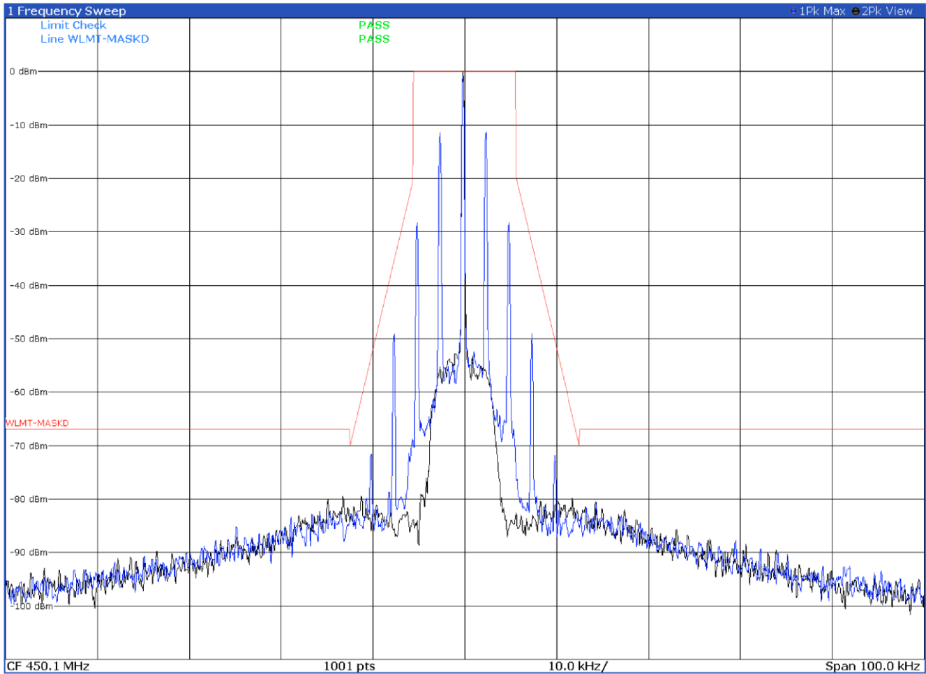
Emission mask D with modulation FM 12.5 kHz at 450.1 MHz
