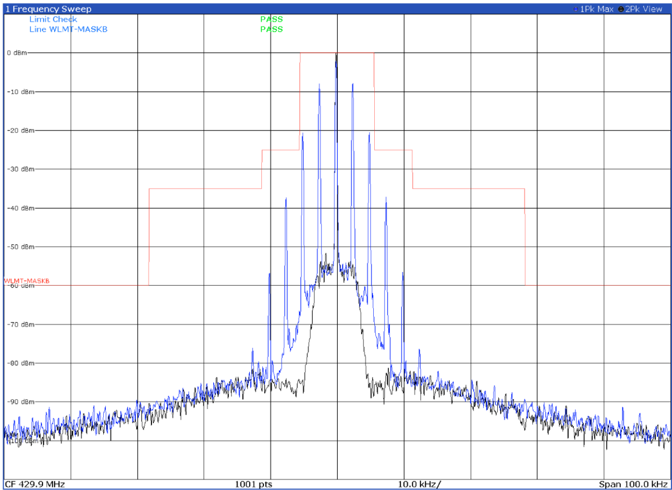
Emission mask B with modulation FM 25.0 kHz at 429.9 MHz
