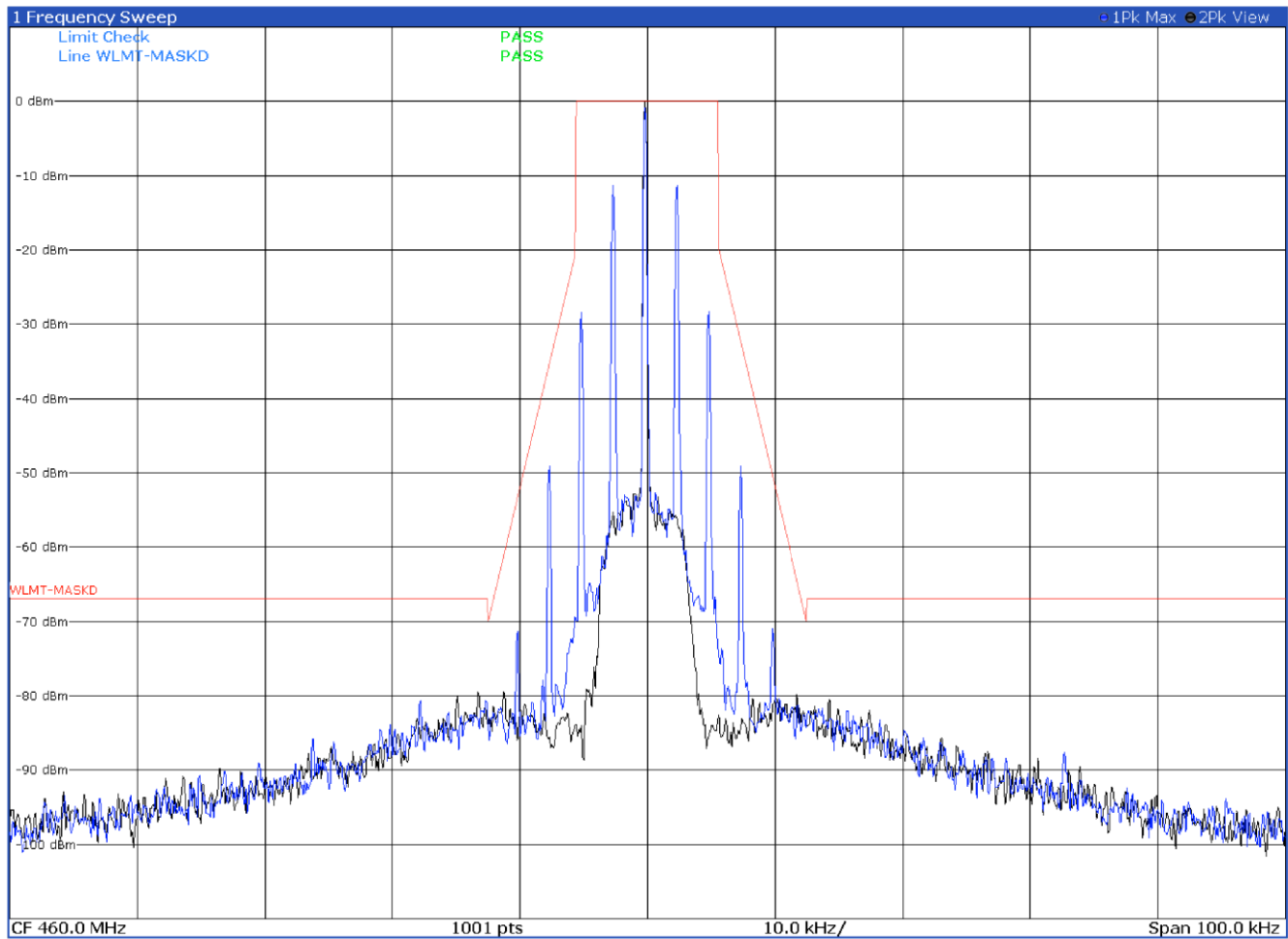
Emission mask D with modulation FM 12.5 kHz at 460.0 MHz
