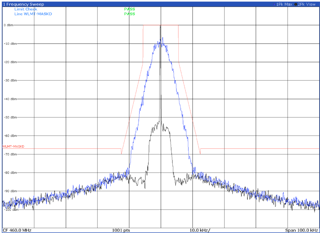
Emission mask D with modulation DMR 4FSK at 460.0 MHz
