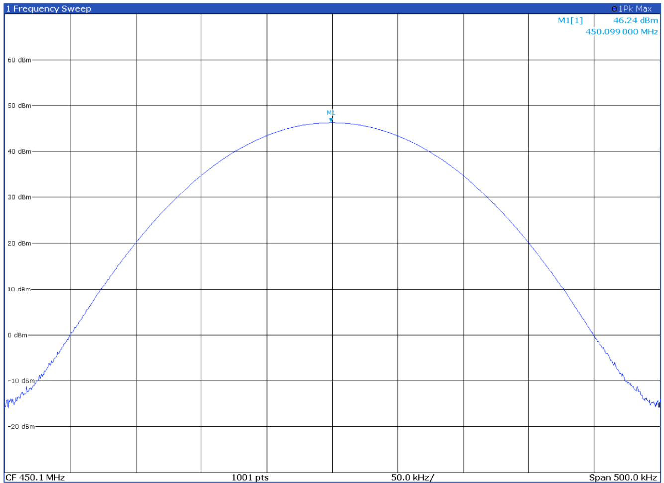
Output power with modulation P25 C4FM at 450.1 MHz
