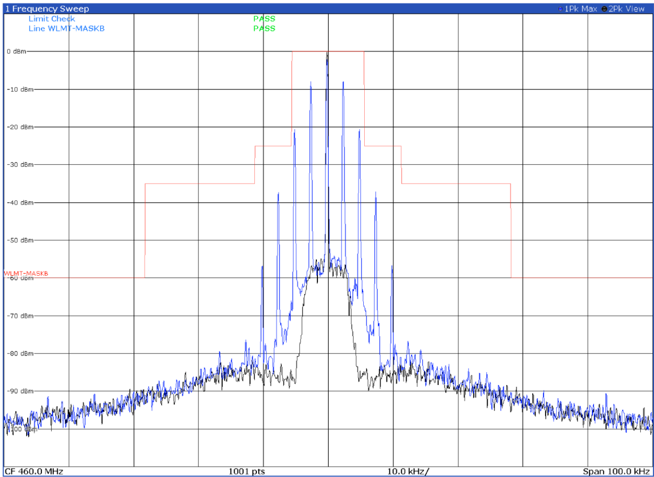
Emission mask B with modulation FM 25.0 kHz at 460.0 MHz
