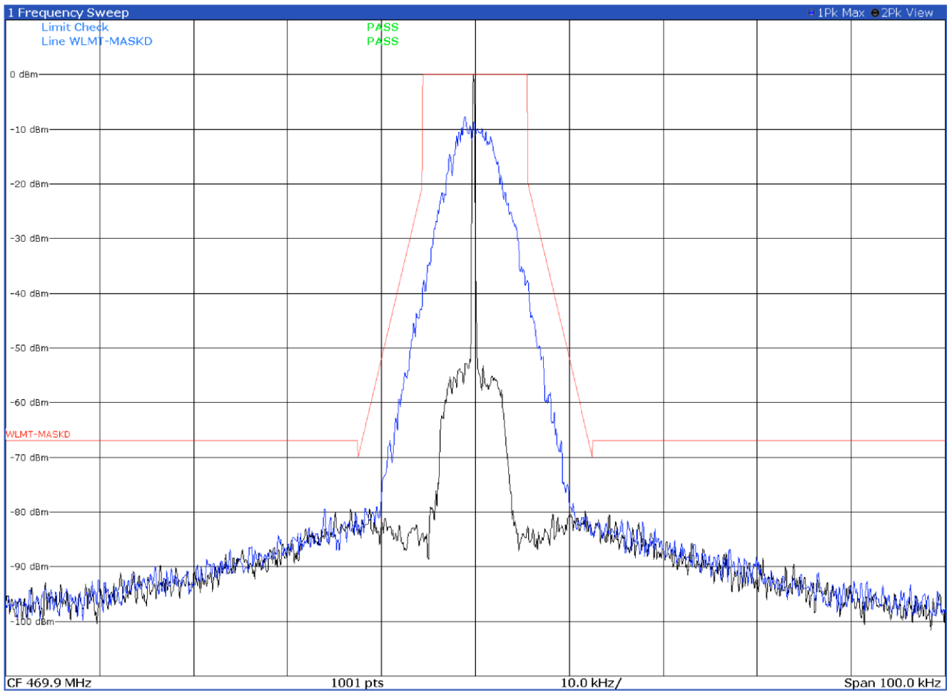
Emission mask D with modulation DMR 4FSK at 469.9 MHz
