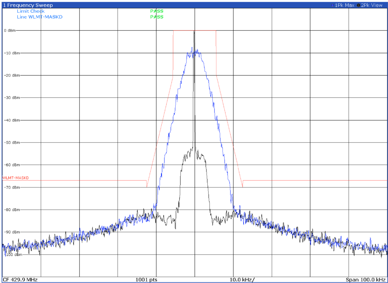
Emission mask D with modulation DMR 4FSK at 429.9 MHz
