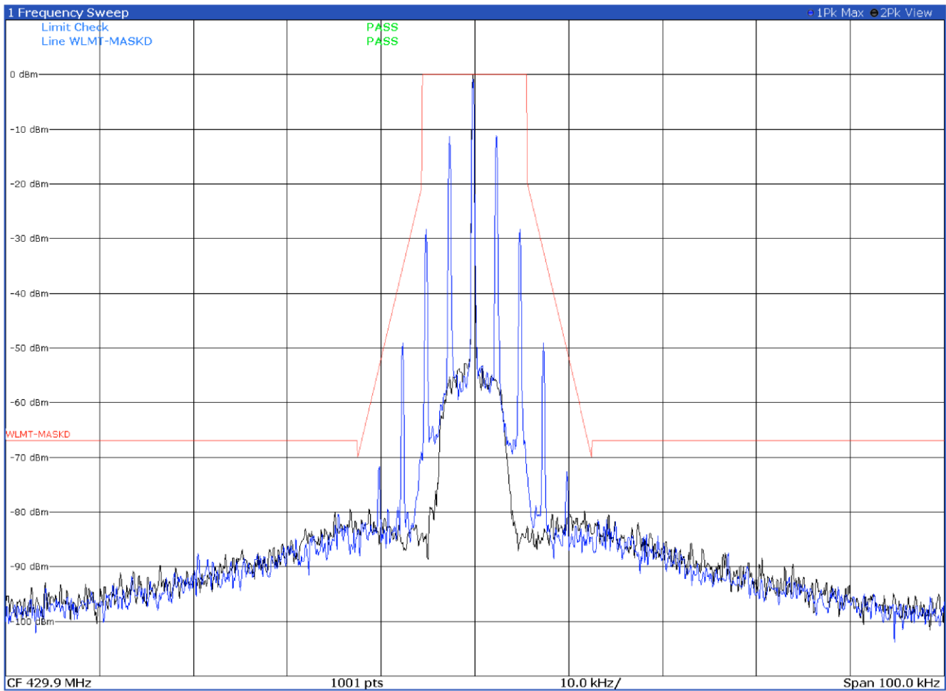
Emission mask D with modulation FM 12.5 kHz at 429.9 MHz
