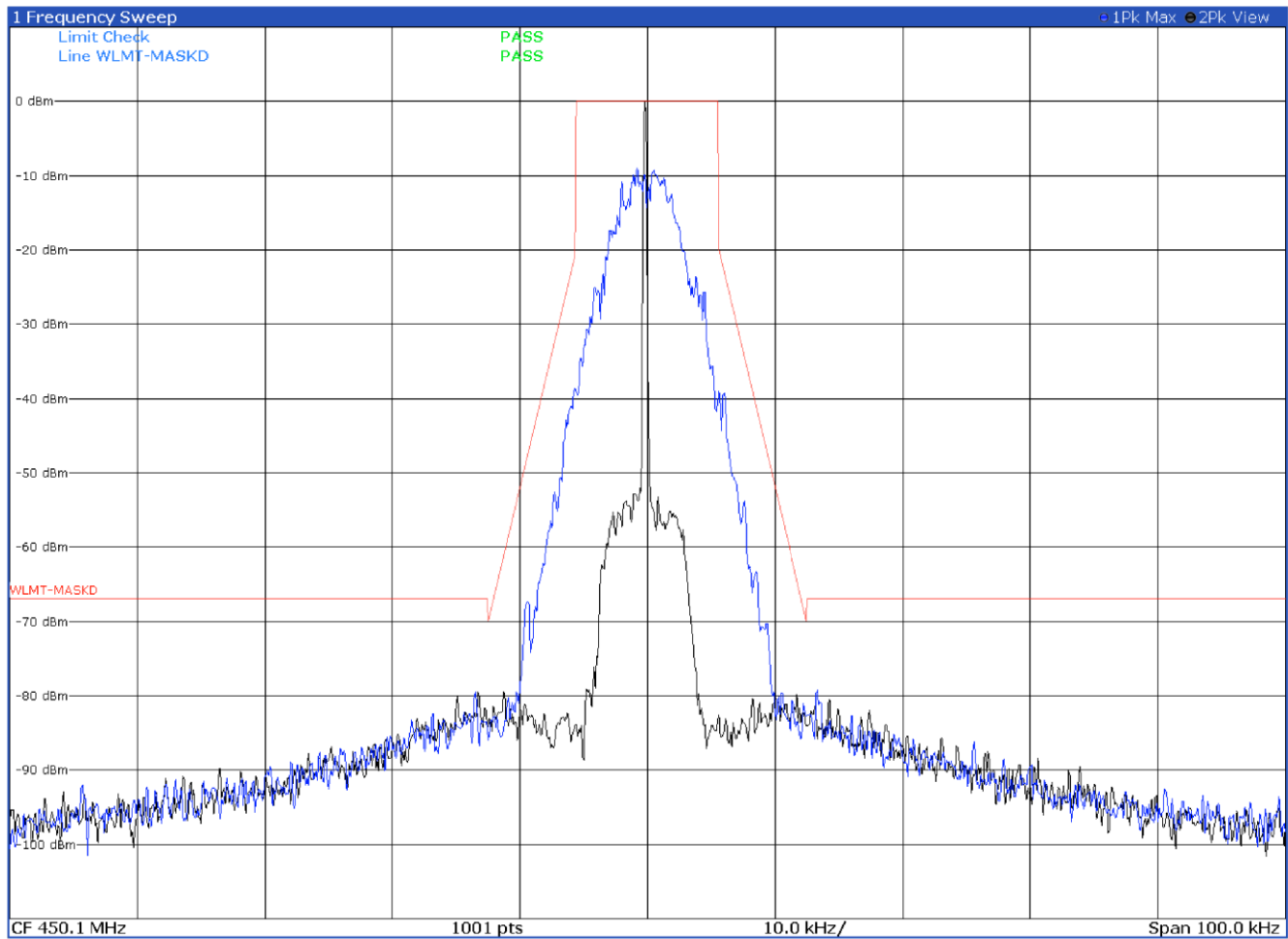
Emission mask D with modulation DMR 4FSK at 450.1 MHz
