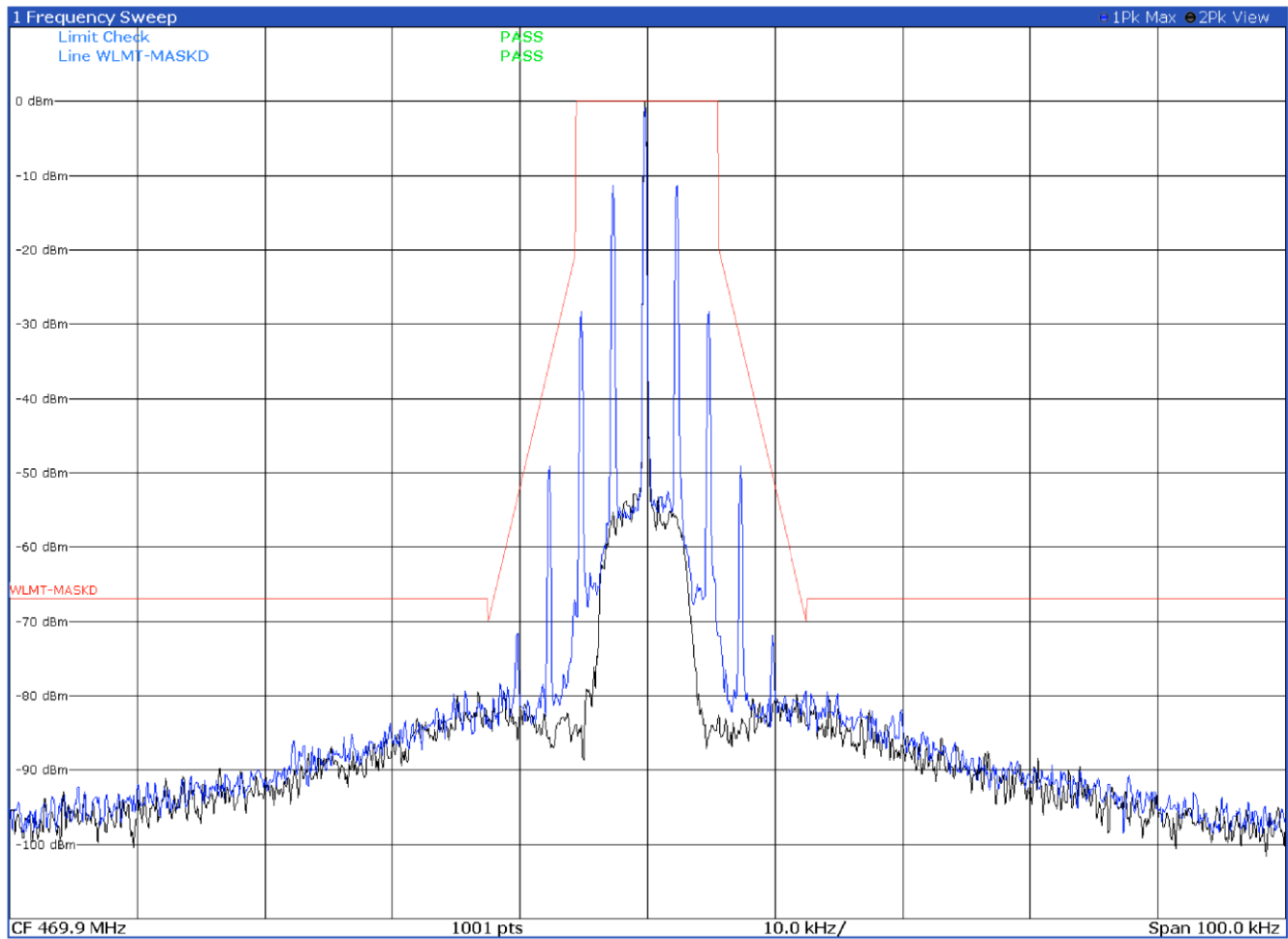
Emission mask D with modulation FM 12.5 kHz at 469.9 MHz
