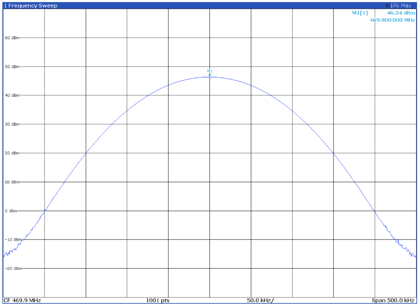
Output power with modulation CST 4FSK at 469.9 MHz
