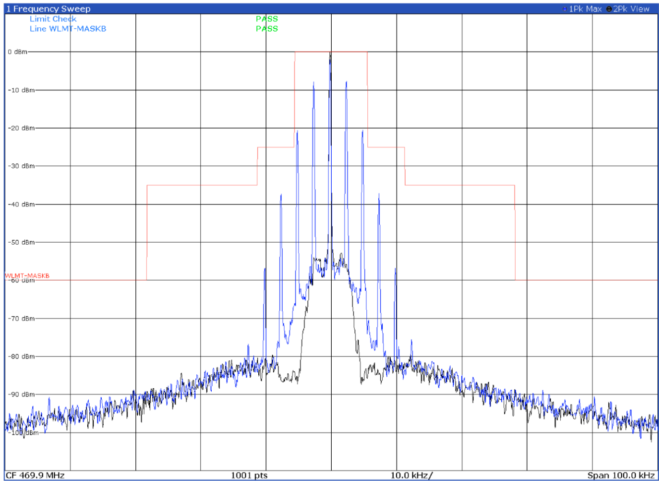
Emission mask B with modulation FM 25.0 kHz at 469.9 MHz
