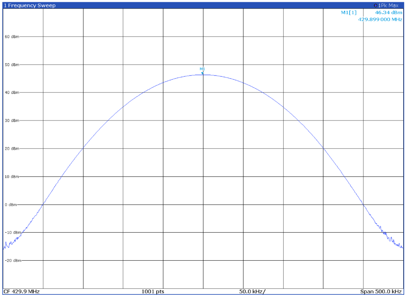
Output power with modulation P25 C4FM at 429.9 MHz
