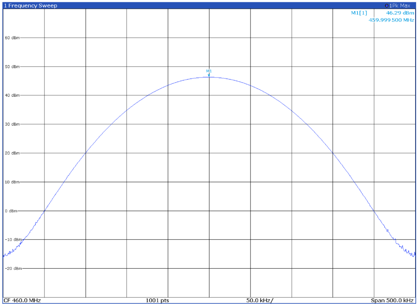
Output power with modulation DMR 4FSK at 460.0 MHz
