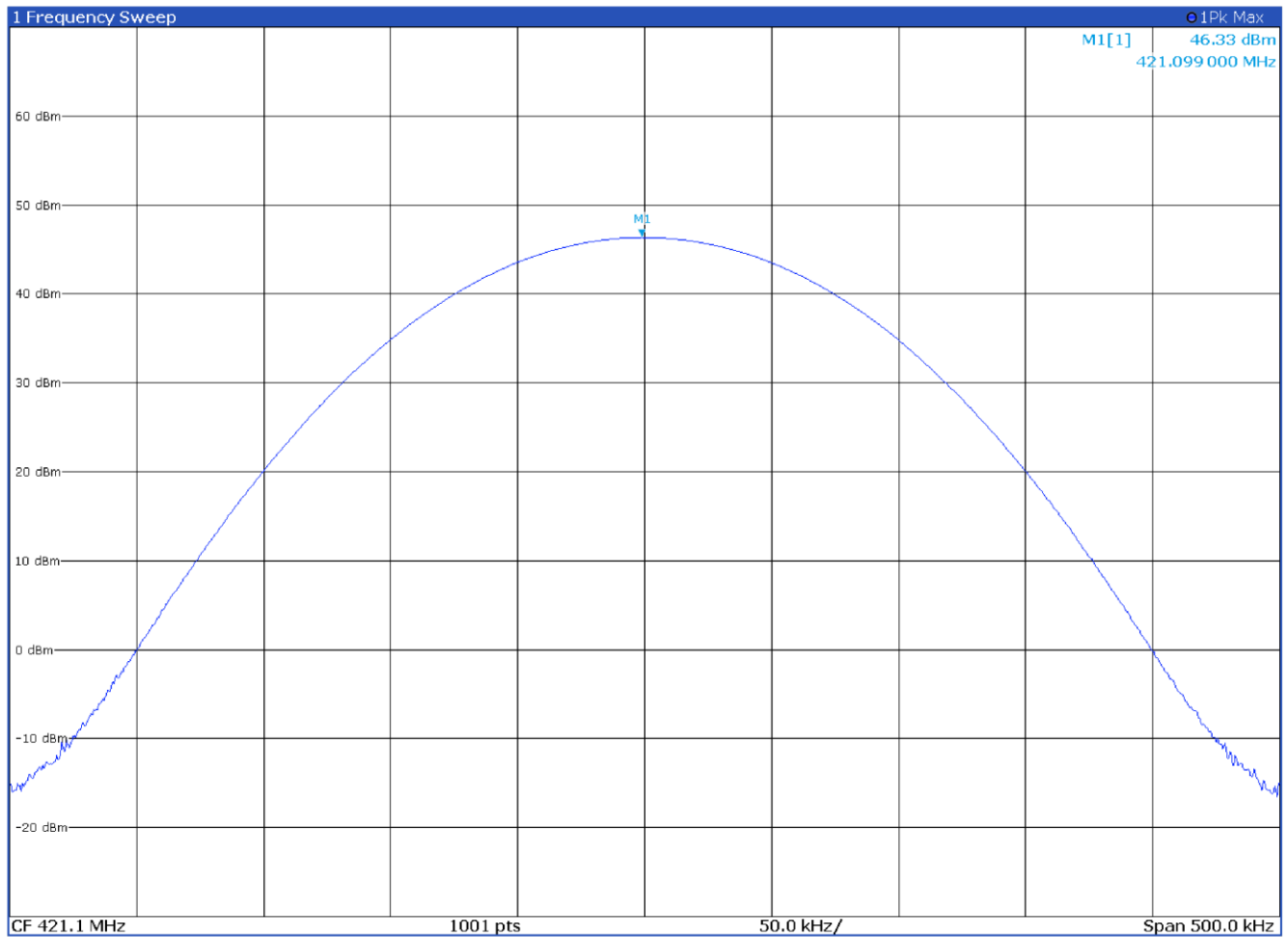
Output power with modulation DMR 4FSK at 421.1 MHz
