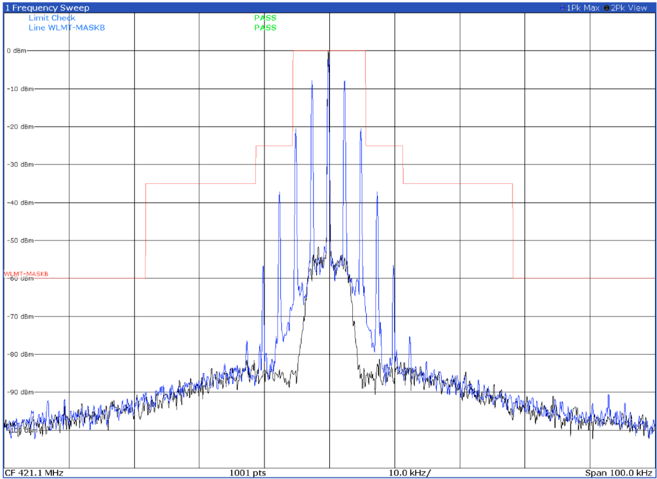
Emission mask B with modulation FM 25.0 kHz at 421.1 MHz
