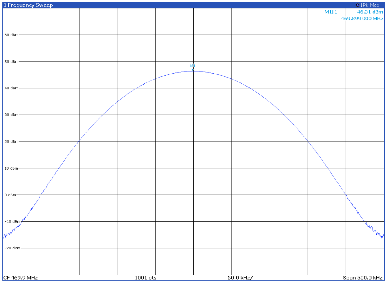
Output power with modulation P25 C4FM at 469.9 MHz
