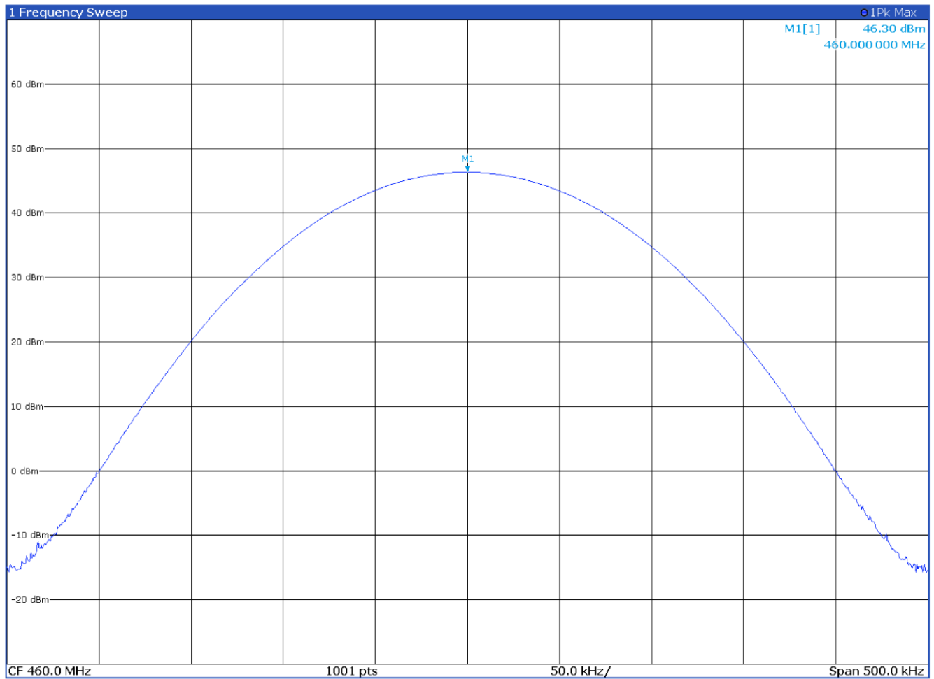
Output power with modulation P25 C4FM at 460.0 MHz
