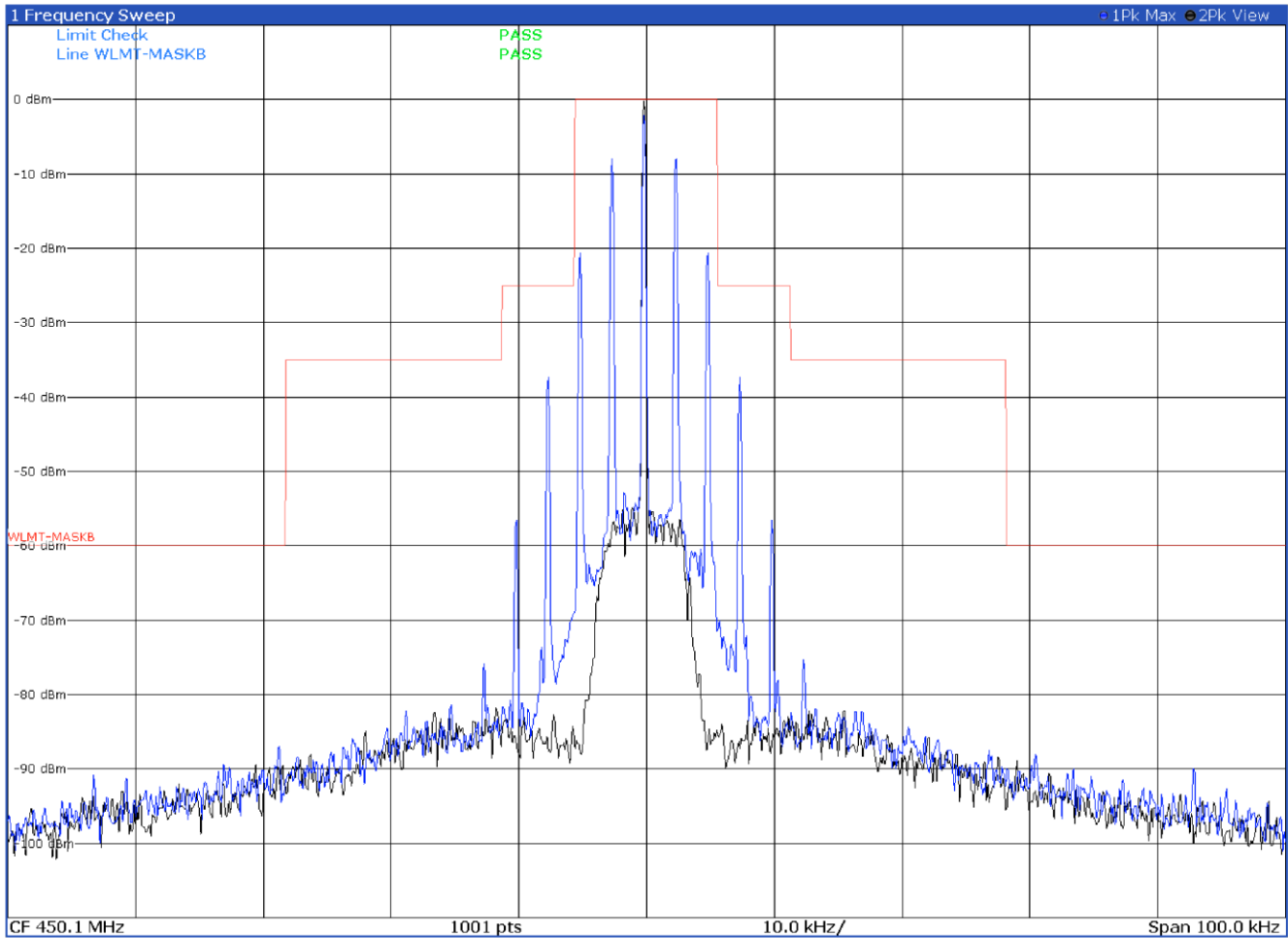
Emission mask B with modulation FM 25.0 kHz at 450.1 MHz
