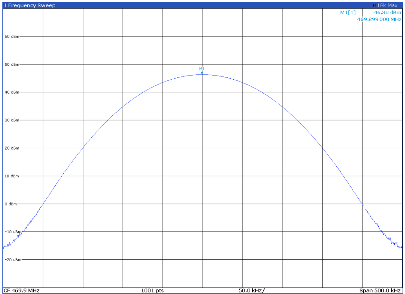
Output power with modulation DMR 4FSK at 469.9 MHz
