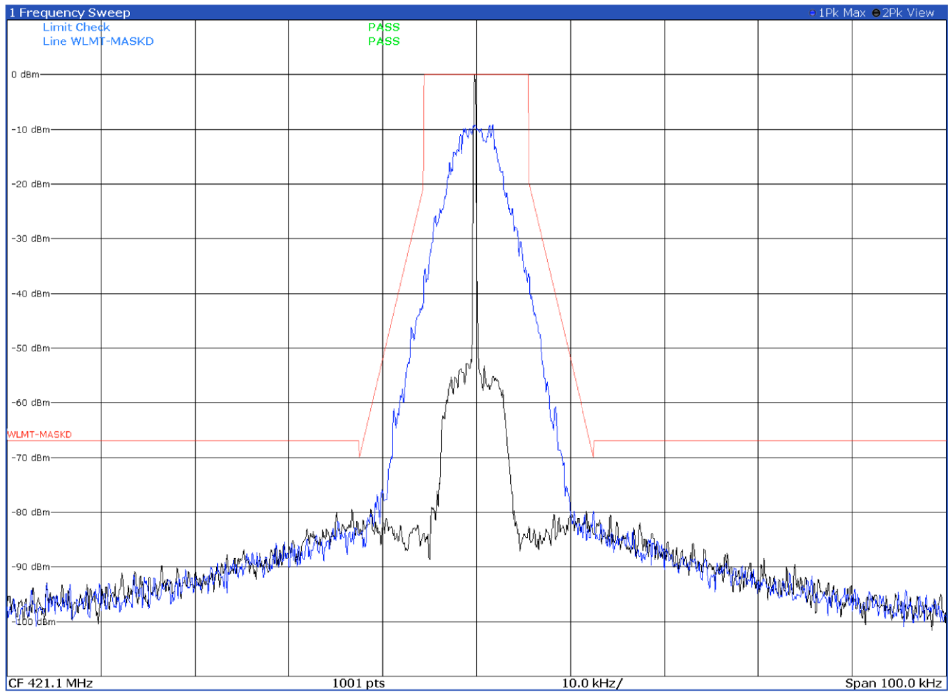
Emission mask D with modulation DMR 4FSK at 421.1 MHz
