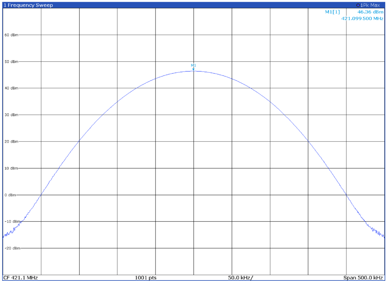
Output power with modulation P25 C4FM at 421.1 MHz
