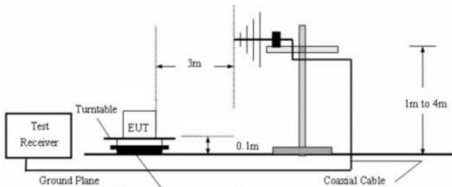
Figure 1. Below 30MHz
