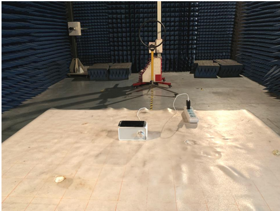
Radiated Emission (WPT)
