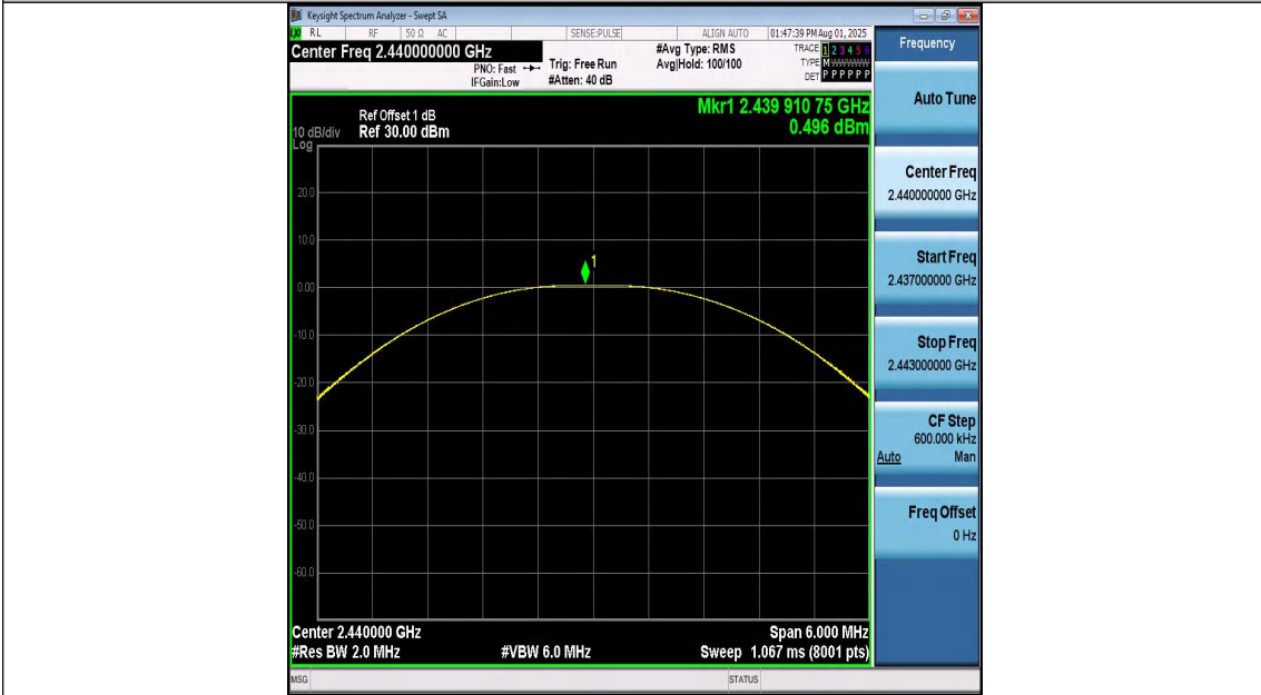
BLE_1M-Ant1-2440-PASS
