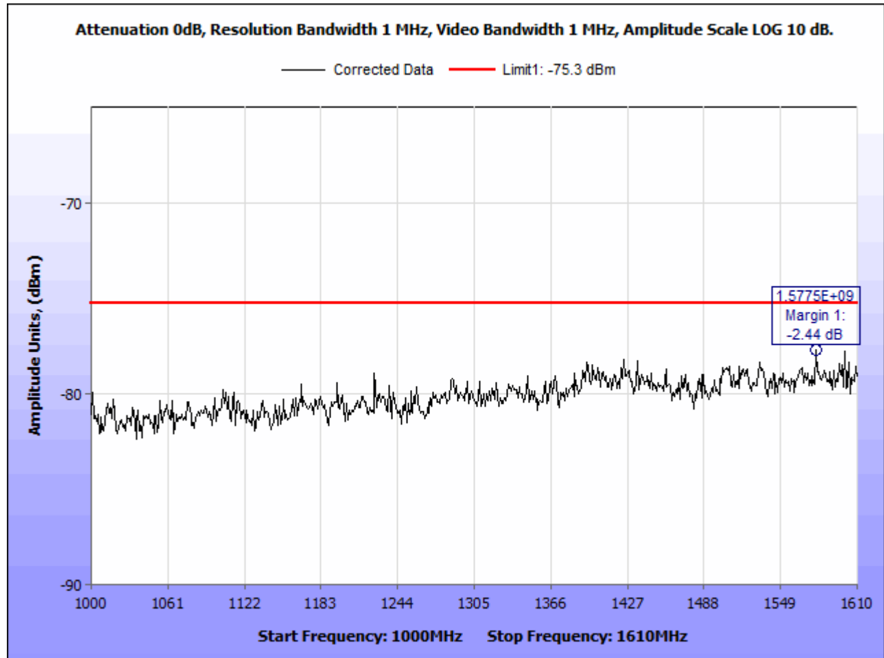
Figure 9. Radiated Emission Limits Test Results, 1 GHz – 1.610 GHz
