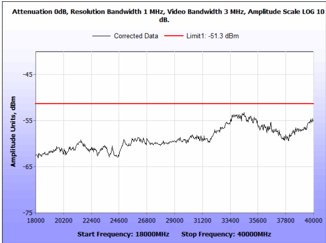
Figure 14. Radiated Emission Limits Test Results, 18 GHz – 40 GHz
