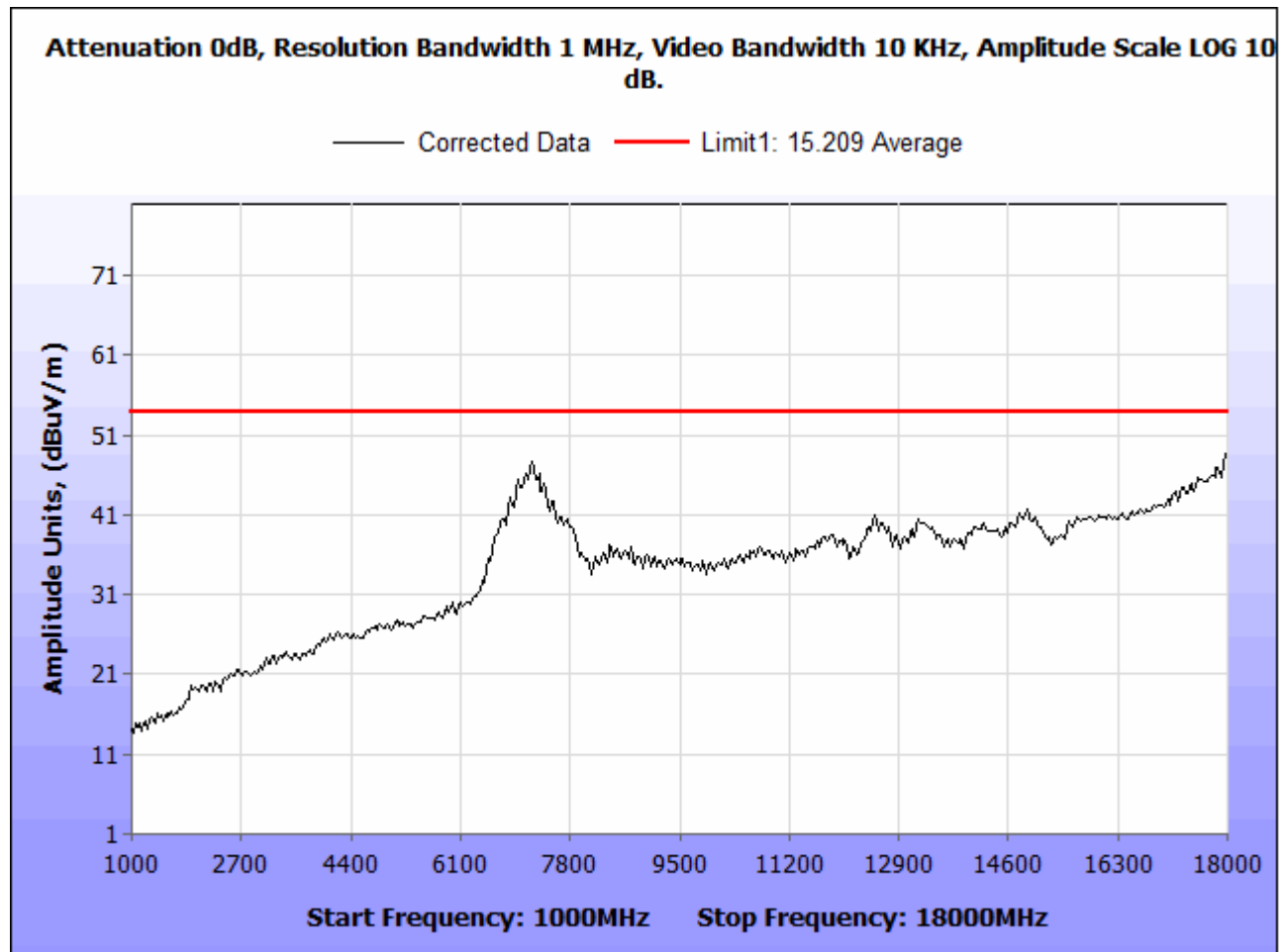
Figure 4. Radiated Emissions Average, 1 GHz – 18 GHz
