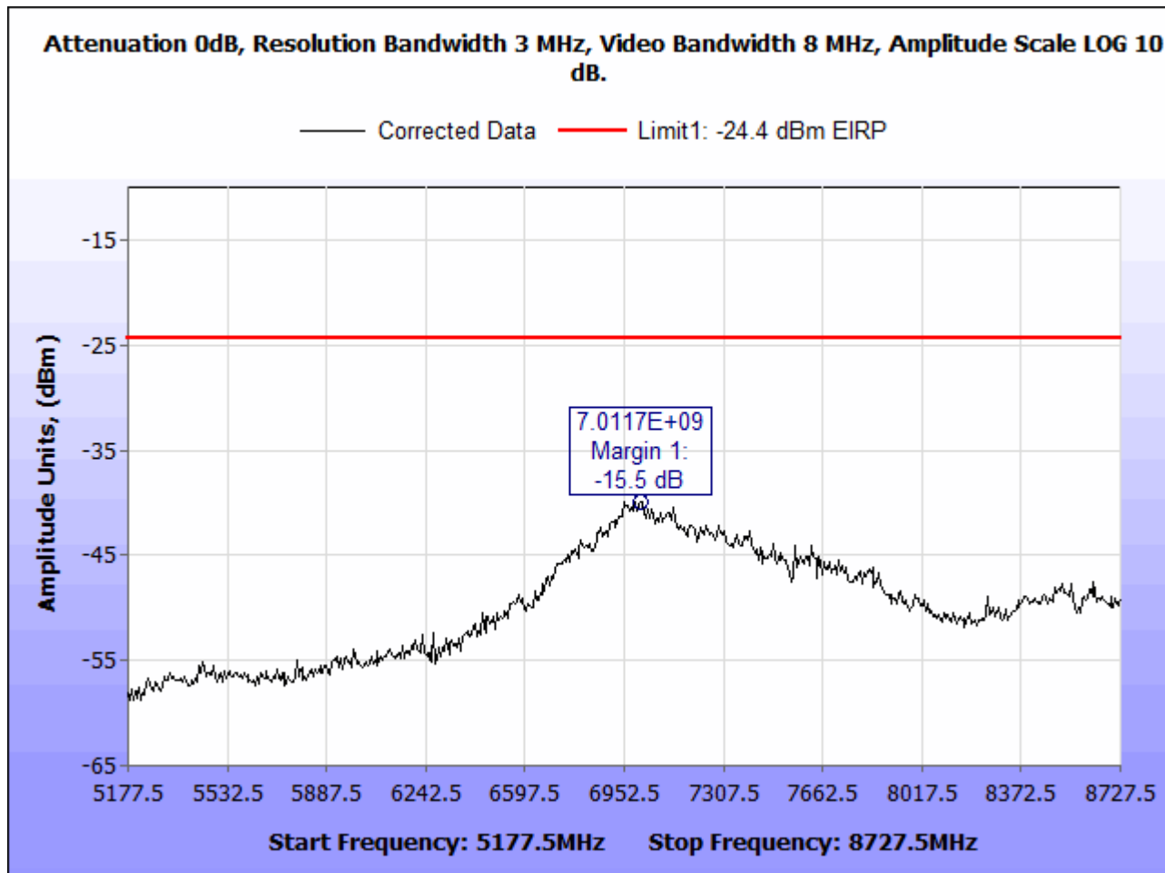
Figure 17. Peak Radiated Emissions Level EIRP
