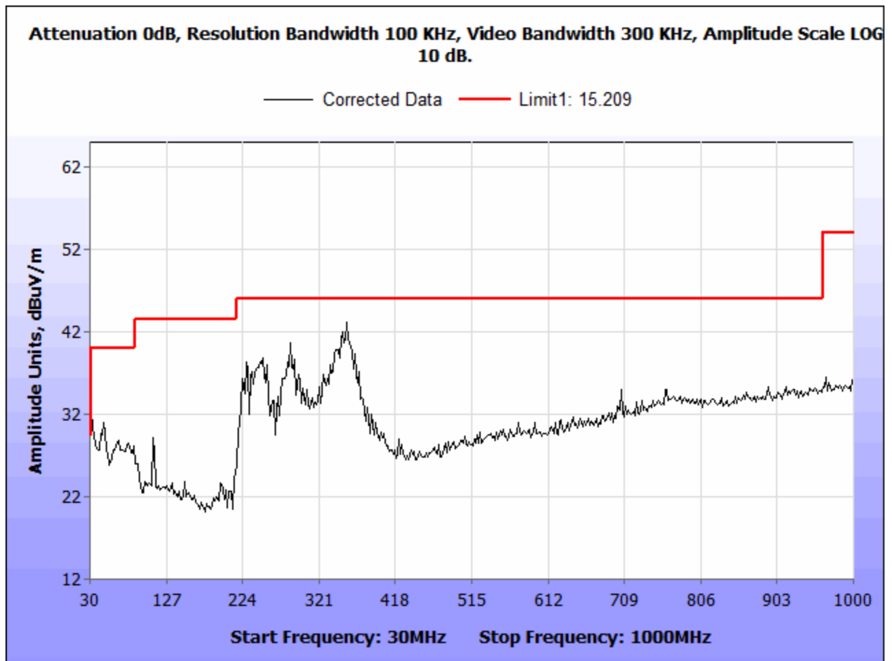
Figure 7. Radiated Emission Limits Test Results, 30 MHz – 1000 MHz
