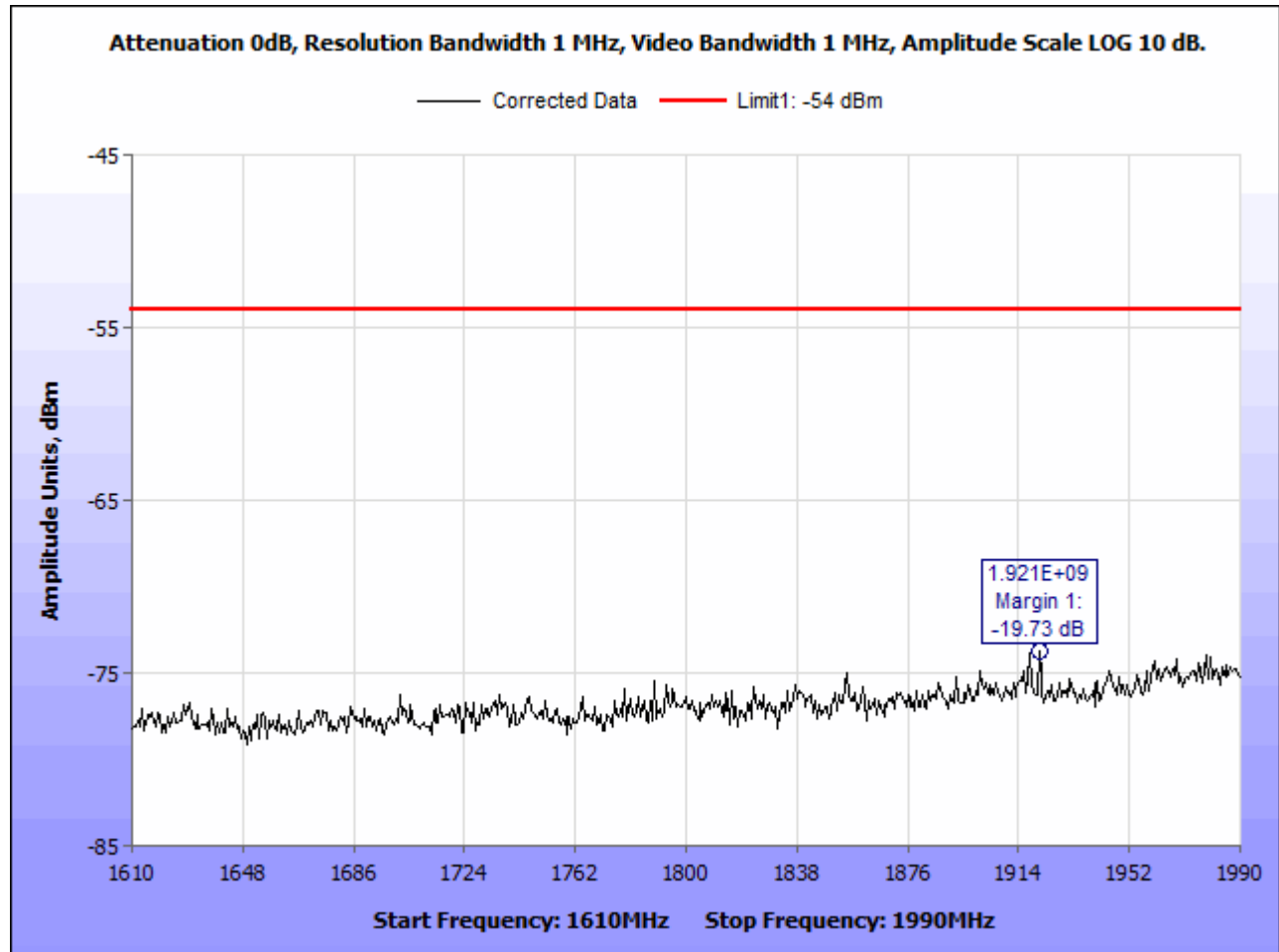
Figure 10. Radiated Emission Limits Test Results, 1610 MHz – 1990 MHz
