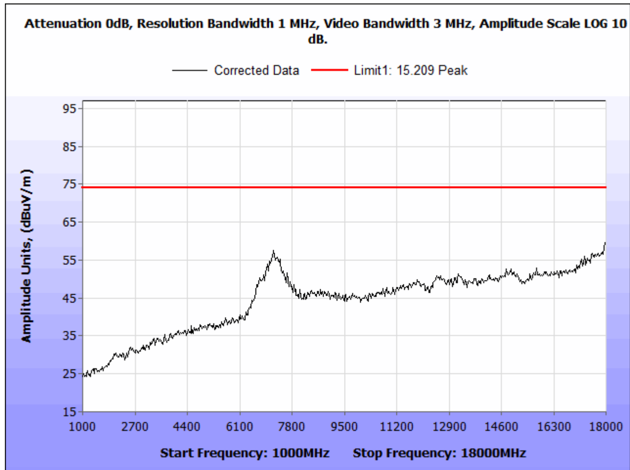
Figure 3. Radiated Emissions Peak, 1 GHz – 18 GHz
