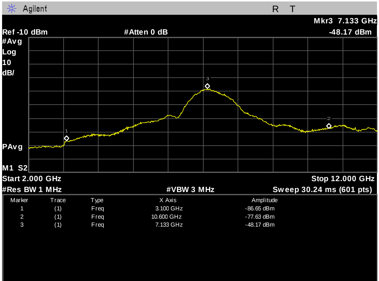
Figure 6. UWB Bandwidth, Test Results UWB Bandwidth contained between 3100 MHz – 10.6 GHz
