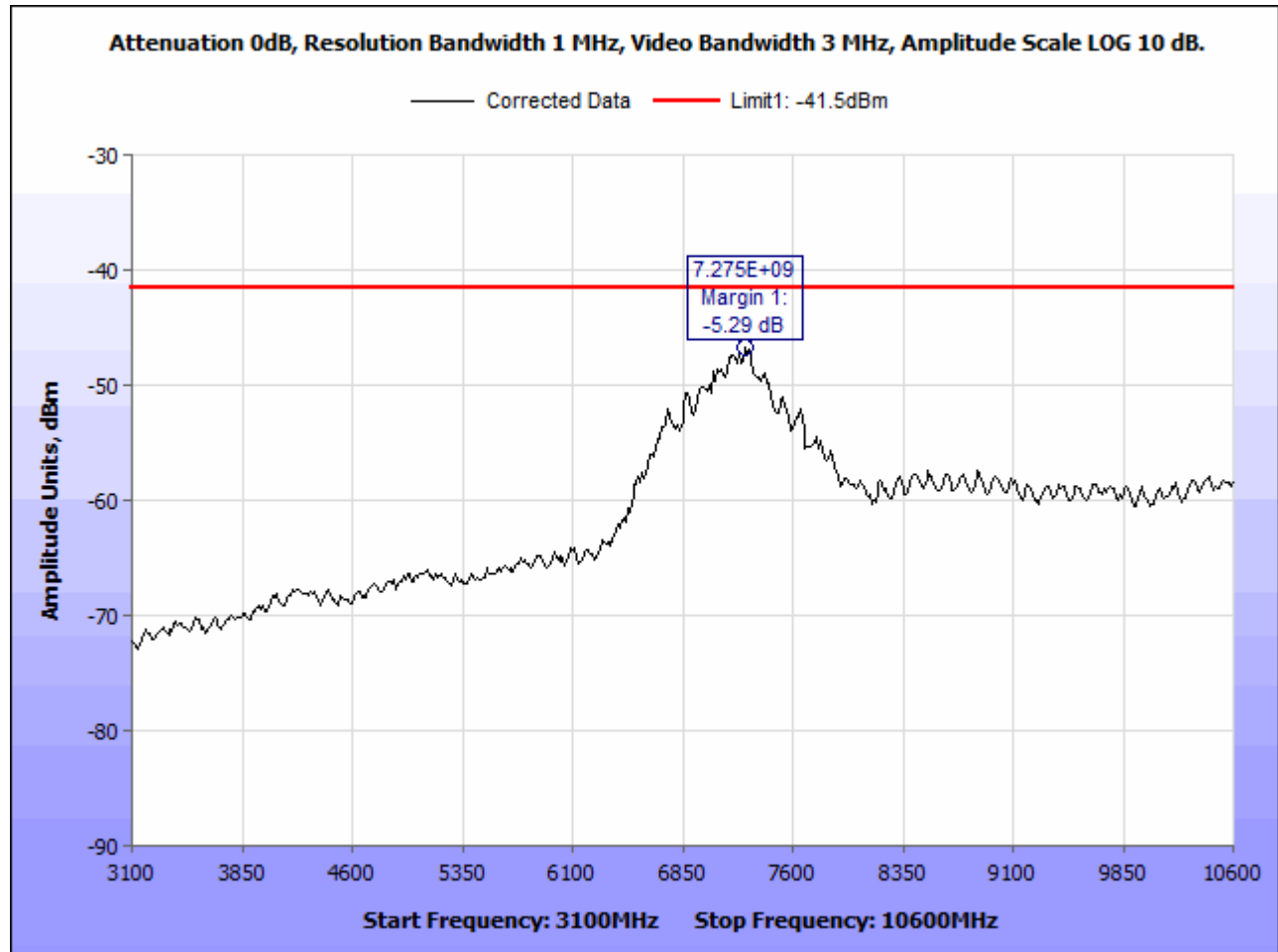
Figure 12. Radiated Emission Limits Test Results, 3100 MHz – 10.6 GHz
