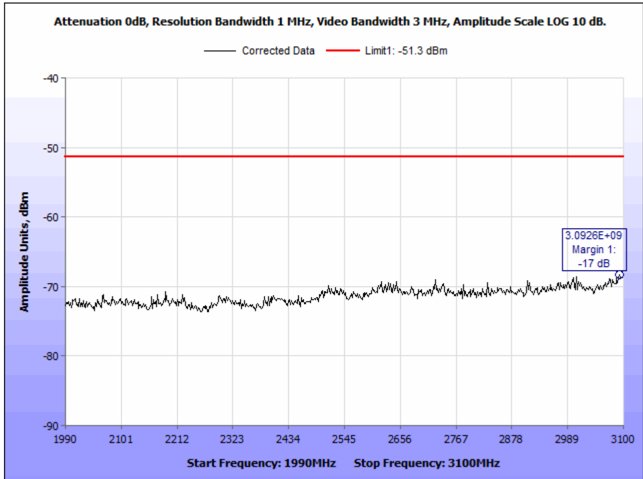
Figure 11. Radiated Emission Limits Test Results, 1990 MHz – 3100 MHz
