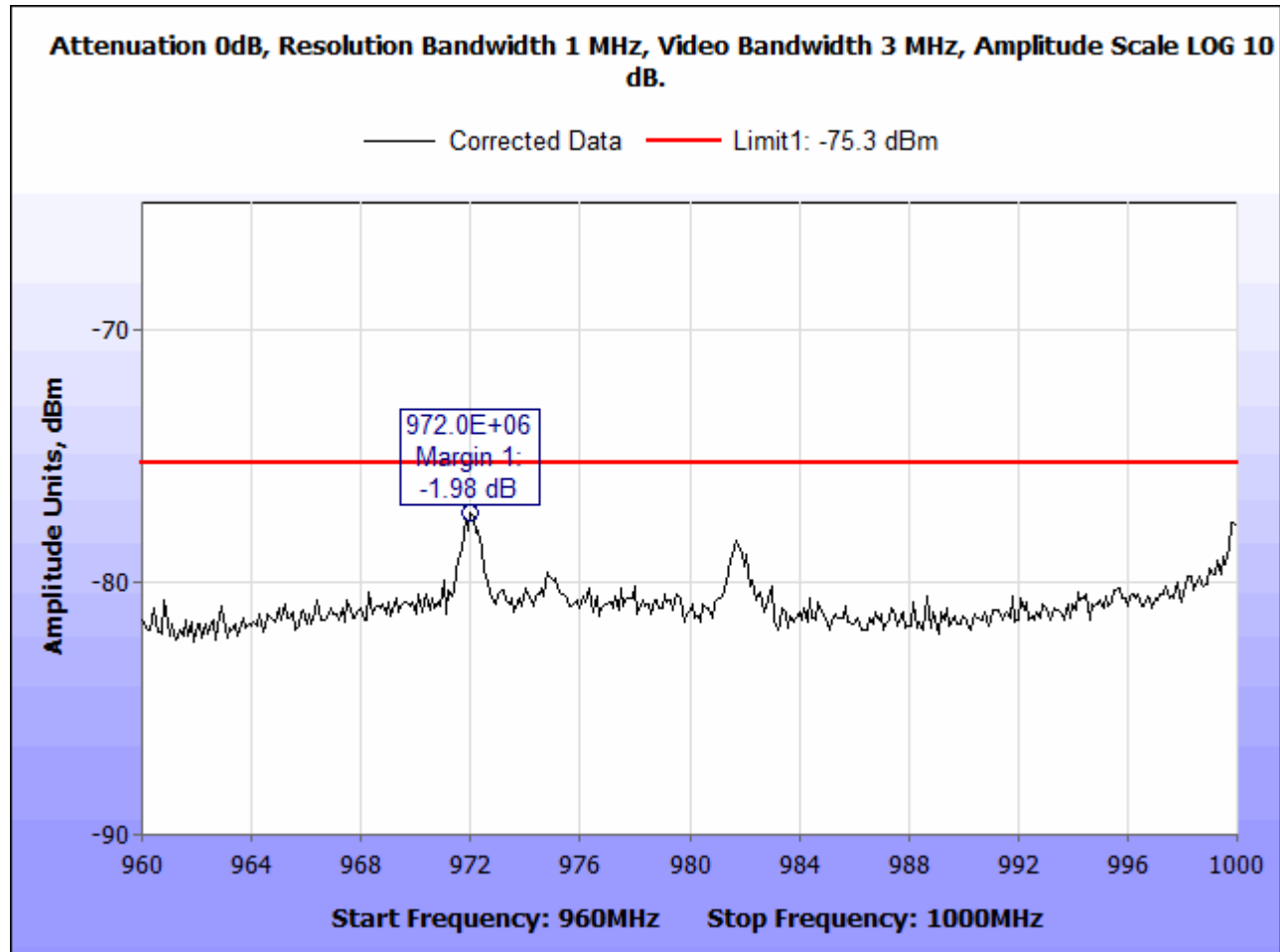
Figure 8. Radiated Emission Limits Test Results, 960 MHz – 1 GHz
