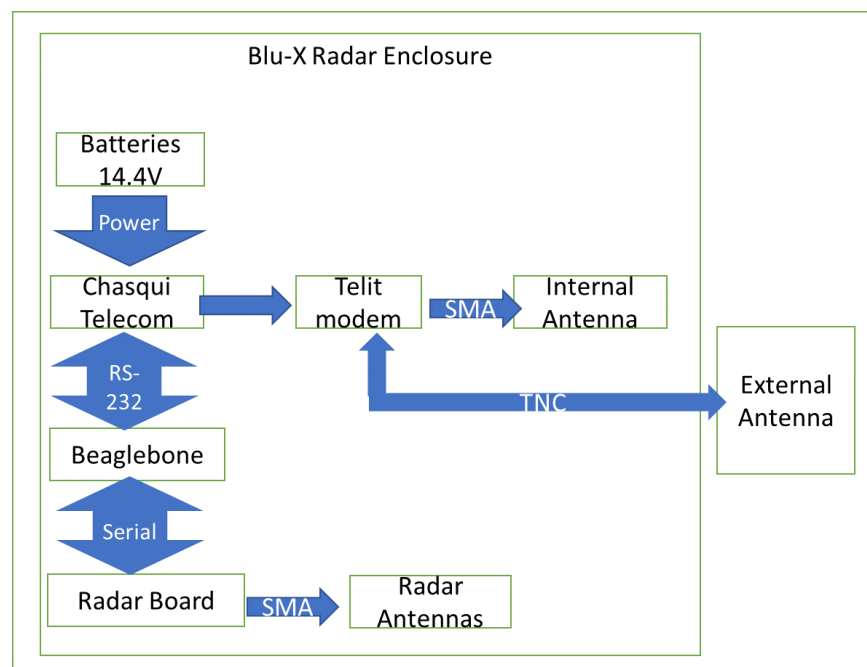
Figure 1. Block Diagram of BluX Radar Sensor
