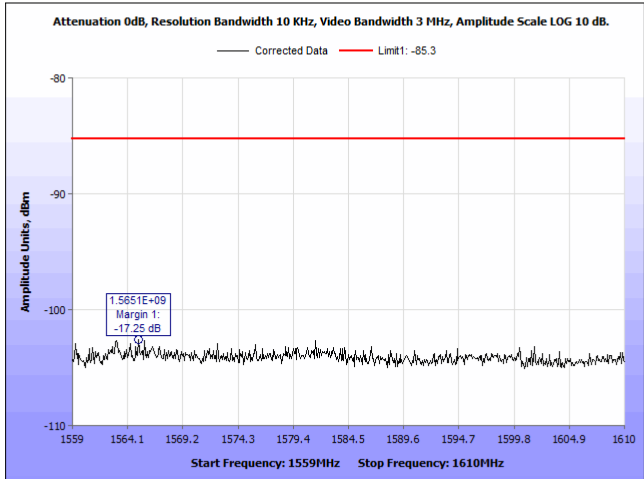
Figure 16. GPS emissions Requirements, 1559 MHz – 1610 MHz
