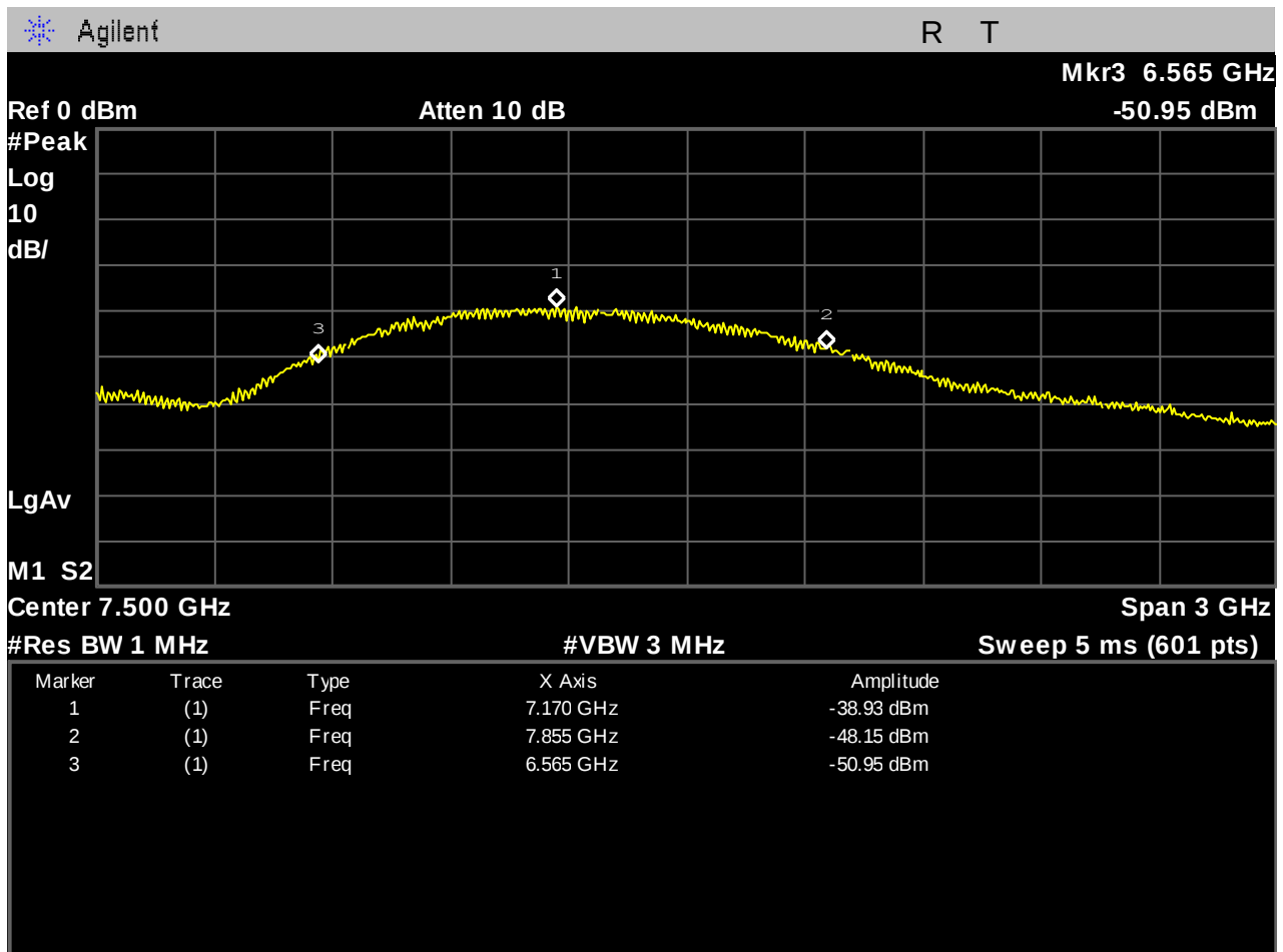
Figure 6. UWB Bandwidth, Test Results, 10dB Bandwidth
