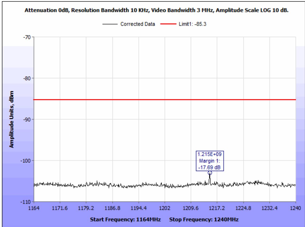
Figure 15. GPS emissions Requirements, 1164 MHz – 1240 MHz
