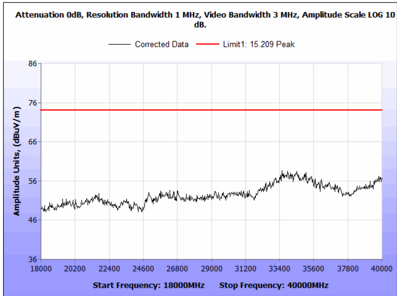
Figure 5. Radiated Emissions Peak, 18 GHz – 40 GHz
