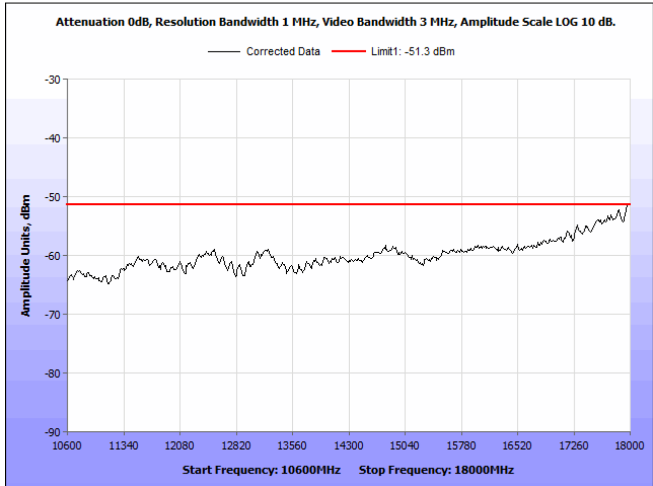
Figure 13. Radiated Emission Limits Test Results, 10.6 GHz – 18 GHz
