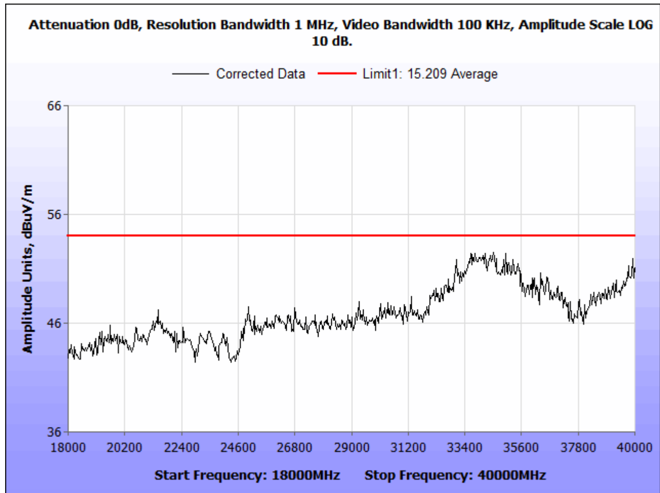
Figure 6. Radiated Emissions Average, 18 GHz – 40 GHz
