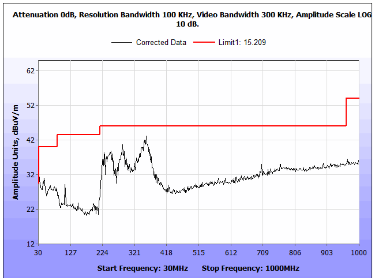
Figure 2. Radiated Emissions 30 MHz – 1 GHz
