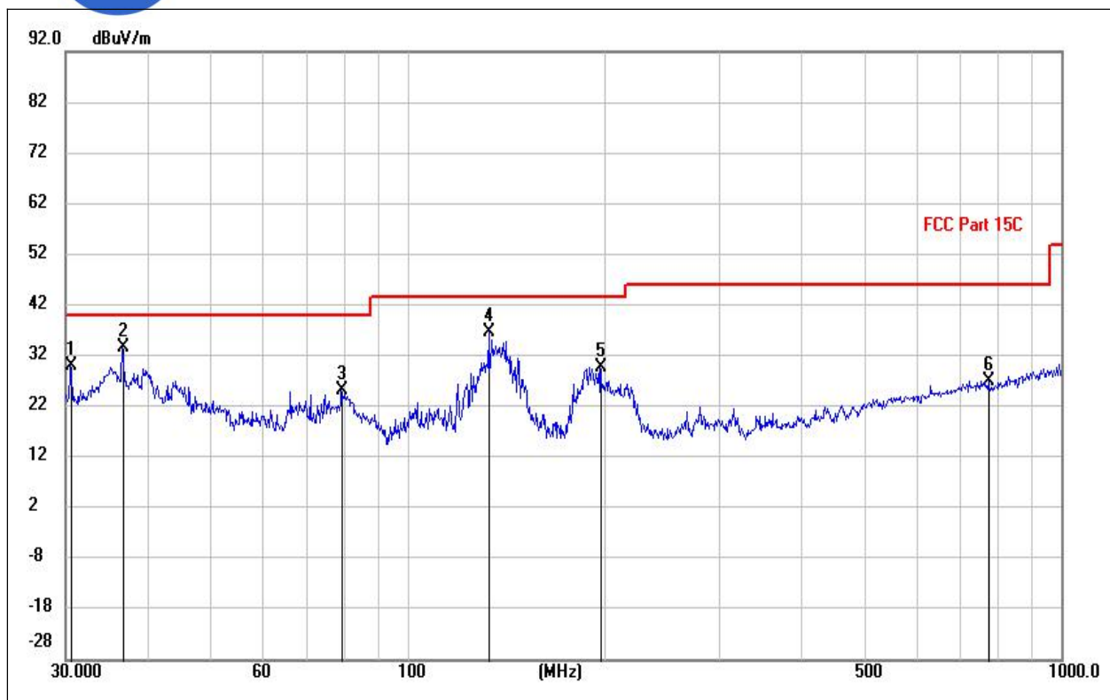
(LE 1M PHY _2442MHz, Antenna Vertical, 30MHz to 1GHz)
