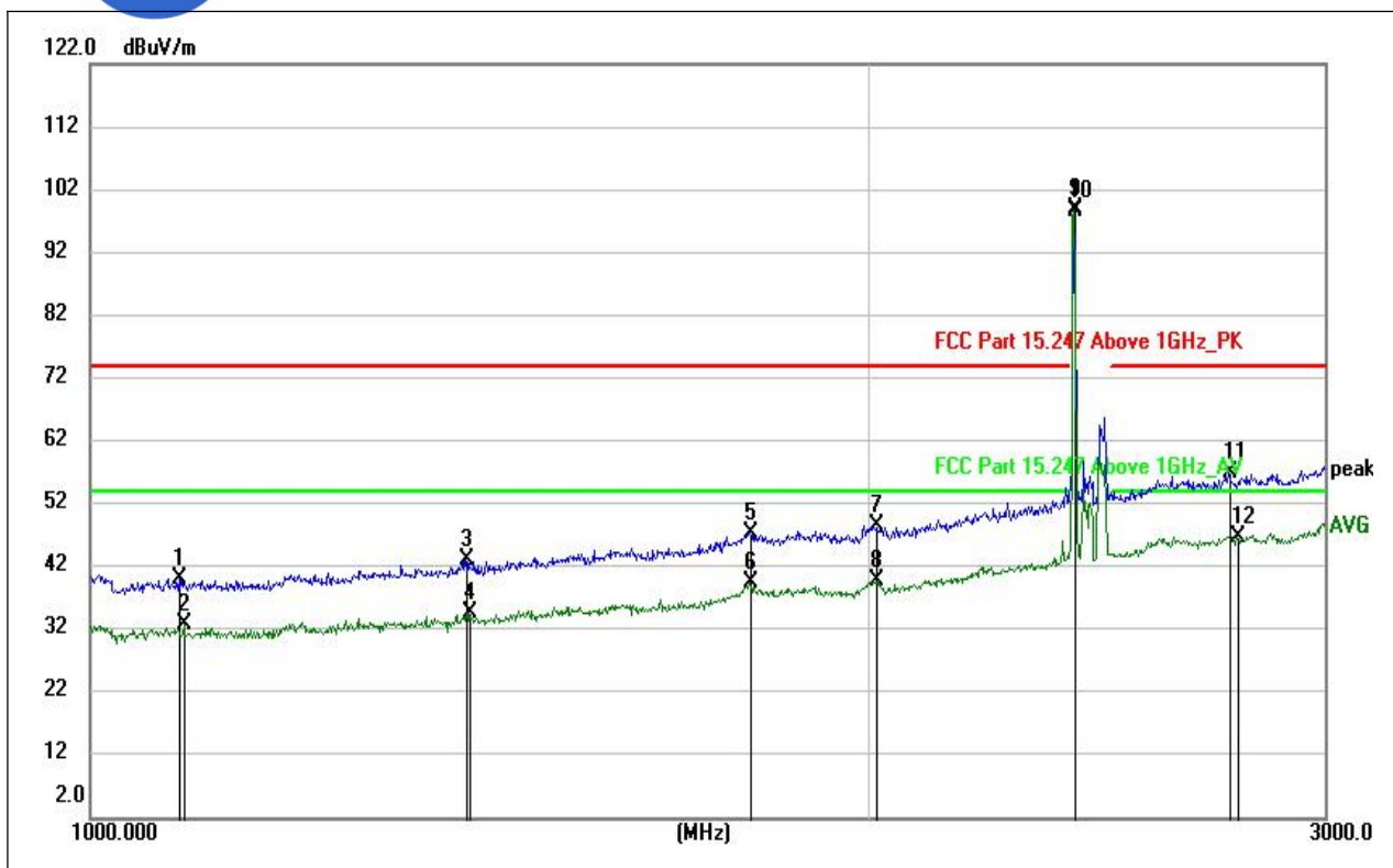
(LE 1M PHY _2402MHz, Antenna Horizontal, 1GHz to 3GHz)
