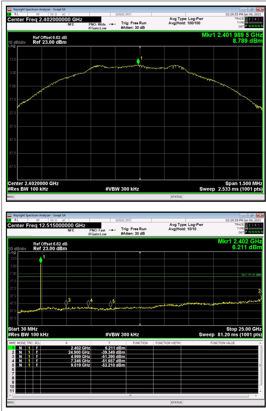
(Channel = 0, 30MHz to 25GHz)
