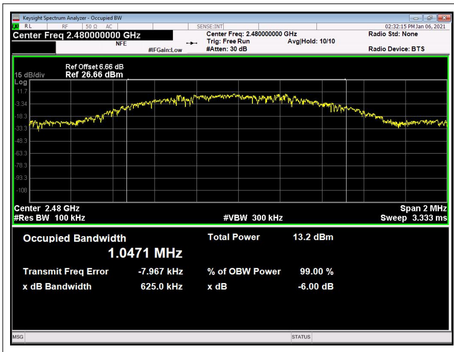
(Channel 39: 2480MHz)
