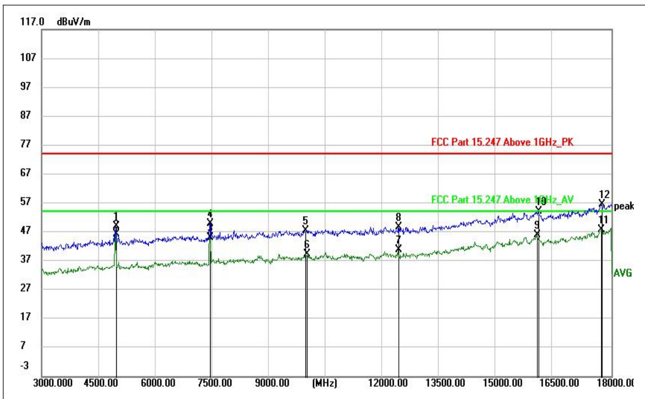
(LE 1M PHY _2480MHz, Antenna Vertical, 3GHz to 18GHz)
