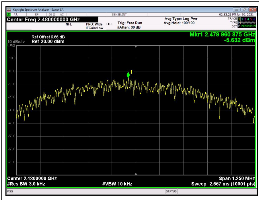
(Channel = 39, 2480MHz)
