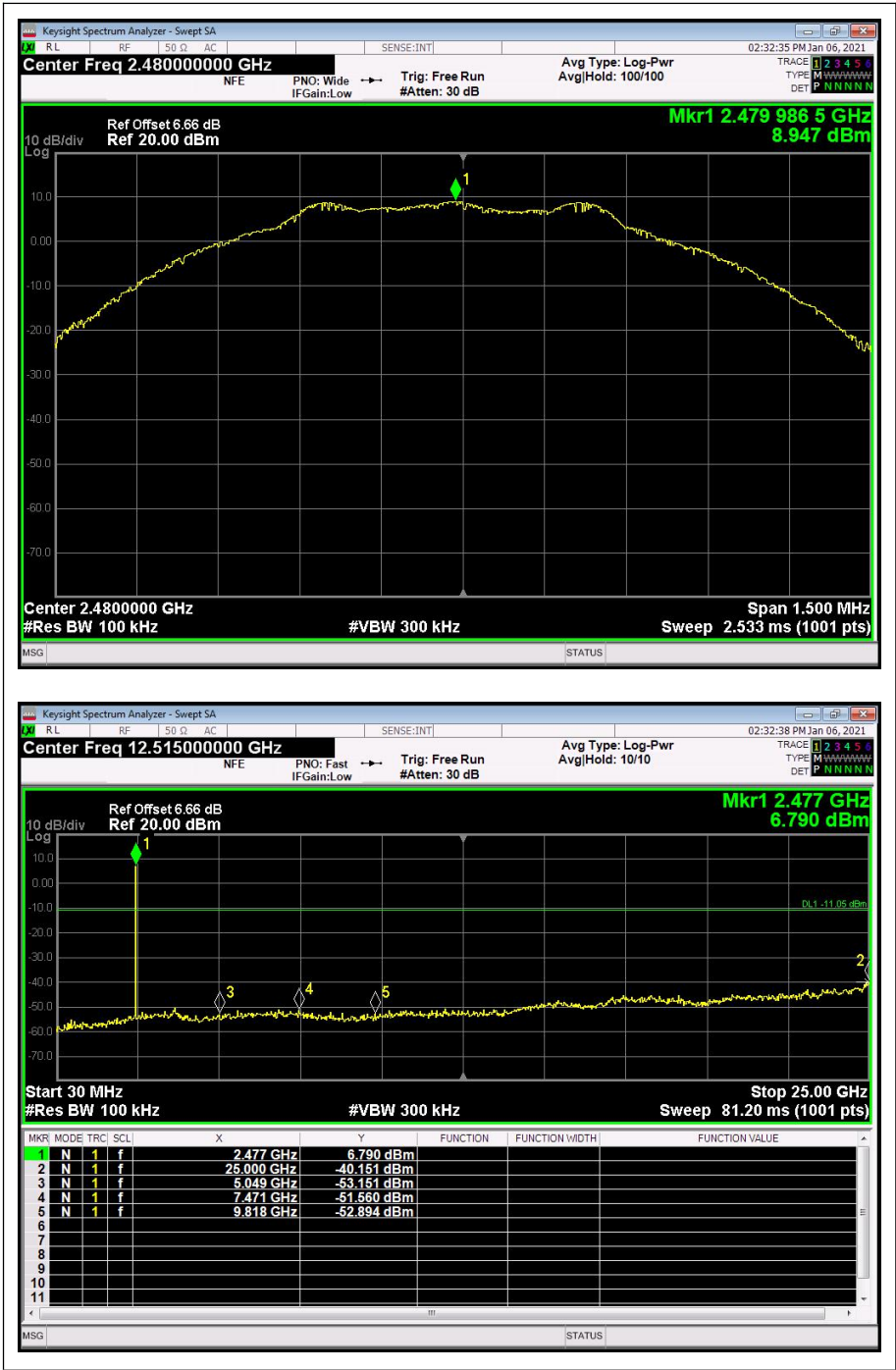
(Channel = 39, 30MHz to 25GHz)
