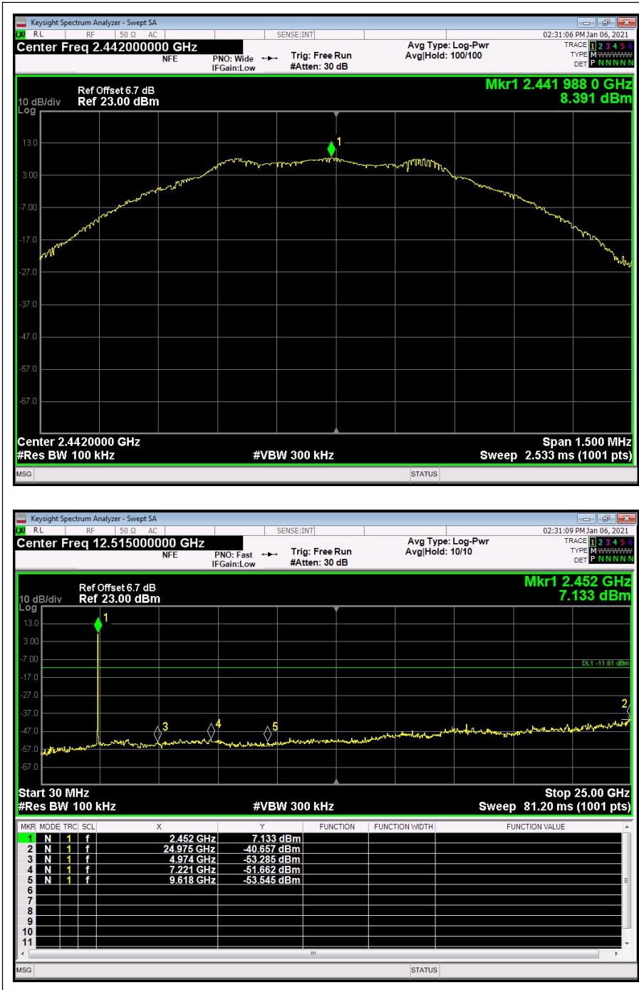
(Channel = 20, 30MHz to 25GHz)
