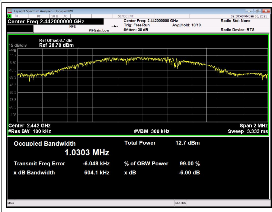
(Channel 20: 2442 MHz)
