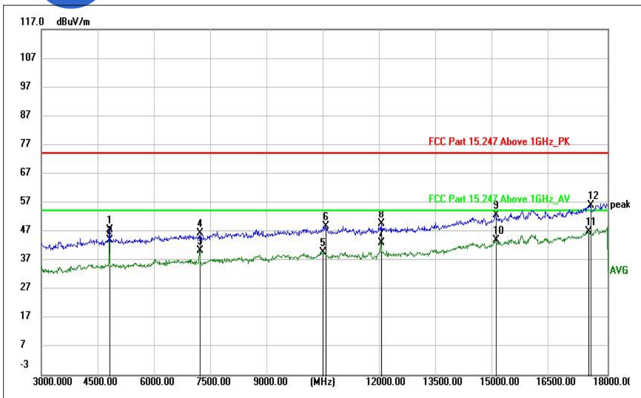
(LE 1M PHY _2402MHz, Antenna Horizontal, 3GHz to 18GHz)
