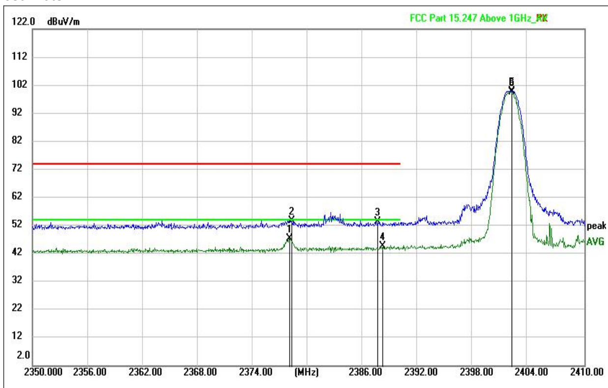
(BLE 1M PHY_2402MHz, Antenna Horizontal)
