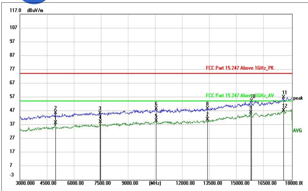
(LE 1M PHY _2480MHz, Antenna Horizontal, 3GHz to 18GHz)
