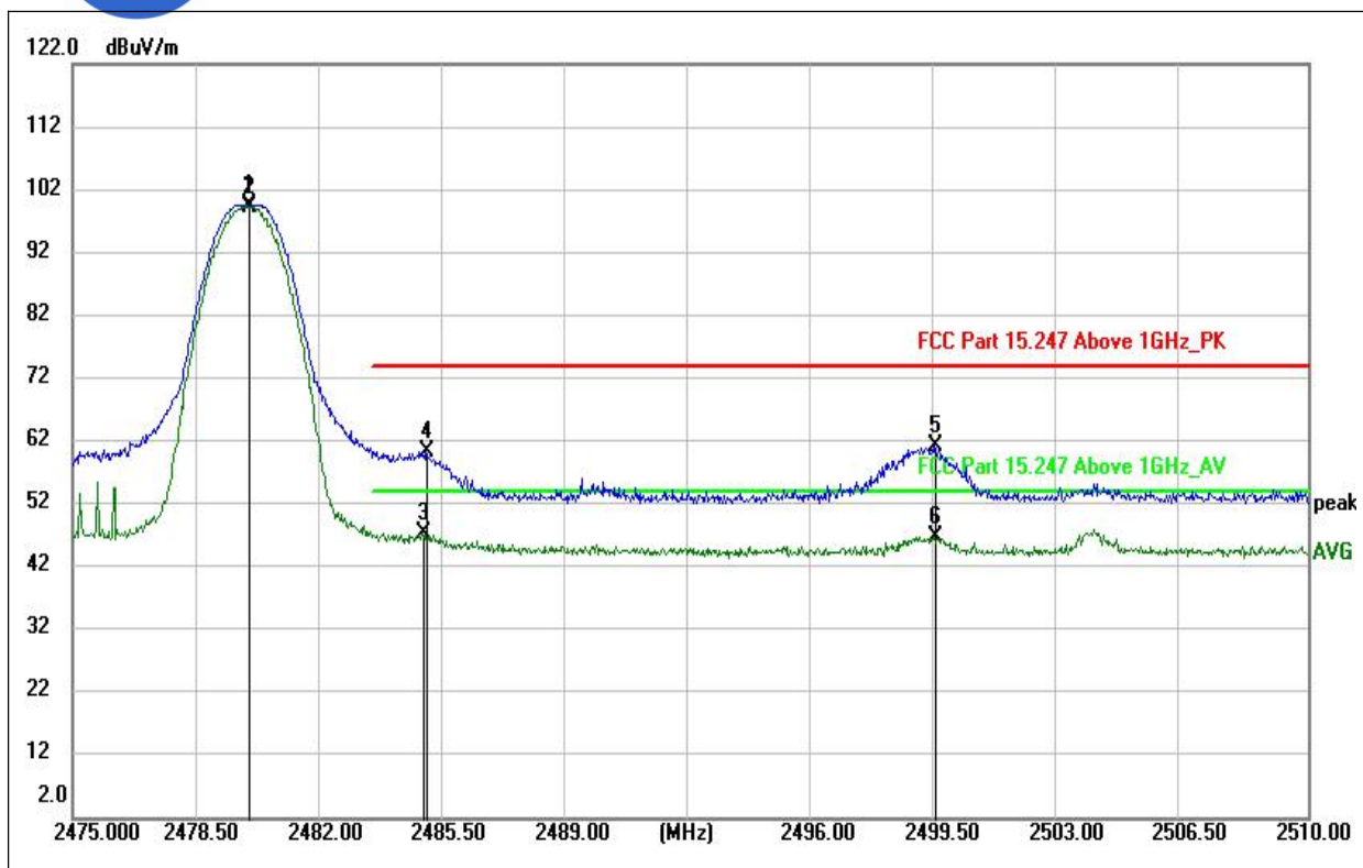
(LE 1M PHY_2480MHz, Antenna Vertical)
