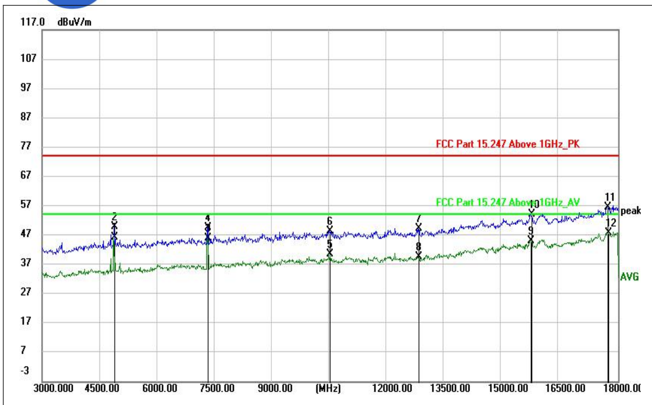
(LE 1M PHY _2442MHz, Antenna Vertical, 3GHz to 18GHz)
