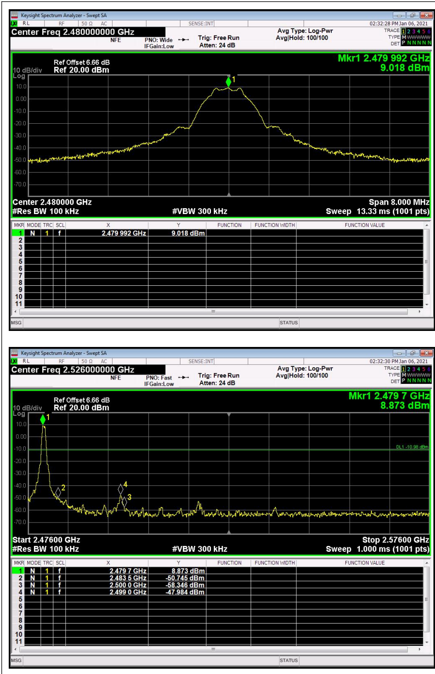
(Band Edge, Channel = 39)
