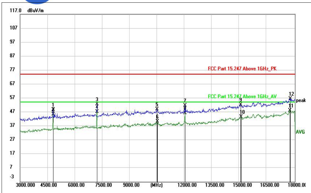
(LE 1M PHY _2402MHz, Antenna Vertical, 3GHz to 18GHz)
