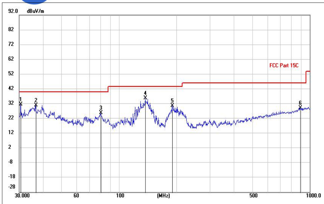
(LE 1M PHY _2402MHz, Antenna Vertical, 30MHz to 1GHz)
