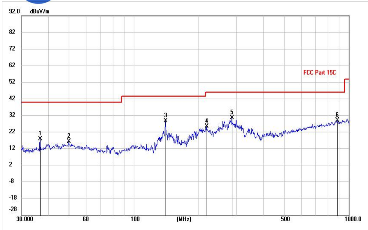
(LE 1M PHY _2480MHz, Antenna Horizontal, 30MHz to 1GHz)
