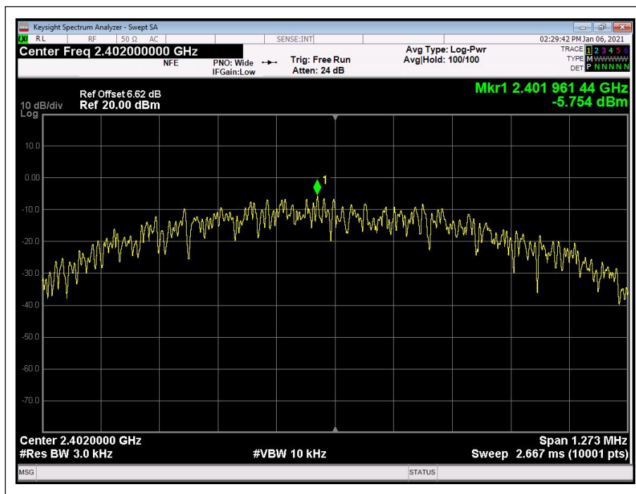
(Channel = 0, 2402MHz)
