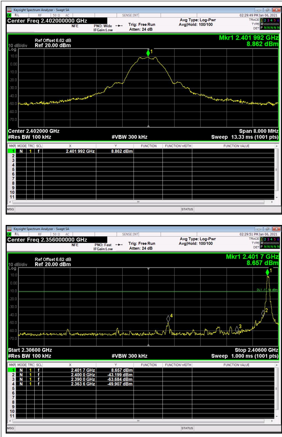
(Band Edge, Channel = 0)
