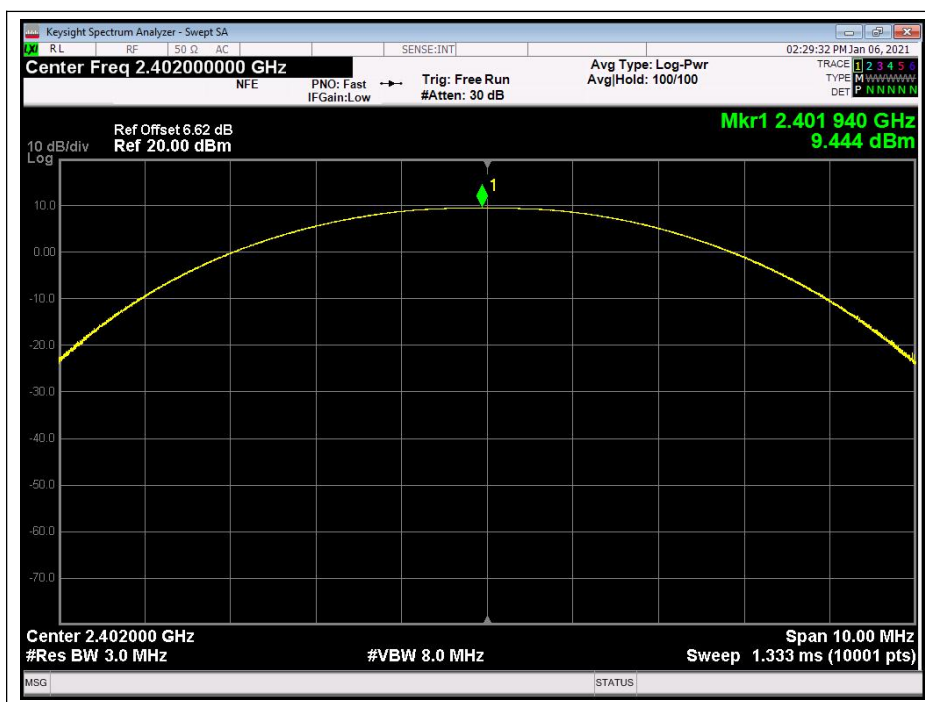
(Channel 0, 2402MHz)
