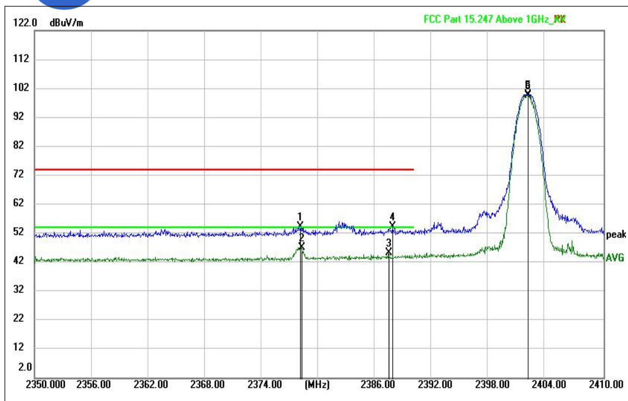
(LE 1M PHY_2402MHz, Antenna Vertical)
