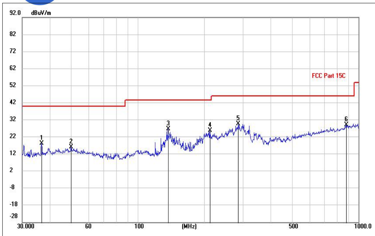
(LE 1M PHY _2442MHz, Antenna Horizontal, 30MHz to 1GHz)
