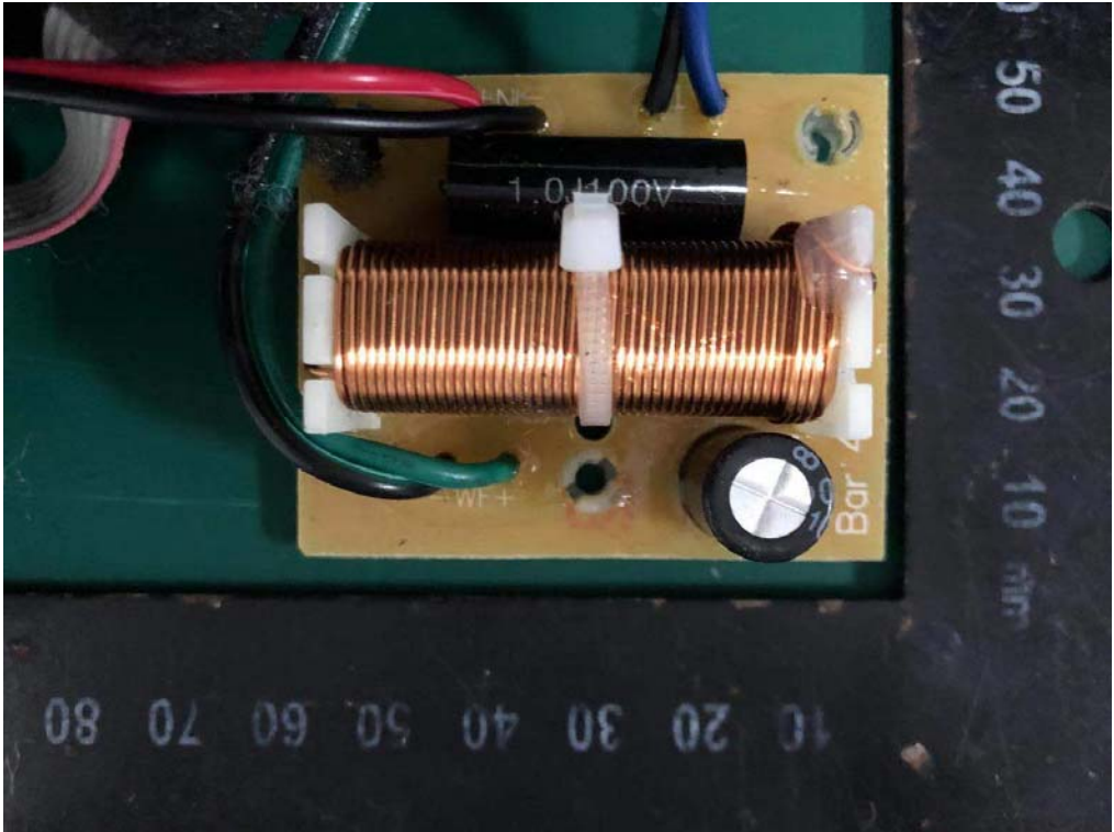
Internal Photos M/N: Bar 40 Sound Bar
