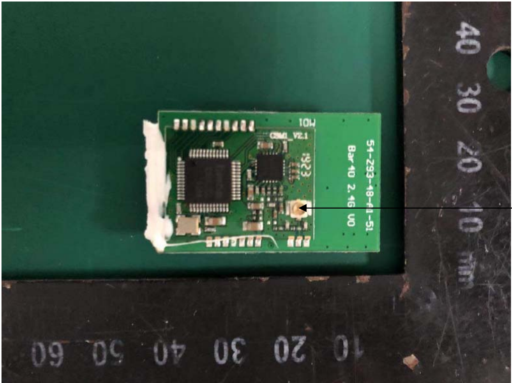
2.4G Antenna Port
