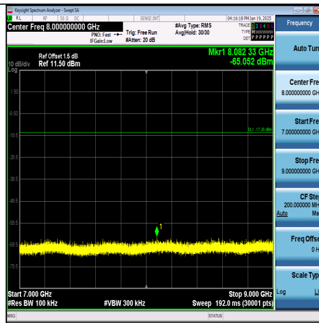
BLE_1M-Ant1-2440-7000~9000-PASS
