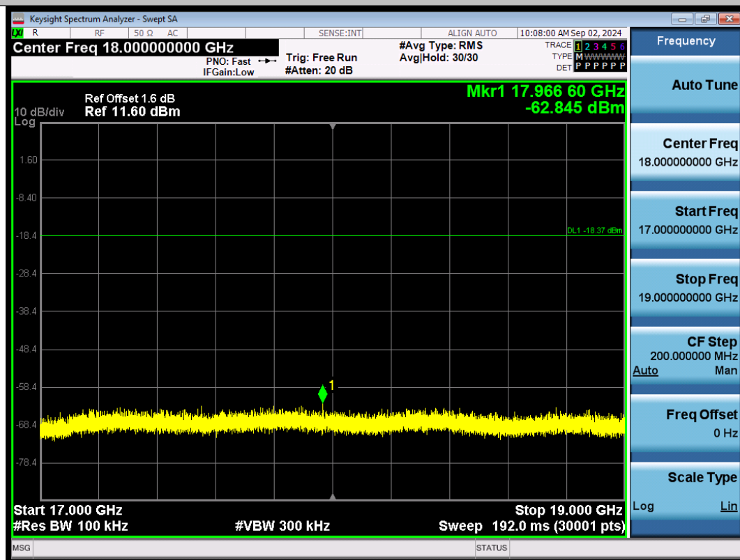
Thread-Ant1-2480-17000~19000-PASS
