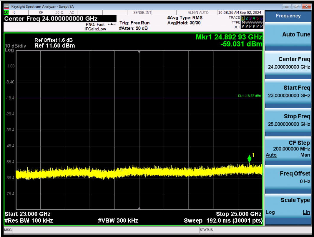
Thread-Ant1-2480-23000~25000-PASS
