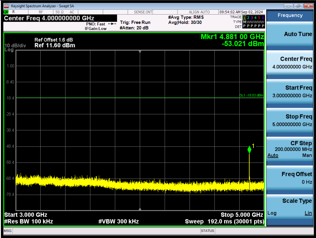
Thread-Ant1-2440-3000~5000-PASS
