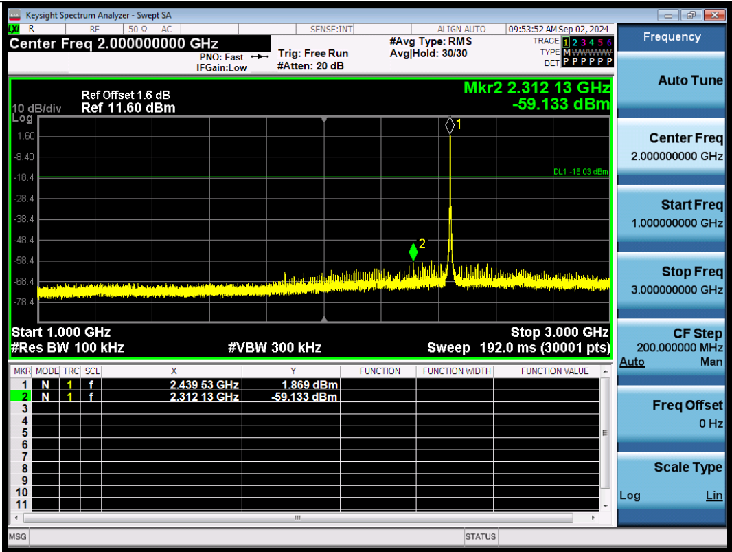
Thread-Ant1-2440-1000~3000-PASS
