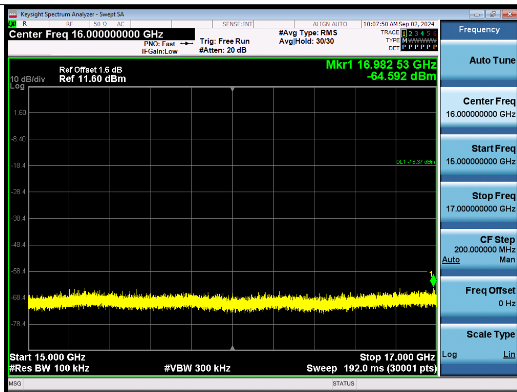
Thread-Ant1-2480-15000~17000-PASS
