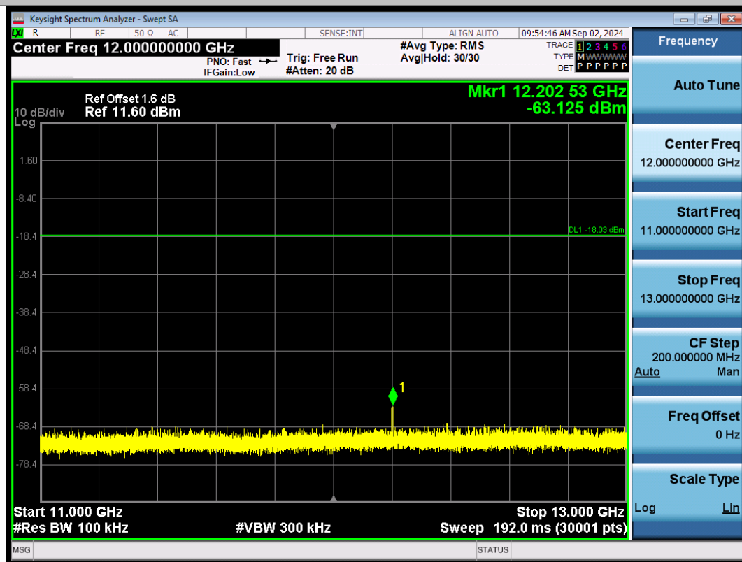
Thread-Ant1-2440-11000~13000-PASS
