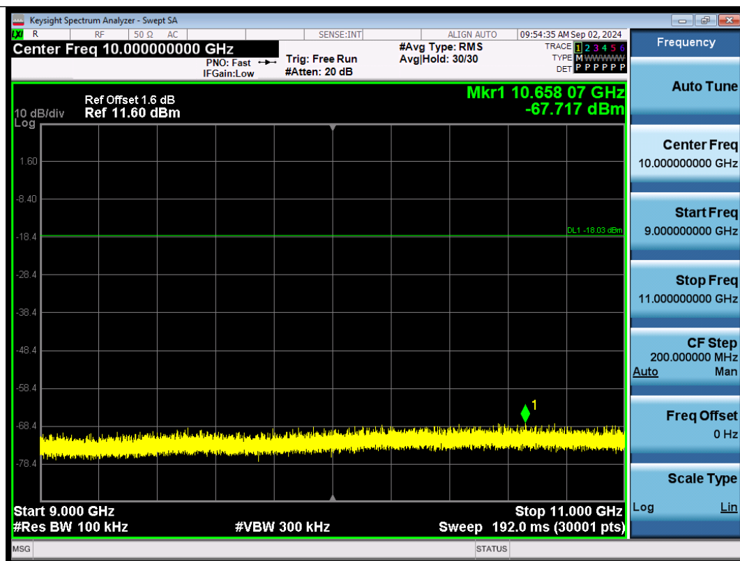
Thread-Ant1-2440-9000~11000-PASS
