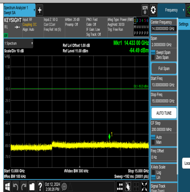
Thread-Ant1-2405-13000~15000-PASS
