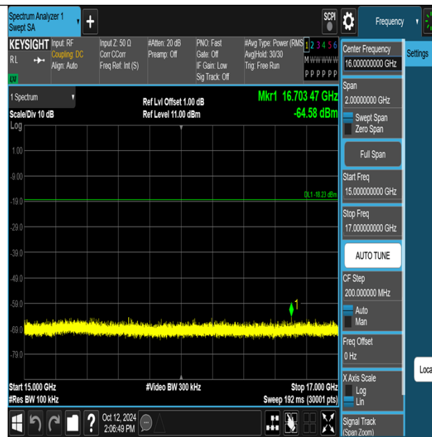
Thread-Ant1-2405-15000~17000-PASS
