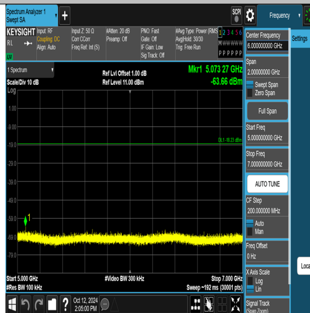
Thread-Ant1-2405-5000~7000-PASS
