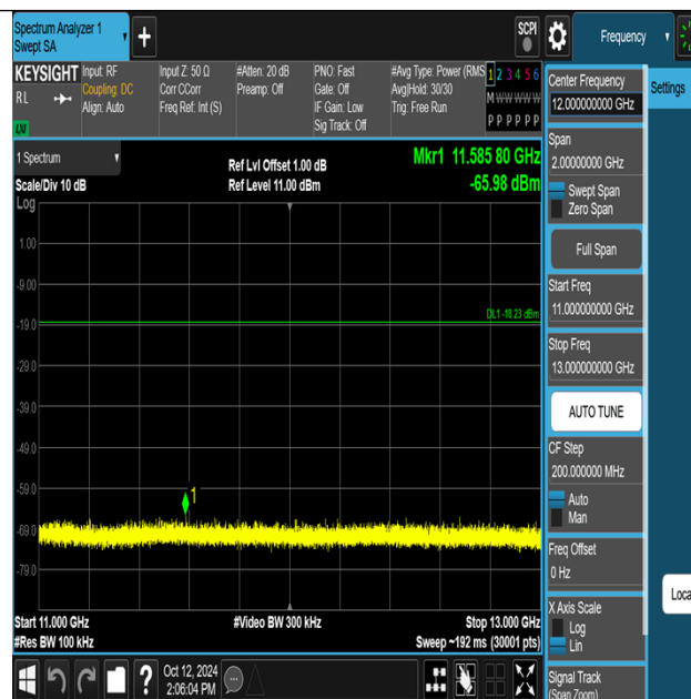
Thread-Ant1-2405-11000~13000-PASS
