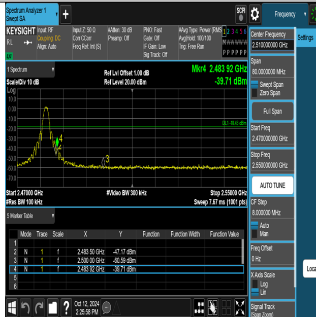
Thread-Ant1-2480-PASS
