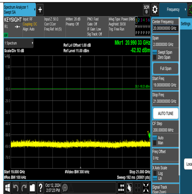
Thread-Ant1-2405-19000~21000-PASS
