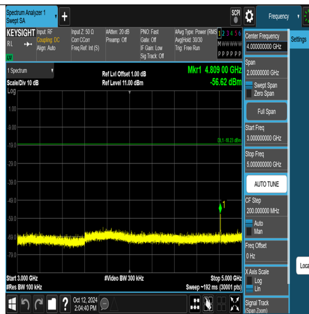
Thread-Ant1-2405-3000~5000-PASS
