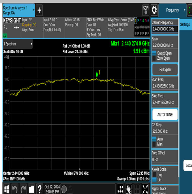
Thread-Ant1-2440-PASS
