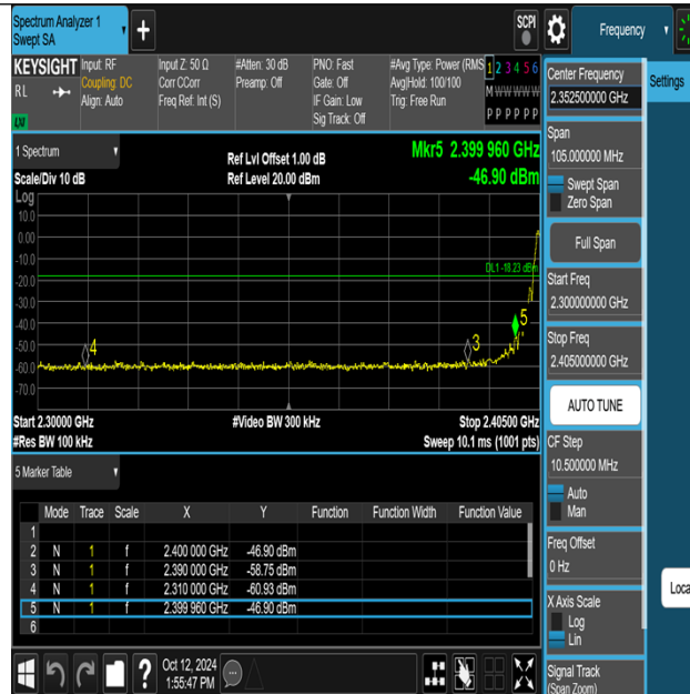
Thread-Ant1-2405-PASS
