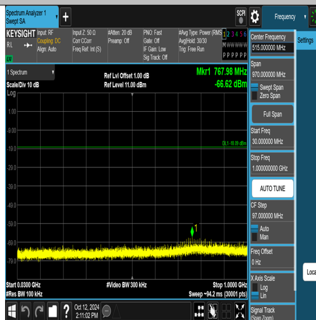
Thread-Ant1-2440-30~1000-PASS
