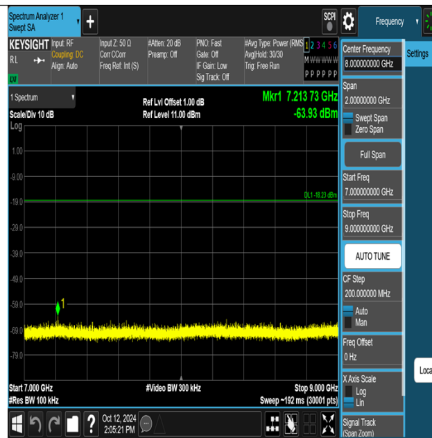
Thread-Ant1-2405-7000~9000-PASS
