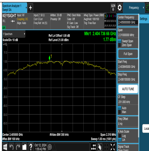
Thread-Ant1-2405-PASS
