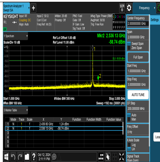
Thread-Ant1-2440-1000~3000-PASS
