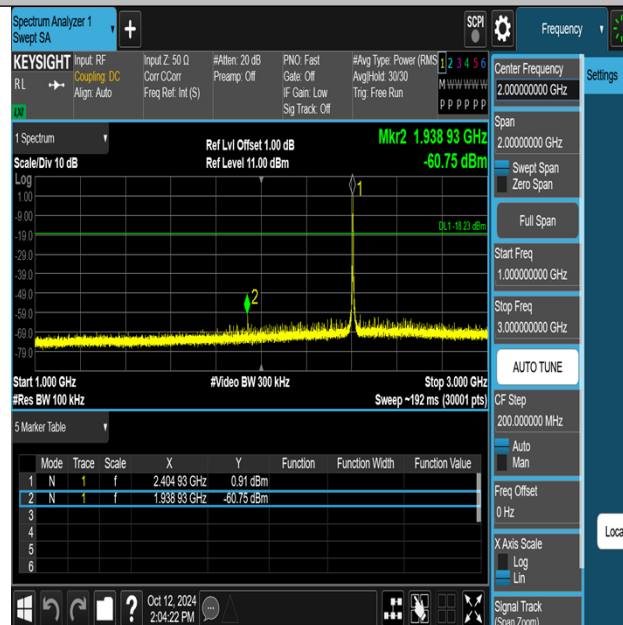
Thread-Ant1-2405-1000~3000-PASS
