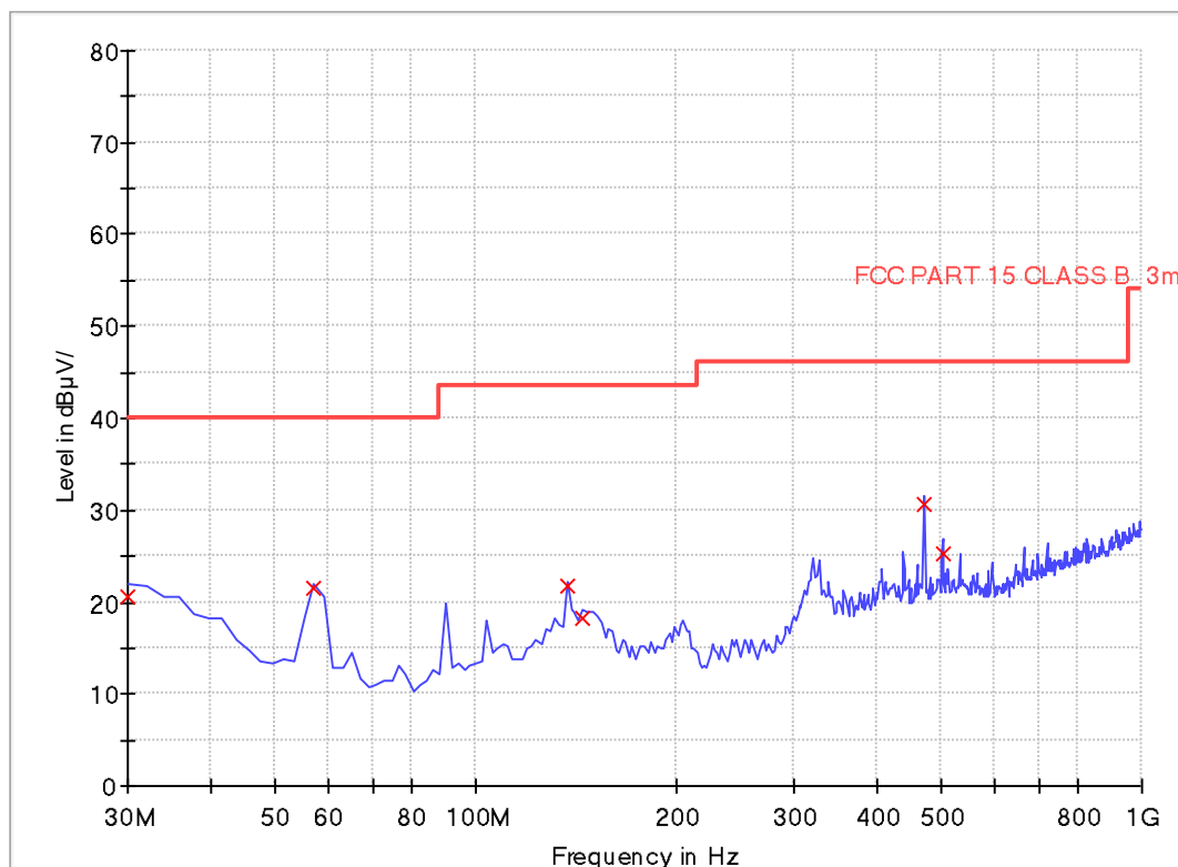
EMI Sweep-3M(30-1G)
