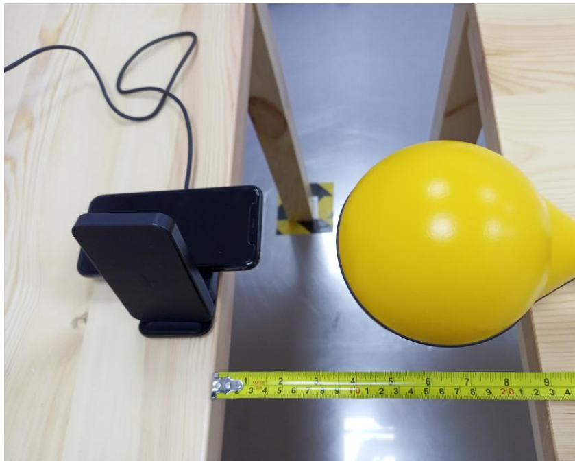
Test setup of D side (For Coil 2)
