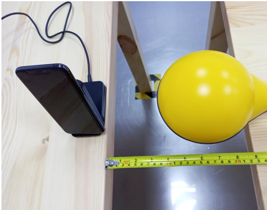
Test setup of D side (For Coil 1)
