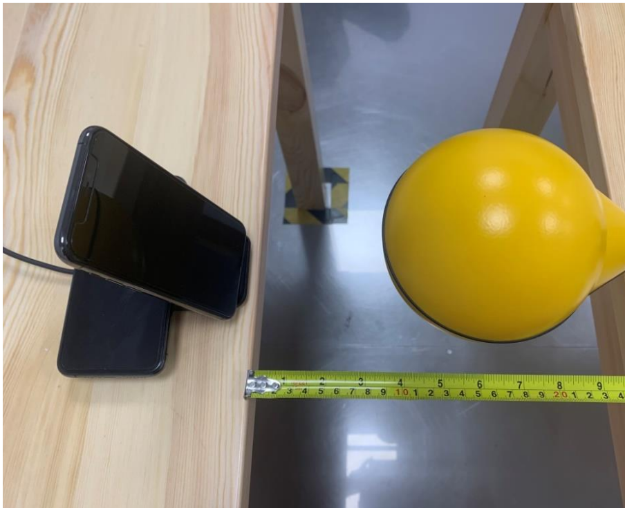
Test setup of A side (For Coil 1 + Coil 2)
