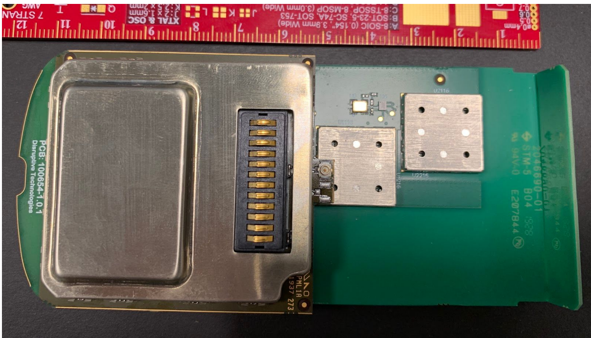
Figure 2: Picture of the bottom of the part 101941 DT-RFIO-Module (US)
