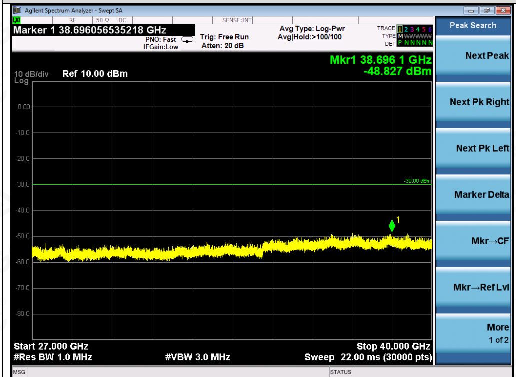
Test_Graph_802.11n40_ANT1_5270_MCS0_Frequency Band 5
