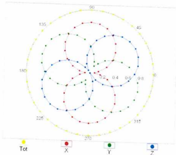
f=600 MHz,TEM
