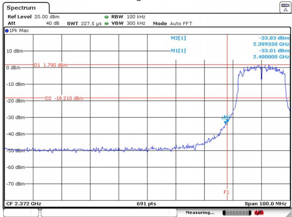
802.11g 2412MHz
