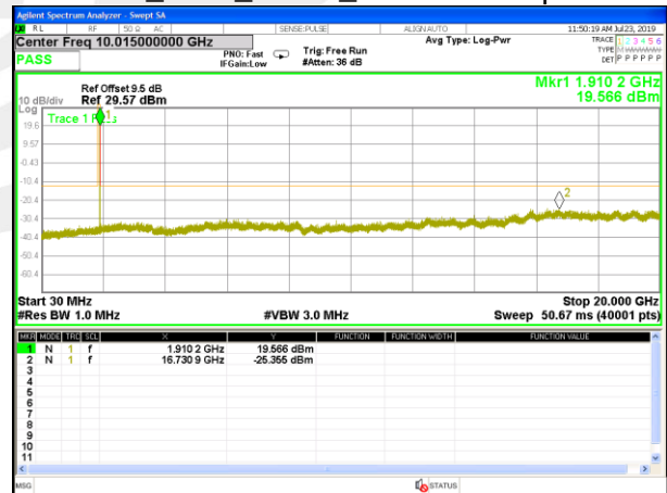
EGPRS_1900_Higher_Conducted Spurious
