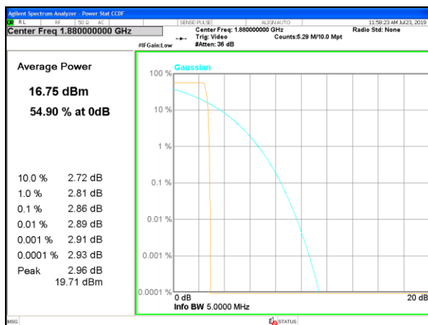
GPRS1900M
