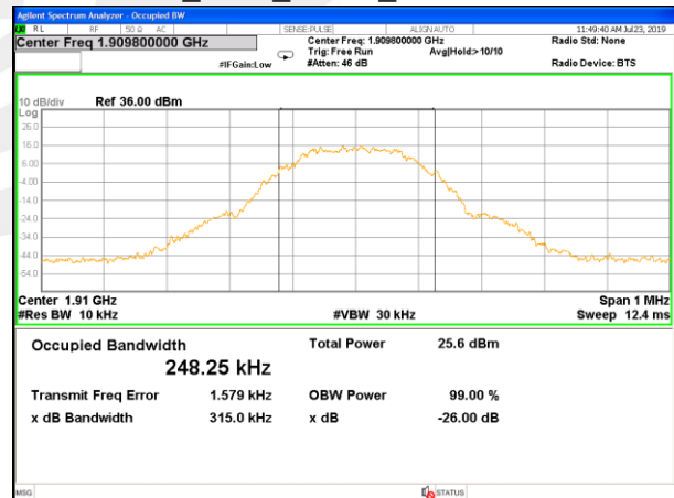
EGPRS_1900_Higher_26BW and 99%
