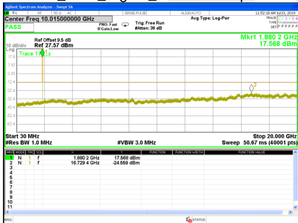
EGPRS_1900_Middle_Conducted Spurious
