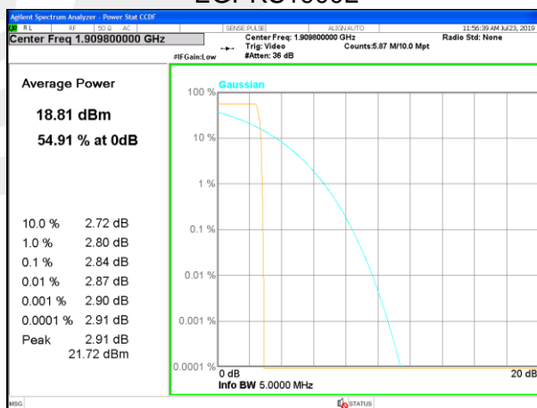
EGPRS1900H
