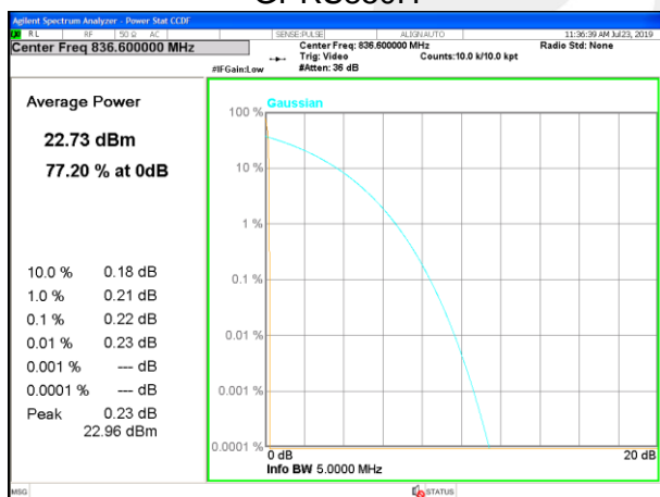
EGPRS850M
