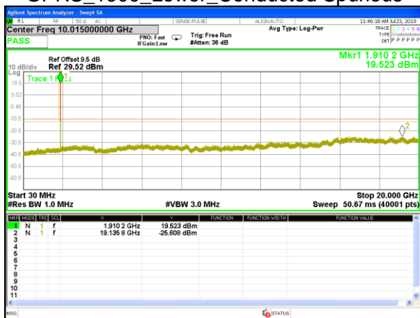
GPRS_1900_Higher_Conducted Spurious
