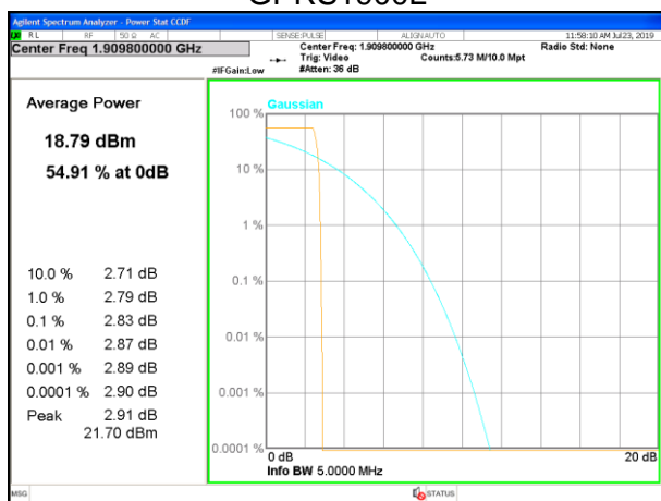
GPRS1900H
