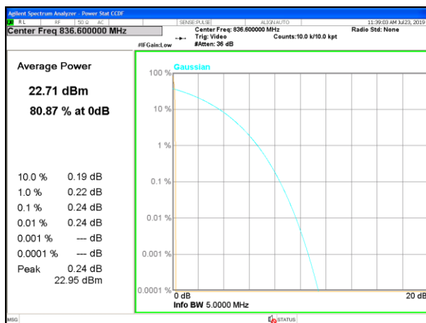
GPRS850M
