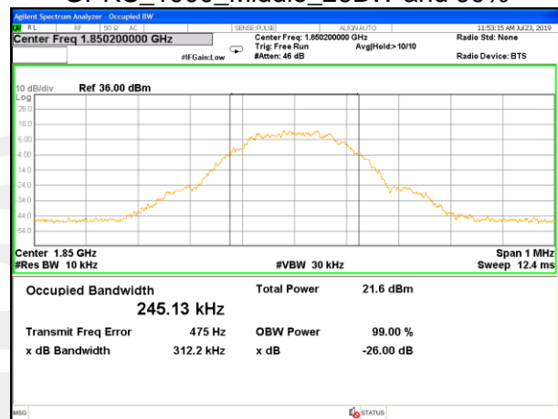
EGPRS_1900_Lower_26BW and 99%
