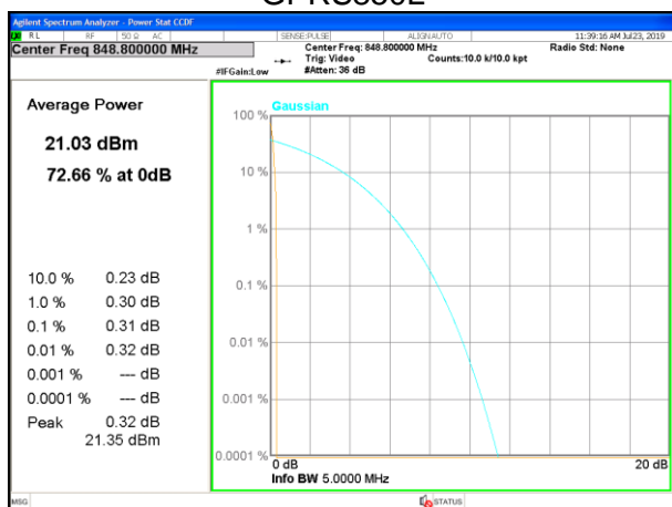
GPRS850H
