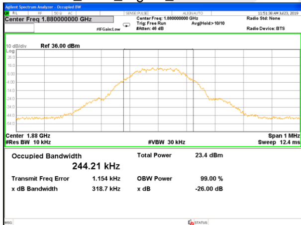
EGPRS_1900_Middle_26BW and 99%
