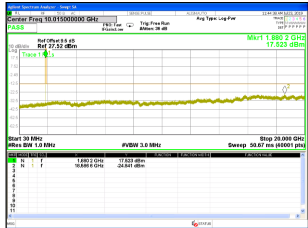
GPRS_1900_Middle_Conducted Spurious
