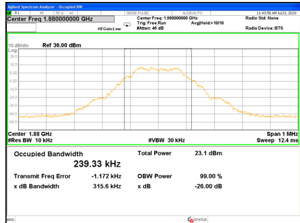
GPRS_1900_Middle_26BW and 99%
